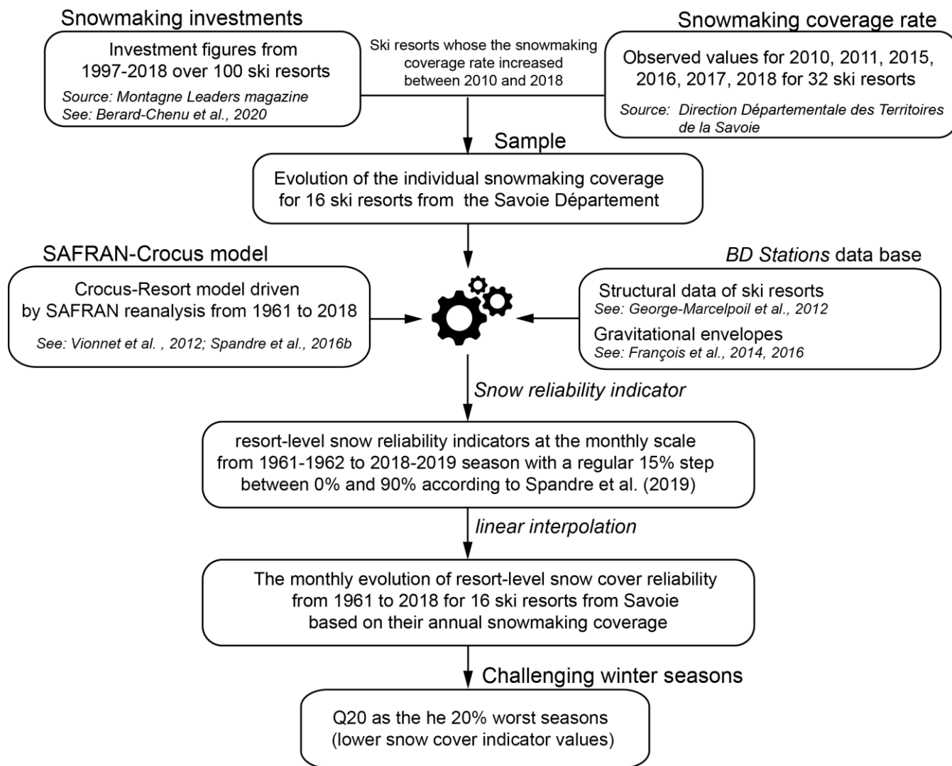
200 Figure 1. Schematic description of the method
