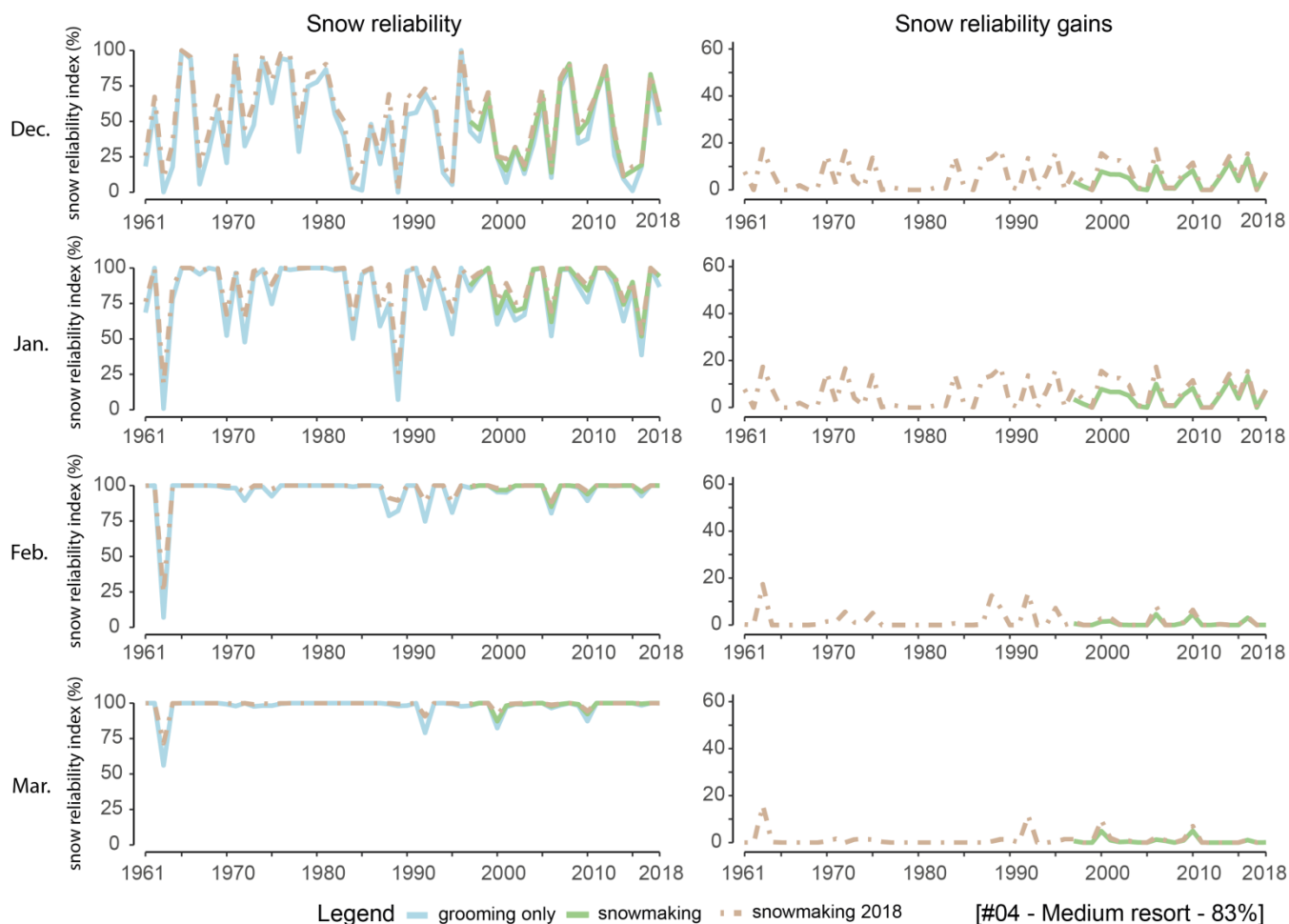
Figure 5. Time evolution of the combined snow reliability indicator and snowmaking fractional coverage for ski resort #04 (medium size, 83% of its surface area below 2000 m elevation) from 1961 to 2018. The left column represents the time variations of the indicator for several snow management options (grooming only, individual evolution of the snowmaking coverage based on investment figures, and the situation corresponding to using the snowmaking coverage in 2018 for the whole time period). The right column represents the increase in snow cover reliability compared to the grooming only situation (taking into account the evolution in snowmaking coverage since 1997 or using the fractional coverage for 2018 throughout the entire record). Each row corresponds to a monthly snow reliability indicator: December to March.
