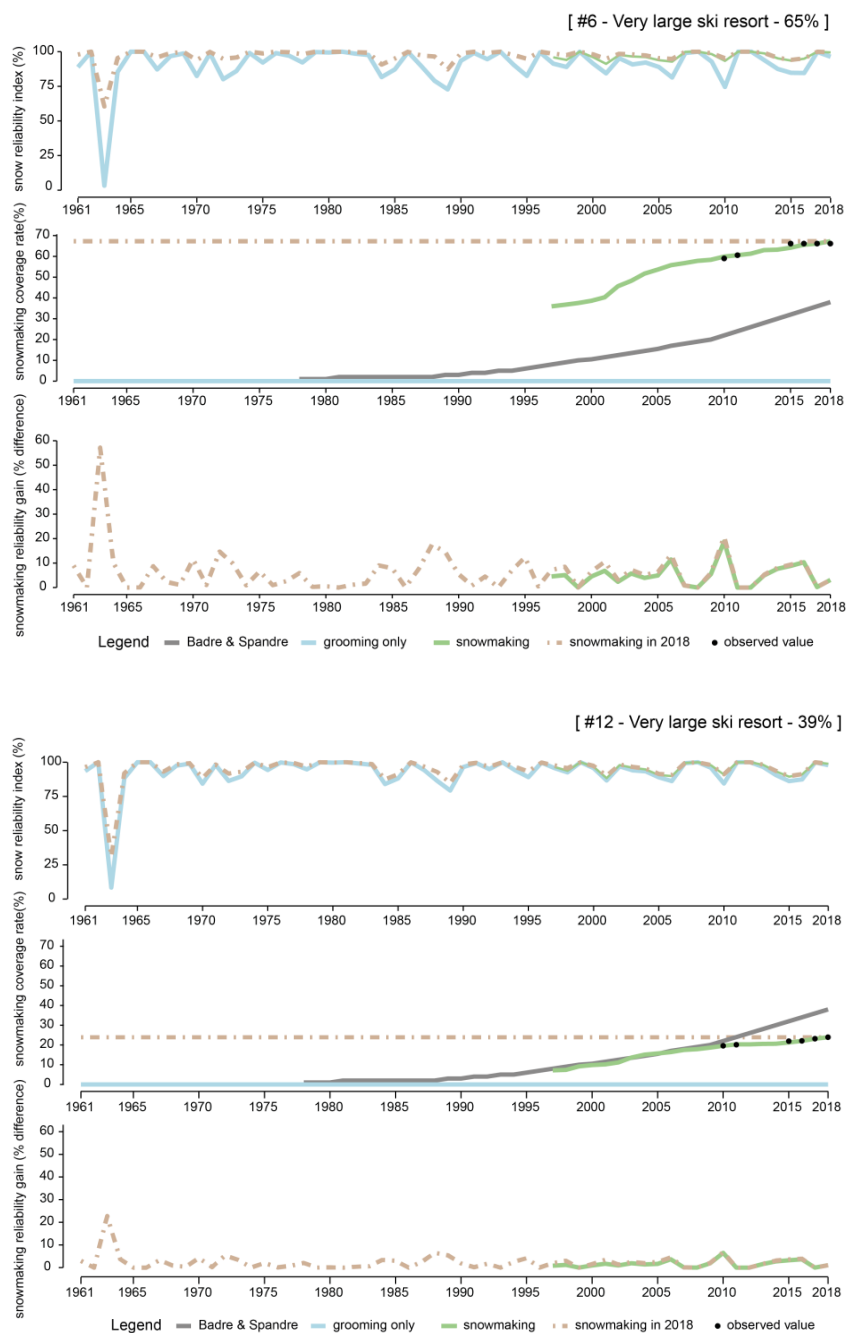
225 Figure 3. Time evolution of the combined snow reliability indicator and snowmaking fractional coverage for two contrasting very large ski resorts (ski resort #6 has 65% of its ski area below 2000m, 39% for ski resort #12) in Savoie from 1961 to 2018. The top row represents the time variations of the indicator for several snow management options (grooming only, snowmaking coverage corresponding to Badré et al.,2009 - mean value for all French ski resorts, individual evolution of the snowmaking coverage based on investment figures, and situation corresponding to using the snowmaking coverage in 2018 for the whole time period). The bottom row indicates the 230 corresponding snowmaking fraction coverage. The last row represents the increase in snow cover reliability compared to the grooming only situation. The ski resort #6 shows a higher-than-average snowmaking equipment, while the ski resort #12 shows a lower-than-average snowmaking equipment.
