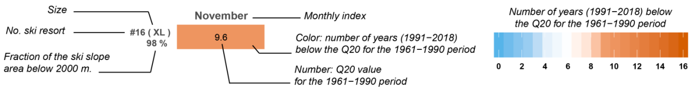
315 Figure 9. Same as Fig.8 but for the snowmaking coverage of 2018 throughout the entire period from 1961 to 2018 (including for the reference time period 1961-1990).
