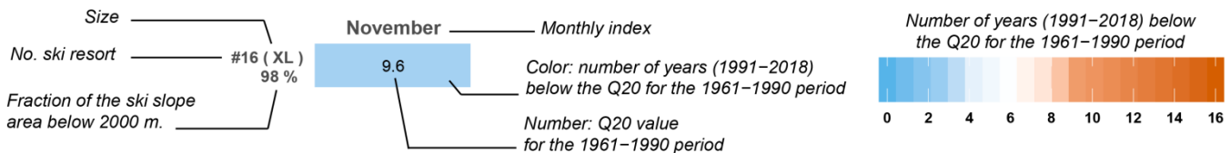
325 Figure 10. Same as Fig. 8 and 9 but with a snowmaking coverage variable in time for each ski resort
