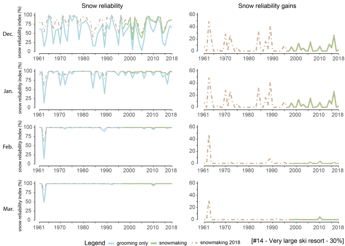
Figure 6. Similar to Fig. 5 but for ski resort #14 (very large ski resorts, 30% of the surface area below 2000 m elevation)
