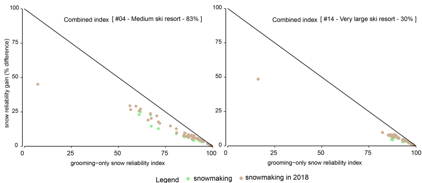
245 Figure 4. Relationship between the combined snow cover reliability difference (y-axis) between configurations with snowmaking and the snow cover reliability with grooming only (no snowmaking, x-axis), for two contrasting ski resorts.
