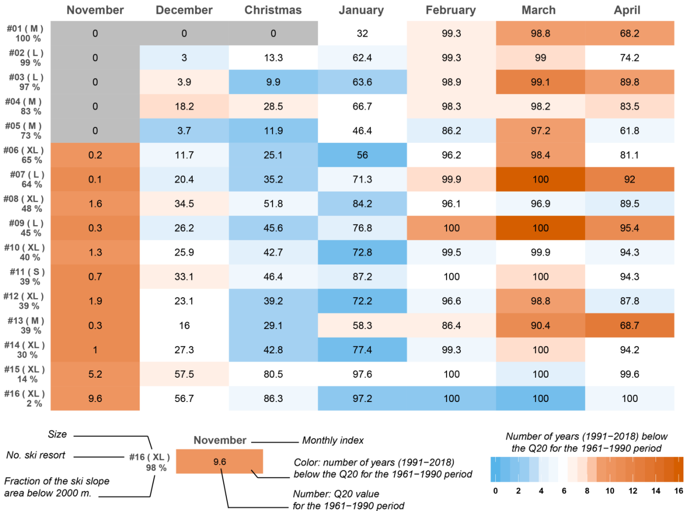
Figure 8. Frequency of occurrence of monthly snow reliability challenging conditions, between 1991 and 2018, below the reference Q20 value for the time period 1961-1990, without snowmaking throughout the entire time period. Each row corresponds to a ski resort (ranked as a function of decreasing fraction of the domain below 2000 m). Each column corresponds to a monthly reliability indicator. The values in the matrix correspond to the Q20 reference snow reliability indicator. Red cells correspond to larger frequencies during 1991-2018 than during the reference time period (more often challenging conditions), and vice versa in blue.
