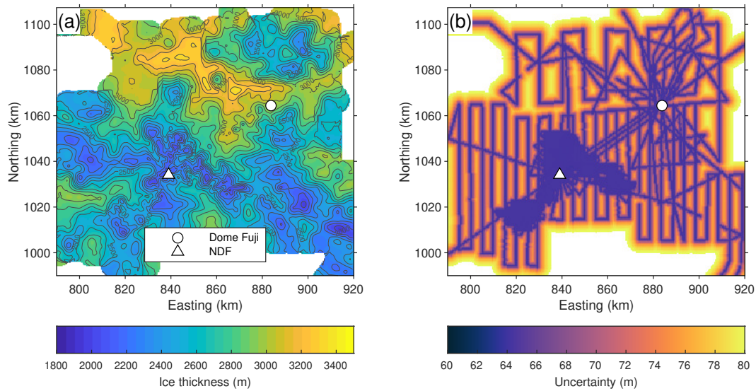
Figure 3. (a) Ice-Gridded ice thickness on the grid (0.5 km horizontal resolution) and the contours with intervals of 100 m. (b) Uncertainty of the gridded ice thickness.
