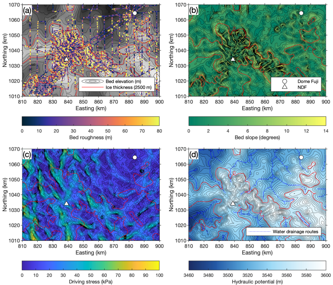
350 Figure 8. (a) Bed roughness superimposed on new bed elevation data (in grayscale) and (b) bed slope. Bed elevation contours in (a) have intervals of 100 m. (c) Driving stress using the new ice thickness data and the Cryosat-2 surface DEM (Helm et al., 2014). (d) Hydraulic potential using the new ice thickness and bed elevation data. The estimated drainage routes of the subglacial water are indicated with blue dots. The red contours in all plots indicate an ice thickness of 2500 m.
