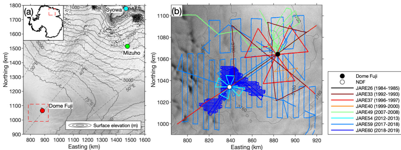
75 Figure 1. (a) The traverse route between Syowa Station and Dome Fuji in Dronning Maud Land, East Antarctica, with the coordinate system of a polar stereographic projection. The box indicates the area shown in (b). The inset shows the location of the region in Antarctica. The contours indicate surface elevation with intervals of 200 m (Helm et al., 2014). (b) Dome Fuji region showing the coverage of the JARE radar survey lines. Surface elevation contours have intervals of 20 m. The background is a RADARSAT-1 L1 image (©CSA, 1997).
