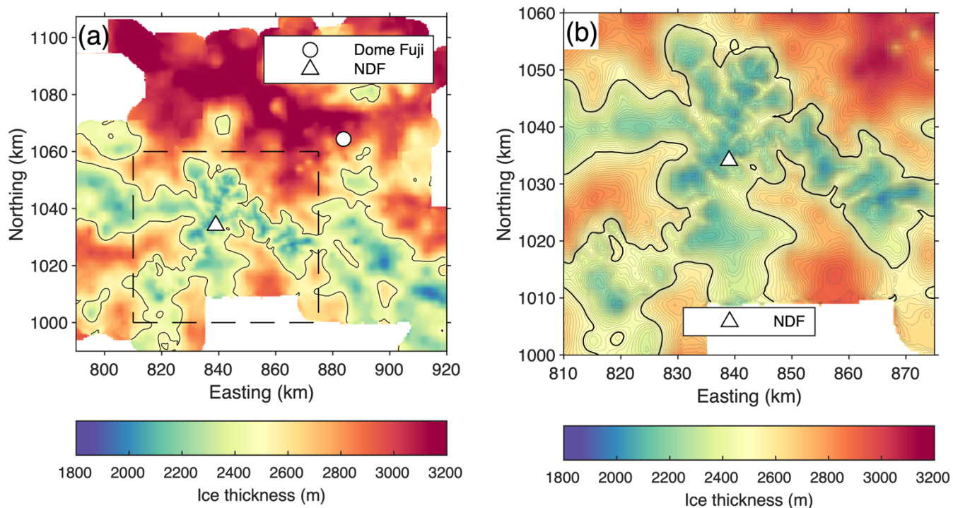
Figure 9. The gridded ice thickness in (a) the study region and (b) the JARE60 observational area. The box in (a) indicates the area shown in (b). The bold contours indicate an ice thickness of 2500 m. The thin contours in (b) indicate ice thickness with intervals of 20 m.
