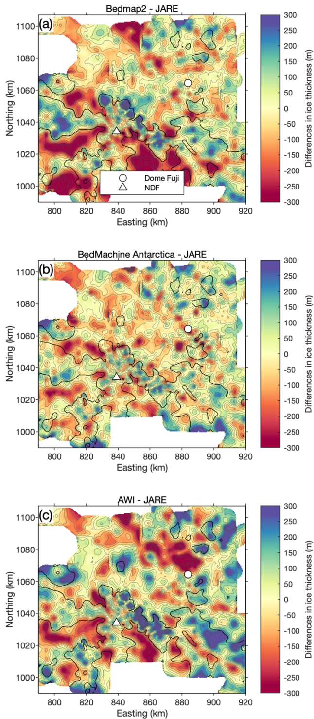
Figure 7. The differences in ice thickness between (a) Bedmap2, (b) BedMachine Antarctica v1, and (c) AWI ice thickness data and the gridded data generated in this study. The bold contours in all plots indicate an ice thickness of 2500 m.
