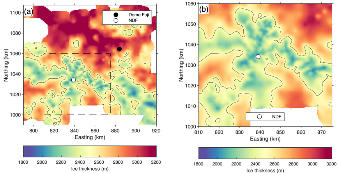
445 Figure 8. The gridded ice thickness in (a) the study region and (b) the JARE60 observational area. The box in (a) indicates the area shown in (b). The contours indicate ice thickness of 2500 m.
