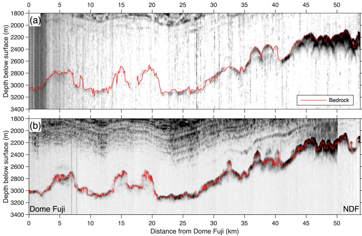
205 Figure 2. Radargrams between Dome Fuji and NDF acquired by the radar systems used in (a) JARE54 (2012–2013) with 3 element Yagi antenna and (b) JARE59 (2017–2018) with 11 element Yagi antenna. The lines indicate bedrock topography traced from the radar data.
