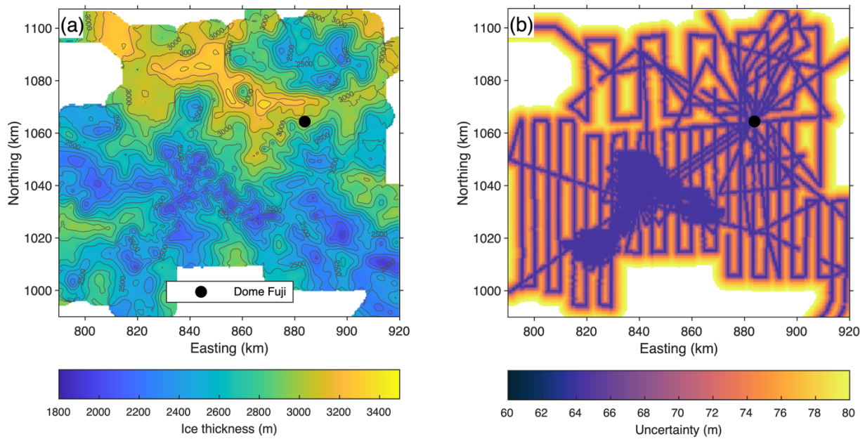
Figure 3. (a) Ice thickness on the grid (500 m horizontal resolution). (b) Uncertainty of the gridded ice thickness.
