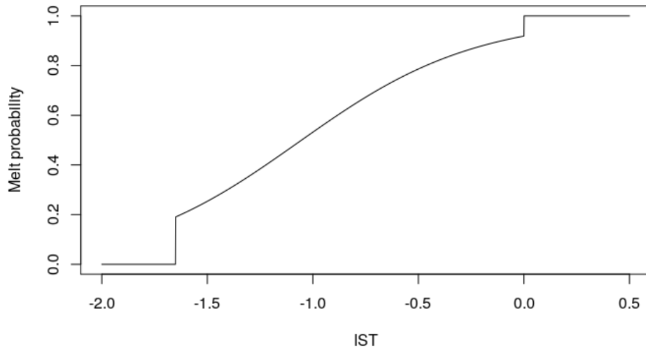
Figure 3. Melt probability estimates of a range of ISTs using the fitted mixture model at a single location-cell (75.37, -58.13) on the Greenland ice sheet between 2001 and 2019. Because some locations-cells have very limited data above -1.65^\circ\text{C} , we use a location-cell on the west coast with a high proportion of data above -1.65^\circ\text{C} (22.55%), thus giving us an increased amount of information in the most pertinent temperature range.
