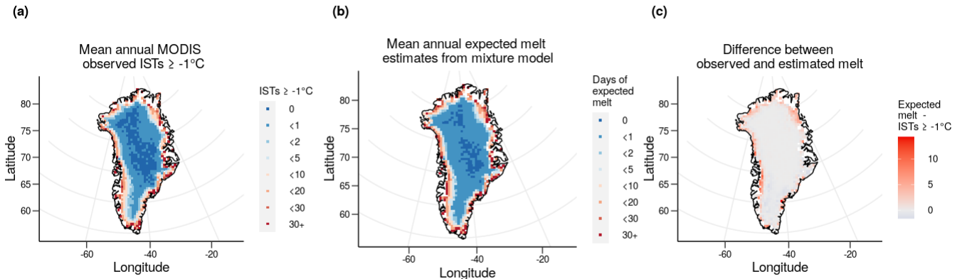
Figure 4. The mean annual number of ISTs above -1^\circ\text{C} per year (a), the mean annual expected melt days estimated from each location cell 's mixture model (b), and the difference between the two variables (c).
