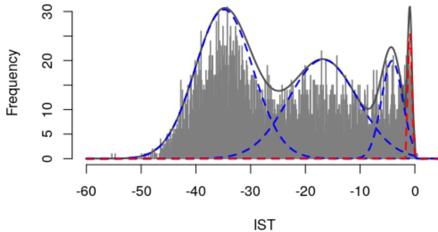
Figure 2. Frequency distribution of daily MODIS IST data from an example location cell (82.47, -37.50) on the Greenland ice sheet between 2001 and 2019. Solid lines show a mixture model fit to these data where black indicates the full model , blue indicates the three 'ice' component and components , red indicates the 'melt' component, and black indicates the full model as the sum of the ice and melt components. Each individual component is a truncated Gaussian distribution, and the lines represent the probability density function of these on a scale to matching that of the histogram.
