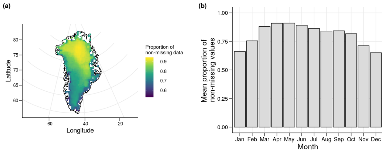
Figure 1. Proportion of non-missing available MODIS IST data (i.e not filtered by the cloud mask) at 1139 locations-cells on the Greenland ice sheet between 2001 and 2019 (a) and mean proportion of non-missing available MODIS IST data by month between 2001 to 2019 (b).
