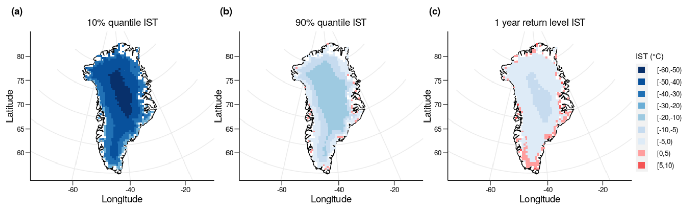
Figure 5. 10% quantile (a), 90% quantile (b), and 1 year return level (c) estimates for MODIS IST data from 2001 to 2019 at 1139 locations-cells . Estimates are calculated from fitted mixture models at each location-cell .
