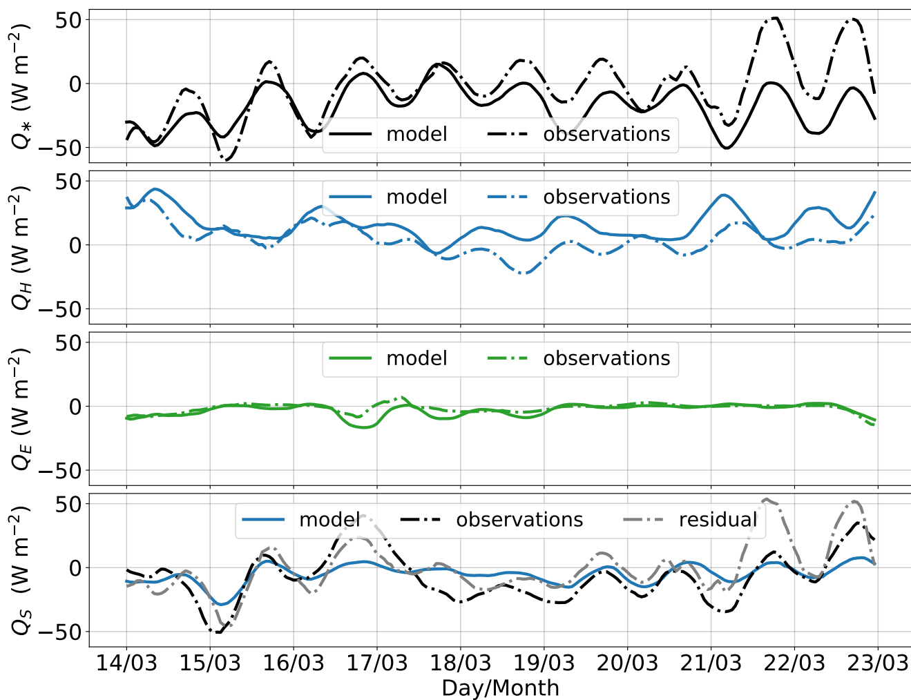
Figure 8. Comparison between observed and modeled hourly means of all constituents of the energy budget at the snow surface from March 14 to 23 2020. The residual snow heat flux is obtained by subtracting the turbulent heat fluxes from the net radiation.
