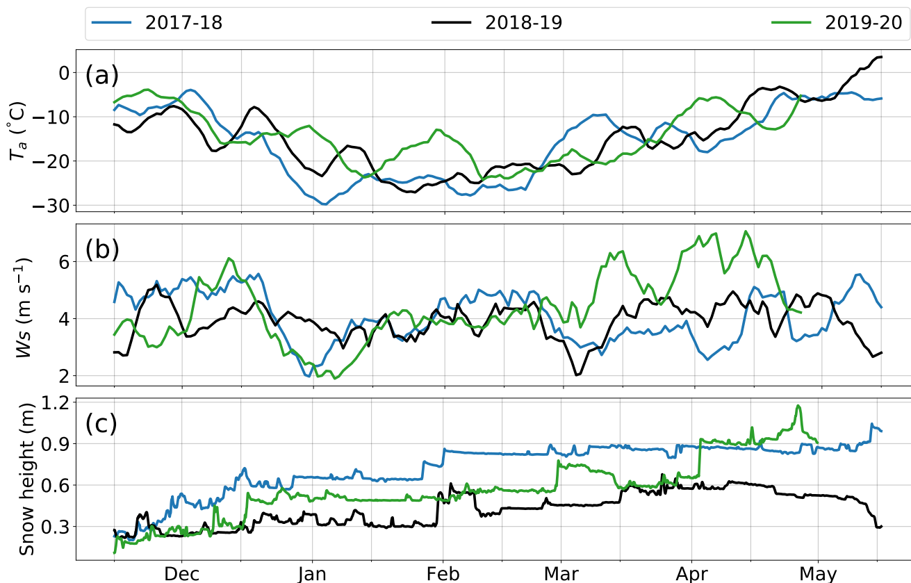
Figure 2. Rolling mean of daily air temperature ( T_a ), wind speed ( W_s ) and snow height for three consecutive winters.
