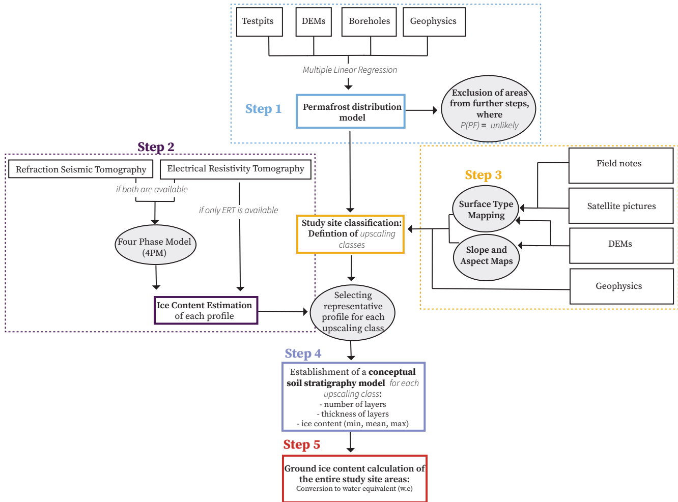
Figure 2. Workflow of the upscaling methodology strategy used in this study. Step 1, we create a simple permafrost distribution model to exclude areas with low permafrost probability from further processing. Then, we use geophysical data, and where applicable, model the ground ice content using the 4PM (Step 2). Then, in Step 3, we define upscaling classes using information from different sources such as aspect and slope maps derived from DEMs, field notes and observations. In Step 4, a conceptual soil stratigraphy model is established using the geophysical results as input for subsurface layers and corresponding ice contents for each upscaling class, which serves as the basis for the upscaling of the ice content to the catchment scale (Step 5).
