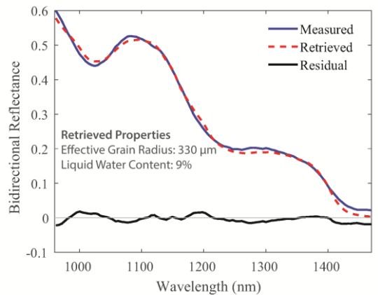
Figure 7: Example of a NIR-HSI measured spectrum, retrieved simulated spectrum using the interstitial sphere model, and the residuals at each band.
