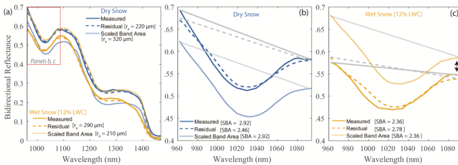
Figure 12: Effective grain radius ( r_e ) retrieval comparison between the residual and scaled band area methods using the interstitial sphere model. (a) An example measured spectra from a dry and wet snow sample and the corresponding retrieved simulated spectra using the residual and scaled band area methods. (b) Dry snow spectra from (a) including the continuum lines, shown in gray, over the absorption feature. (c) Wet snow spectra from (a) including the continuum lines over the absorption feature, shown in gray.
