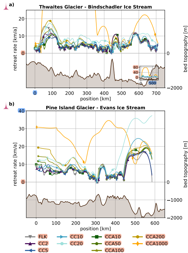
Figure 9. Grounding line retreat rates along the flowlines in Thwaites (a) and Pine Island glacier (b) as a function of grounding line position, together with bed topography. Markers are set every 10 a.
