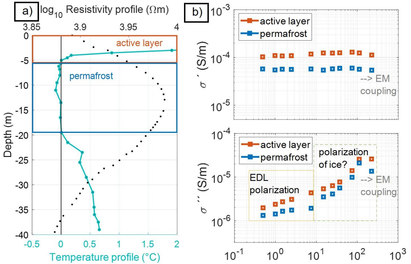
690 Figure 9: (a) Borehole temperature at BH-1108 at the time of the SIP survey with resistivity profile at close proximity to the borehole, and (b) spectral response for a selected depth column at the borehole extracted from the inverted image of profile H2. Pixel values represent the mean value of real and imaginary components and phase of the complex conductivity extracted for two different layers: 0 – 5.6 m depth (thawed active layer) and 5.6 – 19.5 m depth (permafrost).
