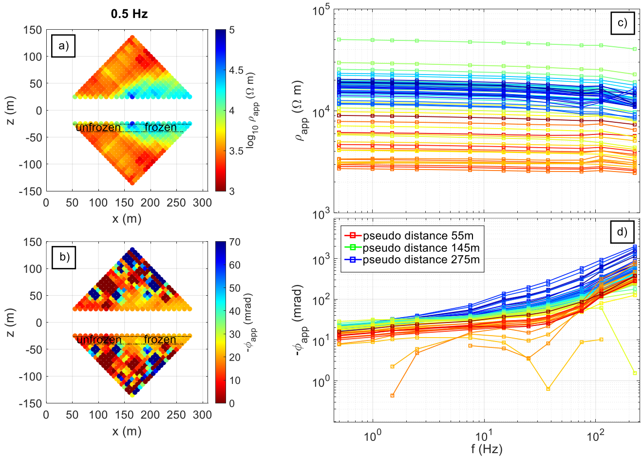
445 Figure 5: Visualization of the frequency-dependence in the electrical impedance measurements collected along profile V2. Impedance magnitude values are converted to apparent resistivity (a) and phase (b) values. The spectral response (c, d) is plotted for level 2 and 3 (i.e. 20 and 30 m electrode separation between current and potential dipoles, between the dashed lines) from north (downslope) to south (upslope) corresponding to the transition from unfrozen to frozen subsurface conditions.
