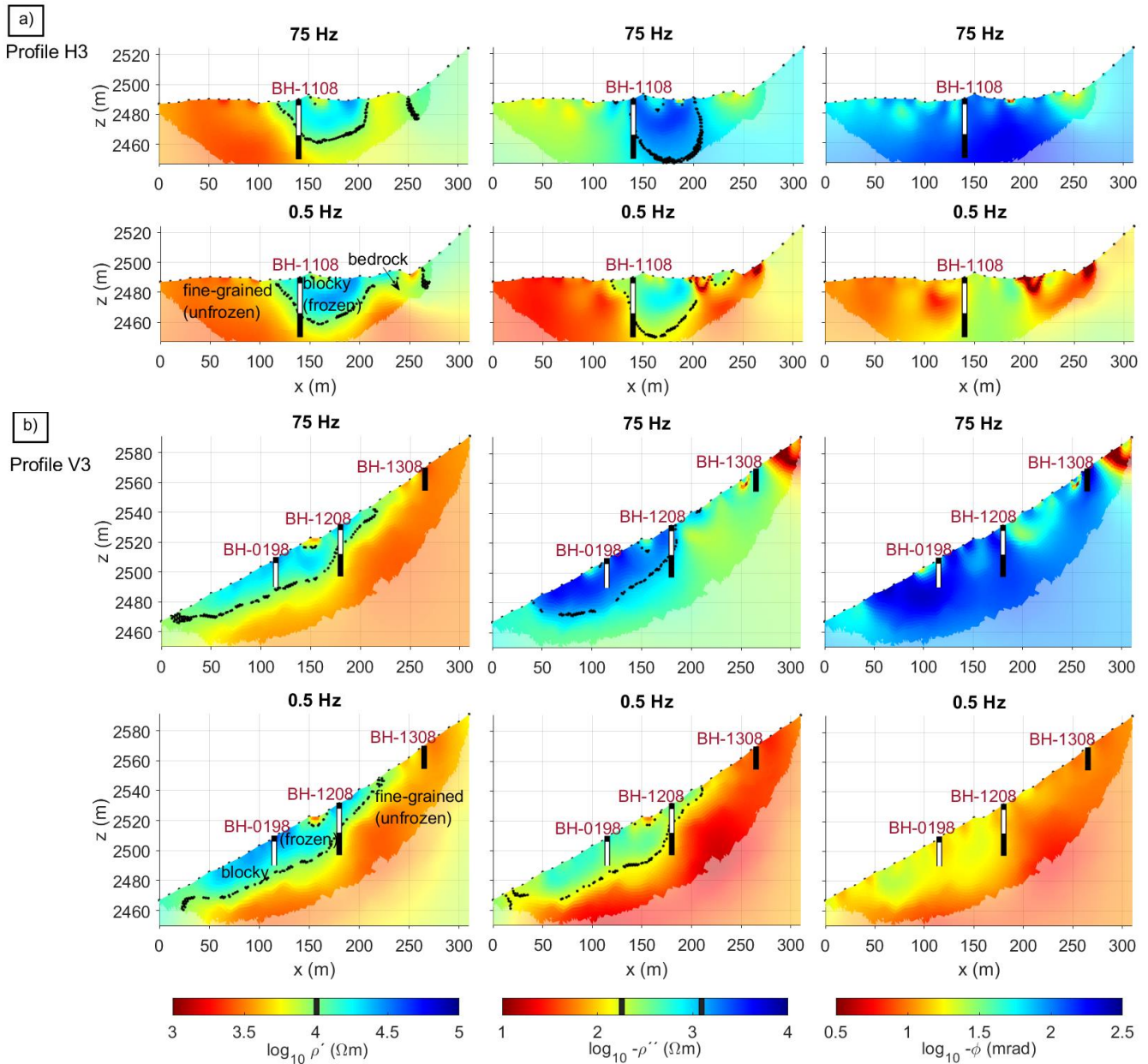
475 Figure 6: Complex resistivity inversion results in terms of real and imaginary components and phase at 75 Hz and 0.5 Hz for profiles a) H3 and b) V3. Our interpretation of frozen and unfrozen parts of the talus slope is indicated by the dashed line, corresponding to values of \rho' = 10,000 \Omega\text{m} , \rho'' = 160 \Omega\text{m} (at 0.5 Hz) and 1,260 \Omega\text{m} (at 75 Hz). The boreholes BH-0198, BH1108, BH-1208 and BH-1308 indicate the thaw depth, permafrost body and permafrost base at the date of the measurement.
