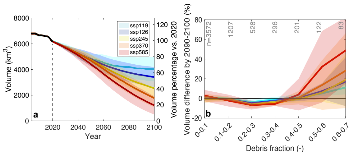
Figure 10. (a) Evolution of the glacier volume for all glaciers in HMA when explicitly modelling debris-cover changes. Results are aggregated to the five SSPs. (b) Difference in volume (mean over 2090-2100) between implicit and explicit debris-cover modelling classified for different debris-cover fractions. The number of modelled glaciers per class is given in grey. The shaded bands represent one standard deviation of all climate model members for a given SSP.
