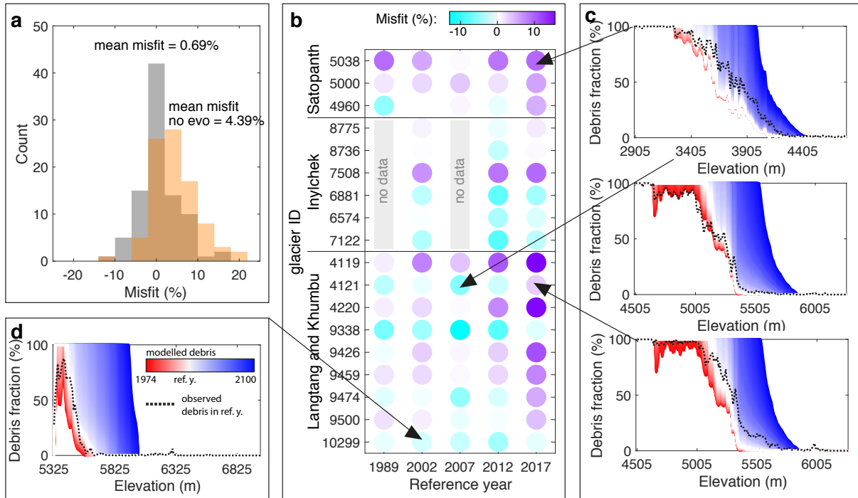
Figure 6. (a) Histograms of the misfit between observed and modelled lateral debris expansion when using c_{lateral} = 2 (grey) and when deactivating the module ( c_{lateral} = 0 , orange). (b) Same as (a) but divided into glaciers and distinguishing between different reference years (corresponding to the Landsat scenes). The colour of each circle represent the misfit (%). (c and d) modelled debris-area evolution (red-white-blue shades) and debris-area evolution as observed in the Landsat scenes (black dashed line) for four selected glaciers (indicated by arrows).
