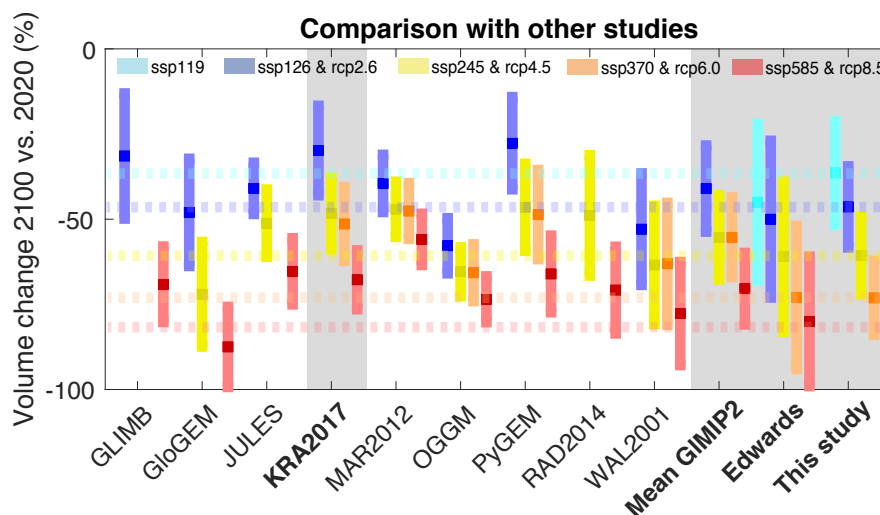
Figure 11. Comparison of modelled volume changes with values from Marzeion et al. (2020) and Edwards et al. (2021). Changes are expressed with respect to the 2020 baseline. From left to right, the abbreviations (GLIMB, GloGEM, JULES, KRA2017, MAR2012, OGGM, PyGEM, RAD2014, WAL2001) stand for Sakai and Fujita (2017); Huss and Hock (2015); Shannon et al. (2019); Kraaijenbrink et al. (2017); Marzeion et al. (2012); Maussion et al. (2019); Rounce et al. (2020); Radić and Hock (2014); Van de Wal and Wild (2001).
