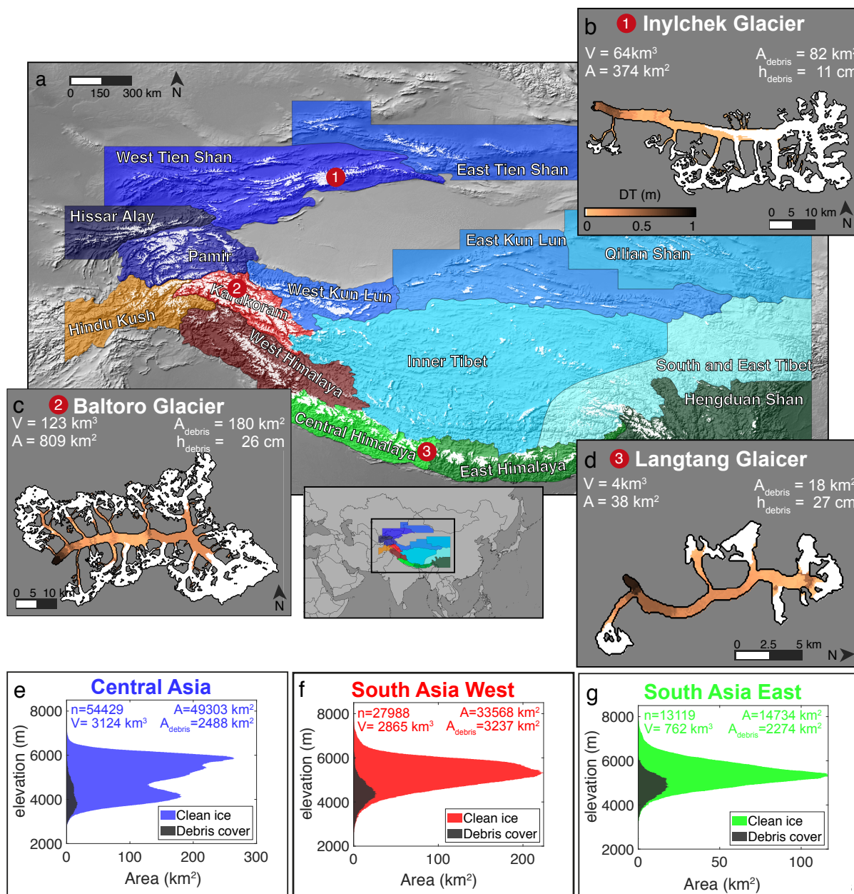
Figure 1. (a) Extent of HMA glaciers (white) as per Randolph Glacier Inventory version 6 (RGI Consortium, 2017). The three main RGI regions (Central-Asia, South-Asia-West, and South-Asia-East) are shown by blueish, reddish, and greenish colours, respectively. RGI second-order regions are labelled individually. Three glaciers are highlighted to illustrate glacier-specific model results (red spheres with numbers). (b & c & d) Map of the three highlighted glaciers with their mean 2000–2016 debris thickness given by colours (scale in panel b). Glacier outlines and debris thickness are from RGI Consortium (2017) and McCarthy et al. (sub.), respectively. For each glacier, V is the glacier ice volume according to Farinotti et al. (2019a), A is the glacier area according to RGI 6.0, A_{\text{debris}} is the debris-covered area, and h_{\text{debris}} is the mean debris-cover thickness according to McCarthy et al. (sub.). (e & f & g) Glacier hypsometry (area per 10 meter elevation band) and debris-covered area distribution at inventory date. n is the number of glaciers within each region (RGI Consortium, 2017) Map source: Natural Earth.
