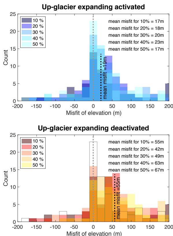
Figure 7. Misfit between observed and modelled highest elevation with a lateral debris expansion \geq 10, 20, 30, 40 and 50\% . The debris area evolution module is activated in panel a and deactivated in panel b .
