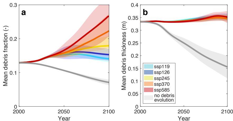
Figure 9. Evolution of (a) debris-covered fraction and (b) debris thickness for all HMA glaciers and as an average for the respective SSP. The shaded bands represent one standard deviation of all climate model members. The grey line indicates the case in which the debris-evolution module is disabled and only today's debris cover is used in the modelling.
