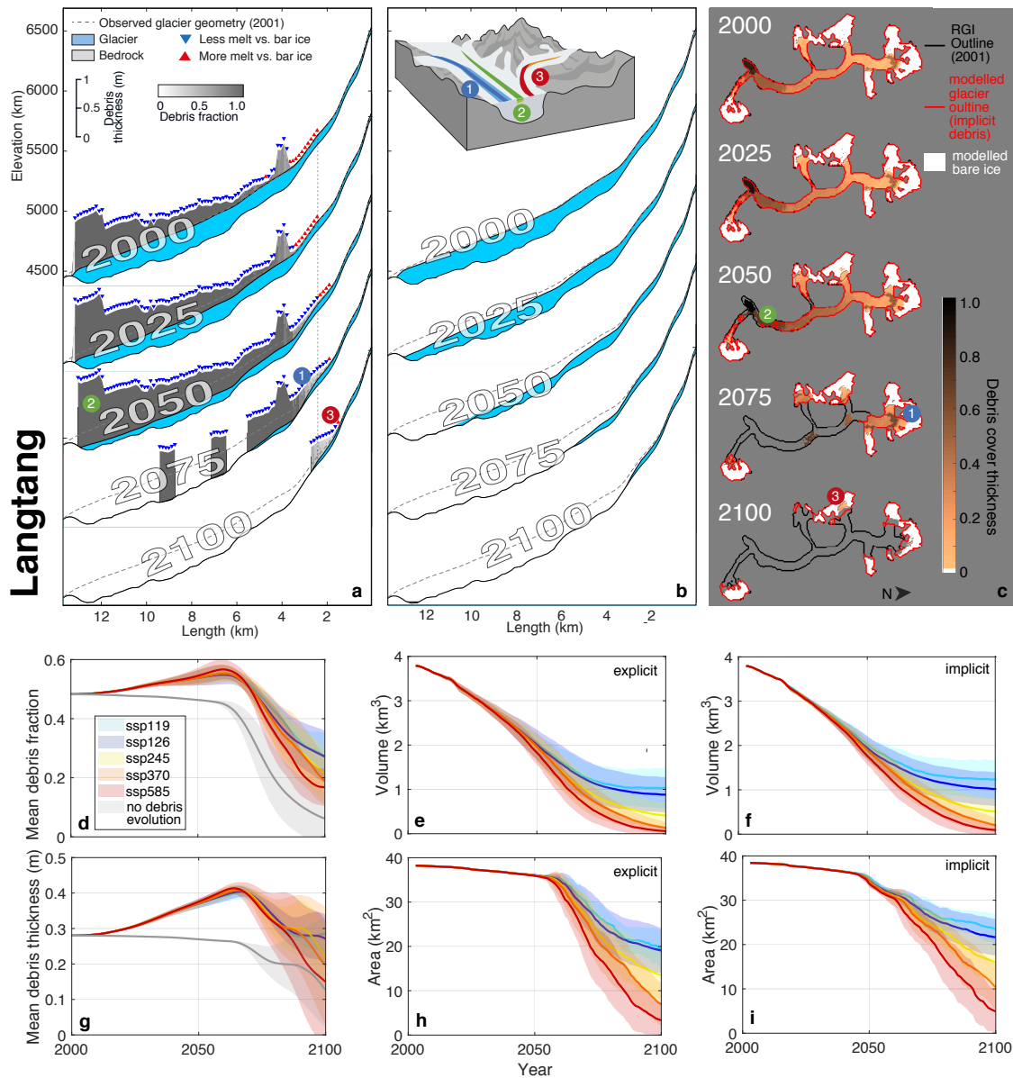
Figure 8. (a) Modelled evolution of Langtang Glacier when debris is explicitly accounted for. The results refer to SSP245. Note that the debris thickness (grey) is exaggerated by a factor of 500 for visibility. The three parametrizations included in the debris-cover module (cf. section 3.2 and Figure 3) are indicated by the circled, colored numbers, and described in the text. (b) Same as (a), but accounting for debris implicitly, i.e. glacier evolution is not modelled with the new debris module, but by re-calibrating some of the model parameters to match observed long-term mass balance (see section 4.1 for details). (c) Model results extrapolated to 2D (see Supplementary Material for the extrapolation method). For every SSP, the evolution of (d) debris-cover fraction, (e/f) glacier volume with explicit/implicit debris-cover modelling, (g) debris thickness, and (h/i) glacier area with explicit/implicit modelling is shown. The shaded ranges represent one standard deviation of all climate model members included in a given SSP.
