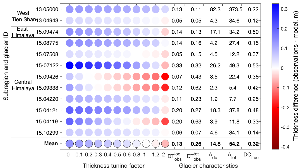
Figure 5. Difference between observed and modelled debris thickness for the period \approx 1981 –2008 (circles). The numbers in the right-hand part of the figure are glacier specific. DT_{obs}^{loc} is the observed mean debris thickness (m) for locations in which the debris was formed between \approx 1974 and \approx 1989 ; DT_{obs}^{tot} is the mean debris thickness (m) of the debris-covered part at inventory date; A_{dc} is the debris-covered area ( \text{km}^2 ); A_{tot} is the area of the whole glacier ( \text{km}^2 ); and DC_{frac} = A_{dc} / A_{tot} (%).
