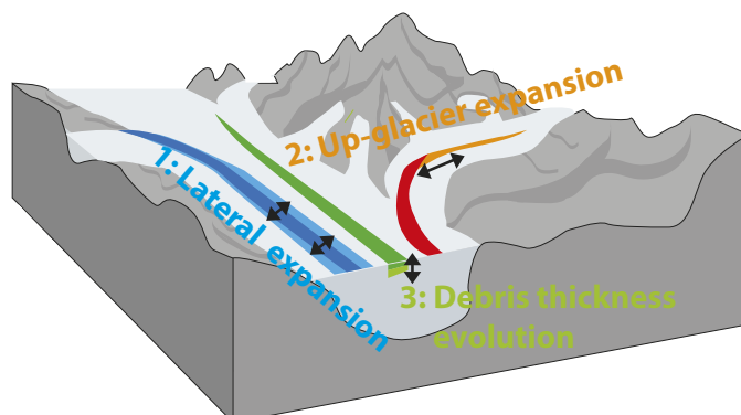
Figure 3. Sketch showing the three main processes (parametrizations) captured by the debris-cover extent and thickness evolution module.
