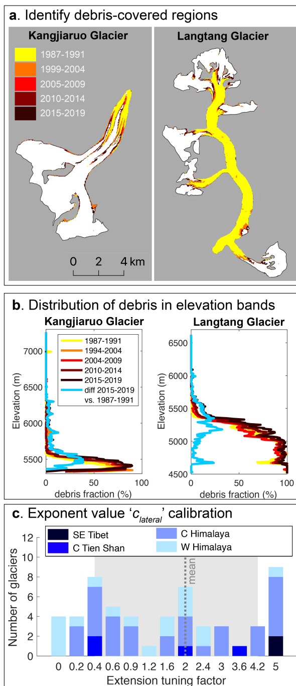
Figure 4. (a) Evolution of the debris-covered area of Kangjiaruo Glacier and Langtang Glacier as inferred from five Landsat scenes. (b) Same as (a), but divided into 10-meter elevation bands. The blue line shows the lateral expansion of the debris cover as observed between the oldest (1987-1991) and the newest (2015-2019) Landsat scene. (c) Distribution of c_{lateral} resulting in lowest misfit between observed and modelled debris fraction evolution (given per number of glaciers). The grey dashed line shows the mean value while the grey rectangle shows values within the 0.25 and 0.75 quartiles.
