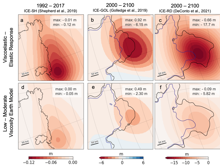
Figure 6. Influence of incorporating viscous behaviour and uncertainty in viscoelastic Earth structure on sea level predictions. Frames (a-c) shows the difference in sea level change predicted from simulations adopting 3-D viscoelastic earth model EM1_L and an elastic Earth model. Frames (d-f) shows the difference in sea level change predicted from simulations adopting two different 3-D viscoelastic earth models EM1_L and EM1_M. Note the difference in scale. Time frames and ice models are as indicated at the top of the columns. In each frame, the black and blue line indicates final and initial grounding lines respectively for each simulation and is annotated with the maximum and minimum data value within the frame. All simulations adopt a 1.9 km grid resolution.
