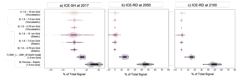
Figure 9. Comparison of factors contributing to differences in sea-level predictions in this study. Each distribution represents the influence of the specific factor across points within 10-km of the grounding line at the specified year of the model run, as a percentage of the total sea-level change at that time for a) ICE-SH ice model from 1992 to 2017; b) ICE-RD ice model from 1950 to 2050; c) ICE-RD ice model from 1950 to 2100. Six factors are compared in this figure, as labelled on the right. To visualise the distribution, we plot a classic box-whisker diagram overlain with a density curve. The edges of the box represents (from left to right) the 25 th percentile, median and 75 th percentile of the distribution, whilst the whiskers represent the “minimum” (25 th percentile – 1.5 x the interquartile range) and “maximum” (75 th percentile + 1.5 x the interquartile range). The diamonds outside the whiskers represent outliers.
