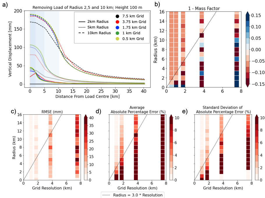
835 Figure 3. Idealized sensitivity experiment of the effect of surface grid resolution on GIA model calculations with elastic bedrock deformation due to instantaneous removal of cylindrical ice loads. Cylinders are all of unit height 100 m, and radius from 0.5 to 16 km. Five grid resolutions applied within an area of minimum 40km width were tested: 0.5, 1, 1.75 km, 3.75 and 7.5 km (Figure S1). 840 (a) Transect of bedrock deformation for removal of ice cylinders with unit height and radii of 2 km (solid lines), 5 km (dotted) and 10 km (dashed lines). (b) – (e) Results of a suite of simulations adopting ranges of ice cylinder radii and grid resolutions. (b) Colors indicate 1 minus the Sealing-Mass Factor, [ 1 – Sealing-Mass Factor ], where the Sealing-Mass Factor is the ratio of the theoretical mass of the load and the mass of the load represented on the given model grid. 0 represents a scenario where the model grid perfectly represents the mass of the idealized load, whilst positive (blue) and negative (red) values indicate the load mass is over- and under- 845 represented by model grid resolution, respectively. (c) Root mean square error across the suite of simulations (mm). (d) Average absolute percentage error (%). (e) Standard deviation of the absolute percentage error (%) of the given test from the finest 0.5 km resolution model result, calculated within 2 km of the loaded region. Dashed black lines represent the 1:3 ratio between idealized load cylinder radius and surface grid resolution whereby average absolute percentage error becomes < 7 \pm 3 (\sigma) \% for all scenarios.
