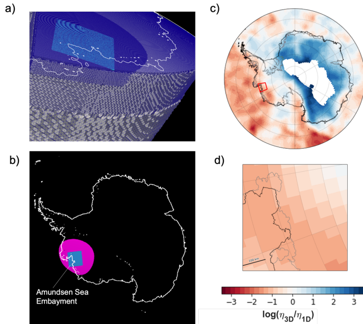
815 Figure 1. Grid and Earth model configuration. (a-b) Configuration of the tetrahedral grid in the finite-volume 3-D GIA model with regional refinement, used for observational and modelled ice loading scenarios. (a) shows a cross-sectional view of the regional refinement along ASE. (b) indicates areas of grid refinement across Antarctica with a surface grid resolution of 7.5 km over all Antarctica in black, 3.75 km over a section of the West Antarctica in magenta and 1.9 km in the ASE (light blue square). (c-d) Logarithmic viscosity perturbation map at depth 200 km for low upper mantle viscosity model EM1_L over (c) Antarctica and (d) our study region in the Amundsen Sea Embayment. Values are relative to reference 1-D model with upper mantle viscosity of 1 \times 10^{20} Pa s, and lower mantle viscosity of 5 \times 10^{21} Pa s. The black line delimits the Antarctic grounding line, and the graydark green line shows the bedrock topography contour at 0 m from Bedmap2 (Fretwell et al., 2013) highlighting marine-based sectors of ice. Transparent patch in (c) contains no data on mantle viscosity as it the region contains lithosphere at 200 km depth.
