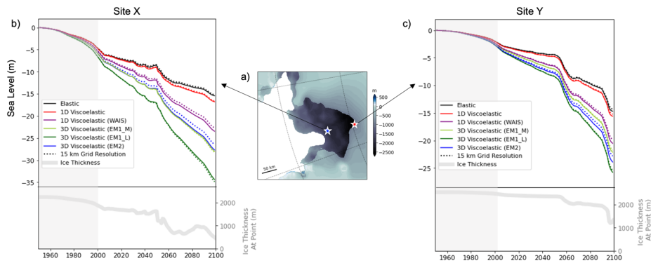
875 Figure 8. Evolution of site-specific sea level in simulations adopting a range of model resolutions and Earth models. (a) ice thickness change from 2000 to 2100 predicted in the ICE-RD simulation. This frame is identical to figure 23c. (b) colored lines show predicted sea level change, in meters, at the Site X that experiences the maximum viscous uplift in the 1.9 km resolution simulation, shown by the blue star in frame (a) in the simulations with a purely elastic solid earth response (black lines), viscoelastic solid earth response based on a global average 1-D earth model (red lines), a 1-D earth model best-fit for the WAIS from Powell et al. (in review) (purple lines), a low viscosity 3-D earth model EM1_L (dark green lines), a moderate viscosity 3-D earth model EM1_M (light green lines) and 3-D viscosity earth model EM2 (blue lines). Solid lines are for simulations performed at 1.9 km resolution, and dashed lines adopt a 15km resolution. (c) is as in frame (b) but for the Site Y along the final grounding line position at 2100 that experiences the greatest ice thickness change, labeled by the red star in frame (a). 880
