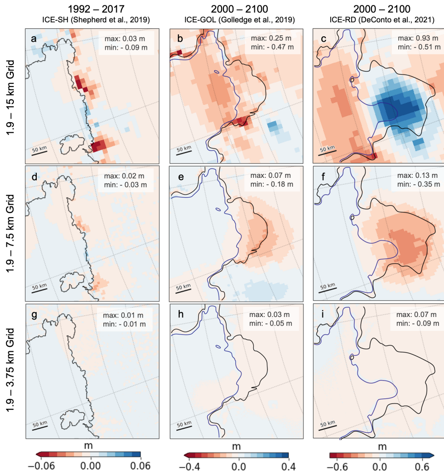
870 Figure 7. Influence of grid resolution on viscoelastic sea level predictions in ASE. As in Figure 4 but adopting 3-D viscoelastic Earth model EMI_L.
