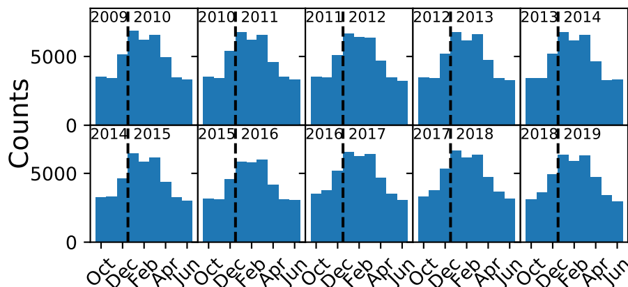
Figure 3. Monthly observation count for each winter year over the whole domain.
