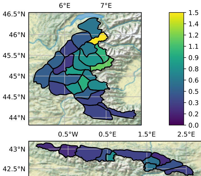
Figure 1. Average daily observation density (per 100 km 2 ) within each SAFRAN massif, in the French Alps (top panel) and French Pyrenees/Andorra (bottom panel).
