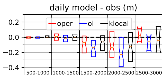
Figure 7. Notched boxplots of the daily difference between modelled and observed values (over the 10 years) of the oper (red), open-loop (blue) and klocal:35km (black), by 500 m-wide elevation bands. Occurrences when the three differences are equal to zero are excluded.
