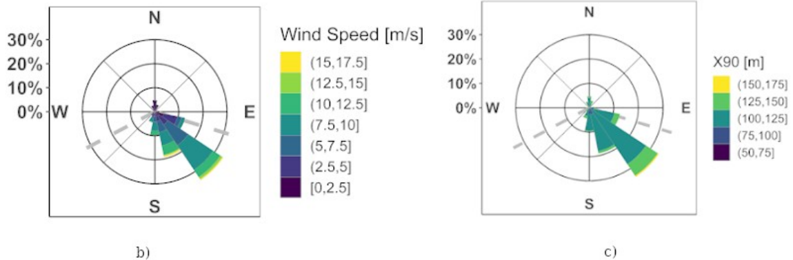
Figure 3: The experiment on the coast of Lake Zub/Priyadarshini: (a) Irgason installed on the lake shore (06.01.2018); (b) wind speed and direction measured at the Irgason site, dashed line indicates the footprint wind sector; (c) the footprint length estimate (X90).
