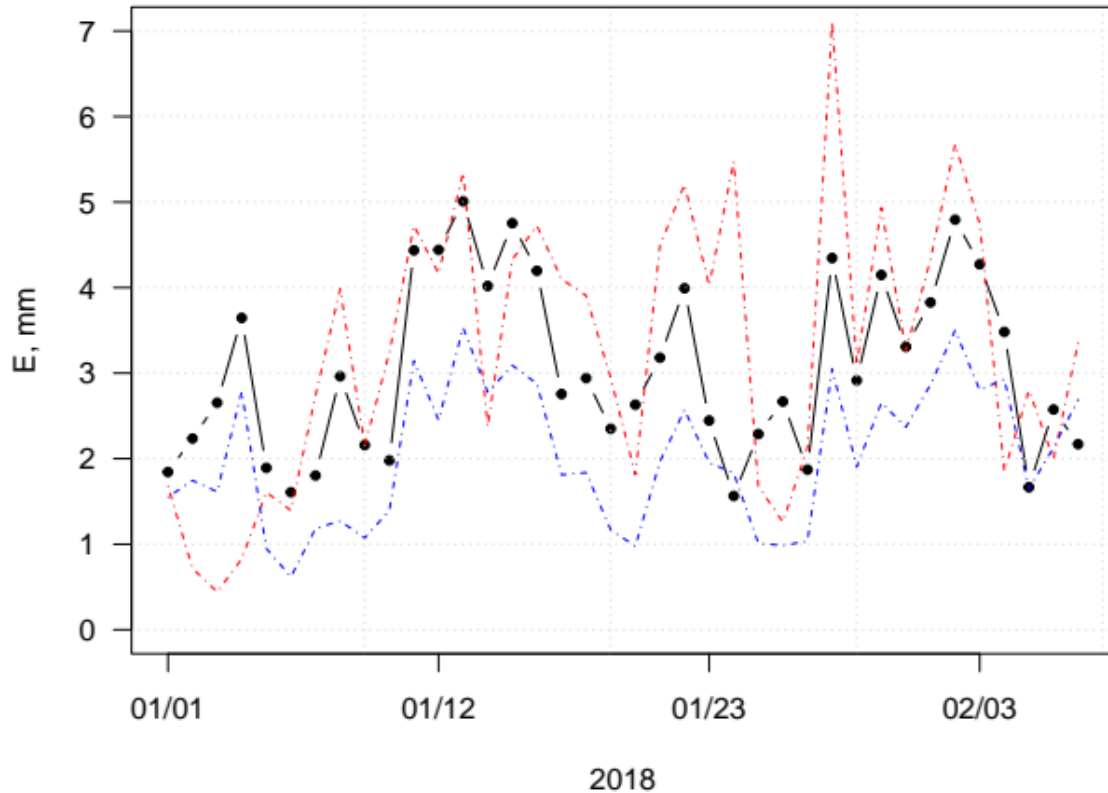
Figure 7. The daily time series of evaporation ( \text{mm day}^{-1} ) calculated by the EC method (black), by the bulk-aerodynamic method (blue) and by new combination equation (red) applying the meteorological measurements at the Maitri site.
