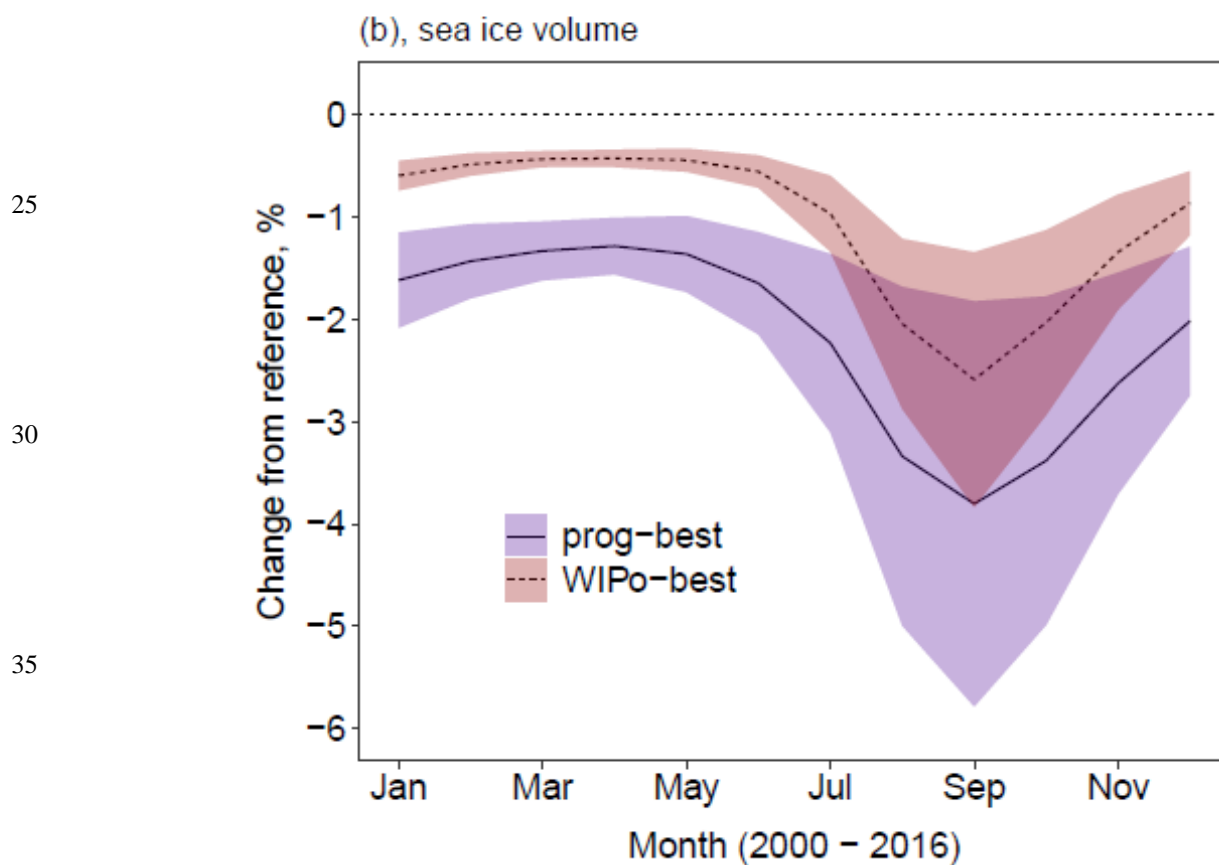
Figure 7: Difference in sea ice extent (top) and volume (bottom) of prog-best (solid, blue shading) and WIPo-best (dashed, red shading) relative to ref averaged over 2000 - 2016. The shading shows, in each case, plus or minus two times the standard deviation around the mean.
