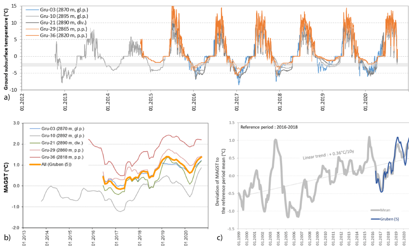
190 Figure 3: Daily ground surface temperature on the Gruben rockglacier rock glacier (gl.p.: glacier-affected part; p.p.: periglacial part; div.: transition zone) since 2013, with indication of the upper limit of BTS for permafrost conditions ( horizontal light-grey bar ) (a), mean annual ground surface temperature (MAGST) (b), and deviation to the reference period 2016 - 2018 in comparison with to the overall signal measured on rockglacier rock glaciers and debris landforms (n= 2 to >20) in the surrounding region (c) (data: PERMOS and University of Fribourg FR).
