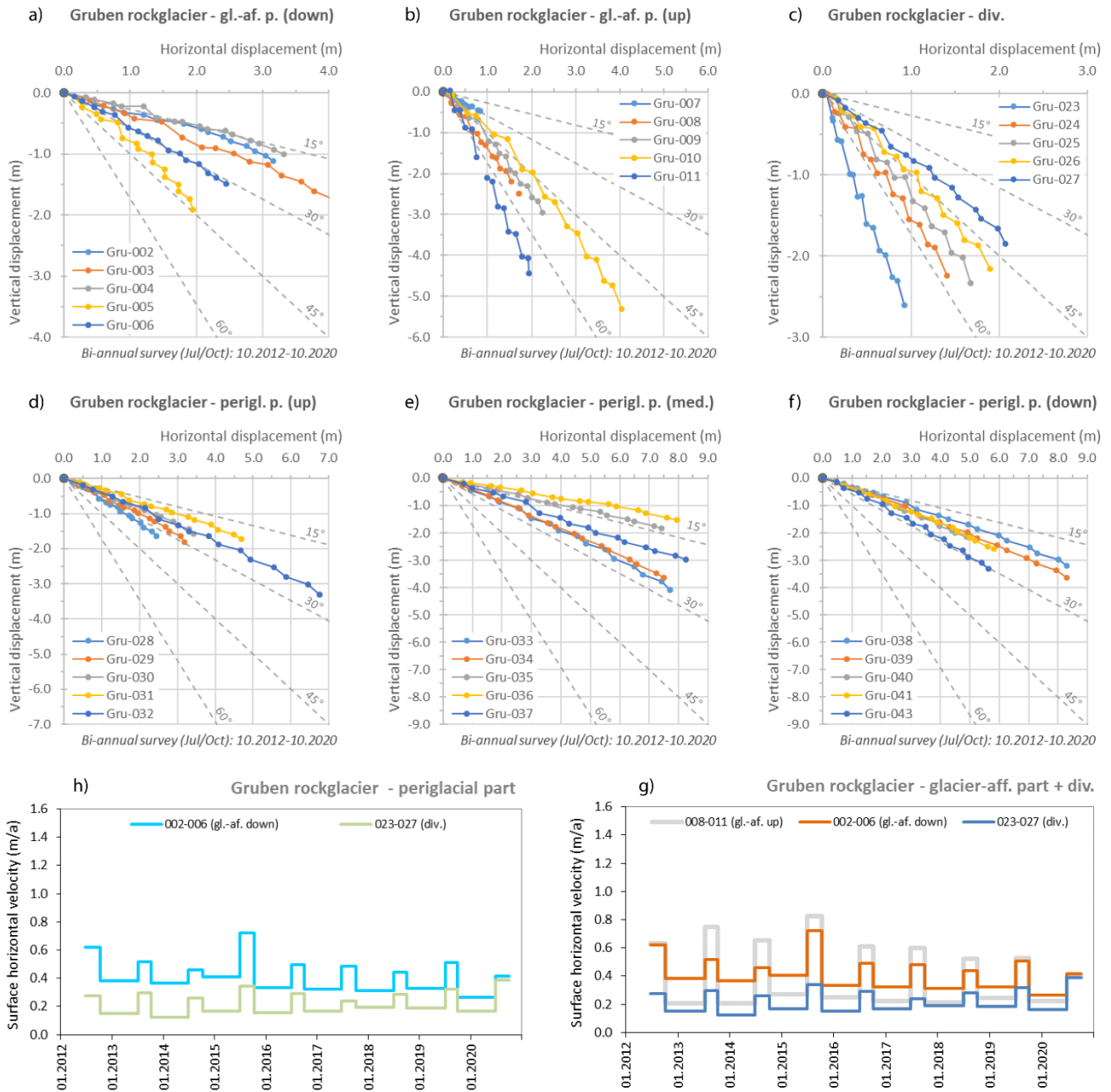
Figure 7: GNSS-based rockglacier kinematic behaviour in both glacier-affected (gl.-af.) and periglacial (perigl.) parts of the Gruben rockglacier rock glacier as well as in their transition zone (div.). a) -f): Horizontal versus vertical displacement of selected items. g) -h): Seasonal horizontal velocities in specific sections. The numbers or identifiers are referring to the GNSS-surveyed items; location in Fig. 6.
