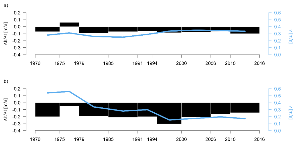
Figure 8: Mean vertical changes (black columns) and horizontal velocities (blue line) of the periglacial part of the rockglacier (a) and the glacier-affected part of the rockglacier (b) from 1970 to 2016. The values of the period 1970 to 1995 result from Kääb et al., 1997.
