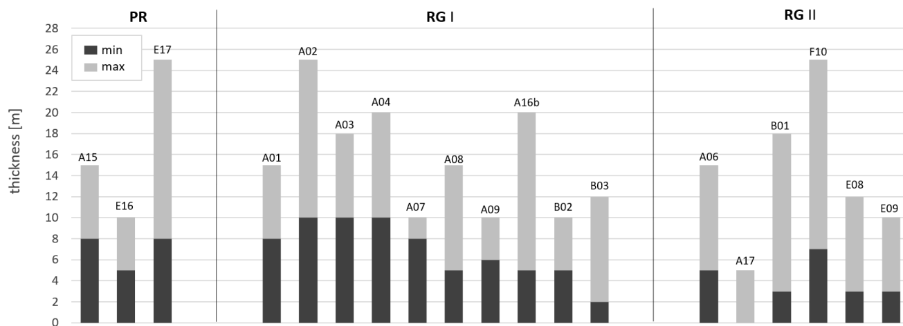
220 Figure 4: Overview over minimum and maximum thickness of ice-rich permafrost in all protalus ramparts (PR), and rock glaciers (RG) of group I and II, determined from the high-resistive zone in the ERT tomograms. Profile A17 is from a relict rock glacier with little probability for ground ice.
