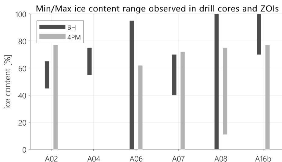
470 Figure 12: Comparison of borehole-derived with 4PM-derived min/max ice contents within the pre-defined ZOIs. Here, only borehole values for the depth range covered by the ZOIs are considered.
