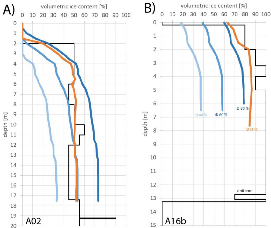
475 Figure 13: Comparison of ground truthing information from a drill core (black line) with 4PM-derived ground ice volumes at the borehole position of profiles A02 (A) and A16b (B). The blue lines correspond to 4PM runs based on homogeneous porosity models with 40, 60, and 80 % (as used for the ZOIs), and the orange line shows the 4PM result after calibration with ground truthing data.
