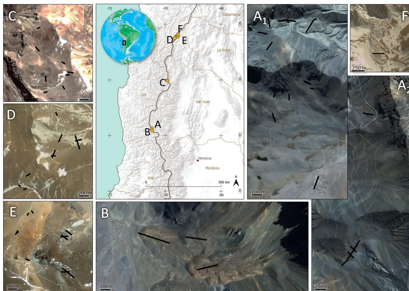
Figure 1: Map of the Central Andes with the study sites A - F, and detailed images for each of the study sites, showing the geophysical lines completed (Map data: © Google Earth 2021).
