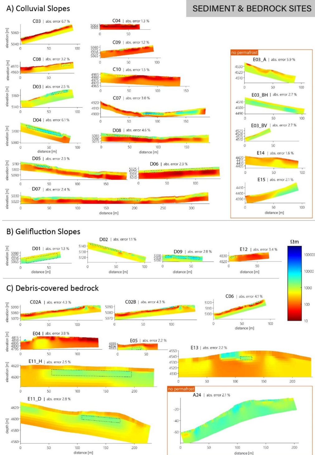
Figure A2: inverted tomograms of all ERT profiles from sediment and bedrock sites (same spatial and colour scales), sorted by landforms
