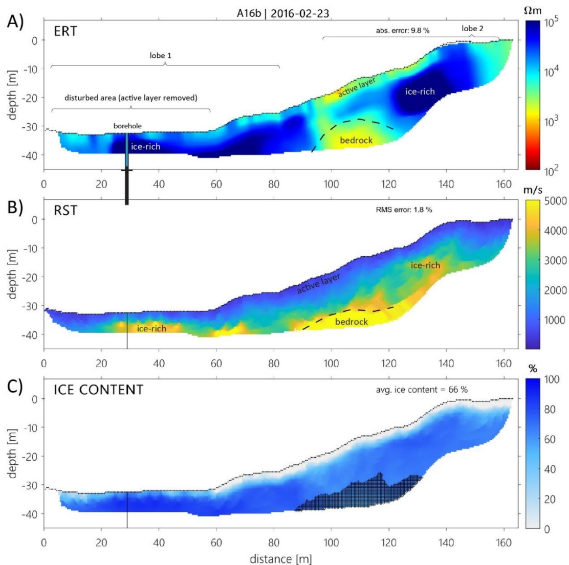
250 Figure 5: Geophysical results of A16B (rock glacier): a) section of the ERT profile covered by the RST profile (see Figure 3a for full profile), b) RST profile, and c) volumetric ice content modelled by the 4PM. The borehole position is indicated, with the light blue part indicating the frozen part. The data misfit of both inversion models is indicated in the upper right corner. The cross-hatched zone marks the area detected as bedrock in the 4PM. Labels denote the interpretation.
