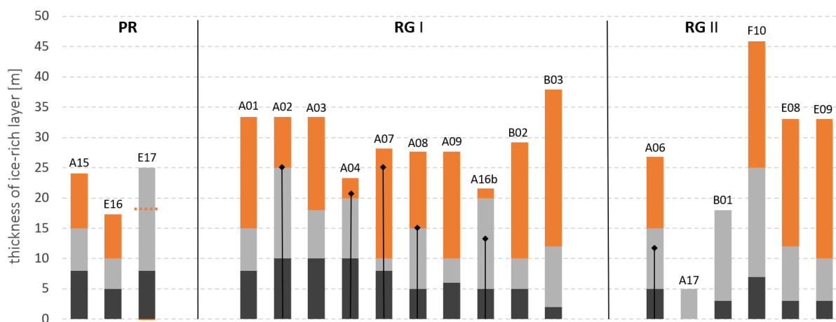
510 Figure 14: Comparison of the minimum/maximum (black/grey) thickness of the ice-rich layer of rock glaciers (as in Figure 4) with the estimated rock glacier thickness according to the area-thickness relation after Brenning 2005 (orange) for selected rock glaciers and protalus ramparts. Brenning's approach has not been applied to A17 and B01, which are strongly degraded or relict rock glaciers. For E17, the area-thickness relation revealed a slightly smaller thickness (dashed orange line) than the geophysical maximum value. Black vertical lines illustrate the permafrost thickness revealed from borehole evidence, where available.
