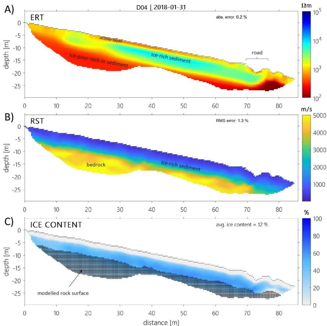
Figure 9: Geophysical results of D04 (colluvial sediments): a) section of the ERT profile covered by the RST profile (see A2a for full profile), b) RST profile, and c) volumetric ice content modelled by the 4PM. The data misfit of both inversion models is indicated in the upper right corner. The cross-hatched zone marks the area detected as bedrock in the 4PM. Labels denote the interpretation.
