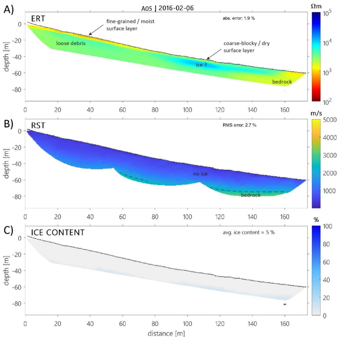
290 Figure 8: Geophysical results of A05 (talus slope): a) section of the ERT profile covered by the RST profile (see Figure 7 for full profile), b) RST profile, and c) volumetric ice content modelled by the 4PM. The data misfit of both inversion models is indicated in the upper right corner. Labels denote the interpretation.
