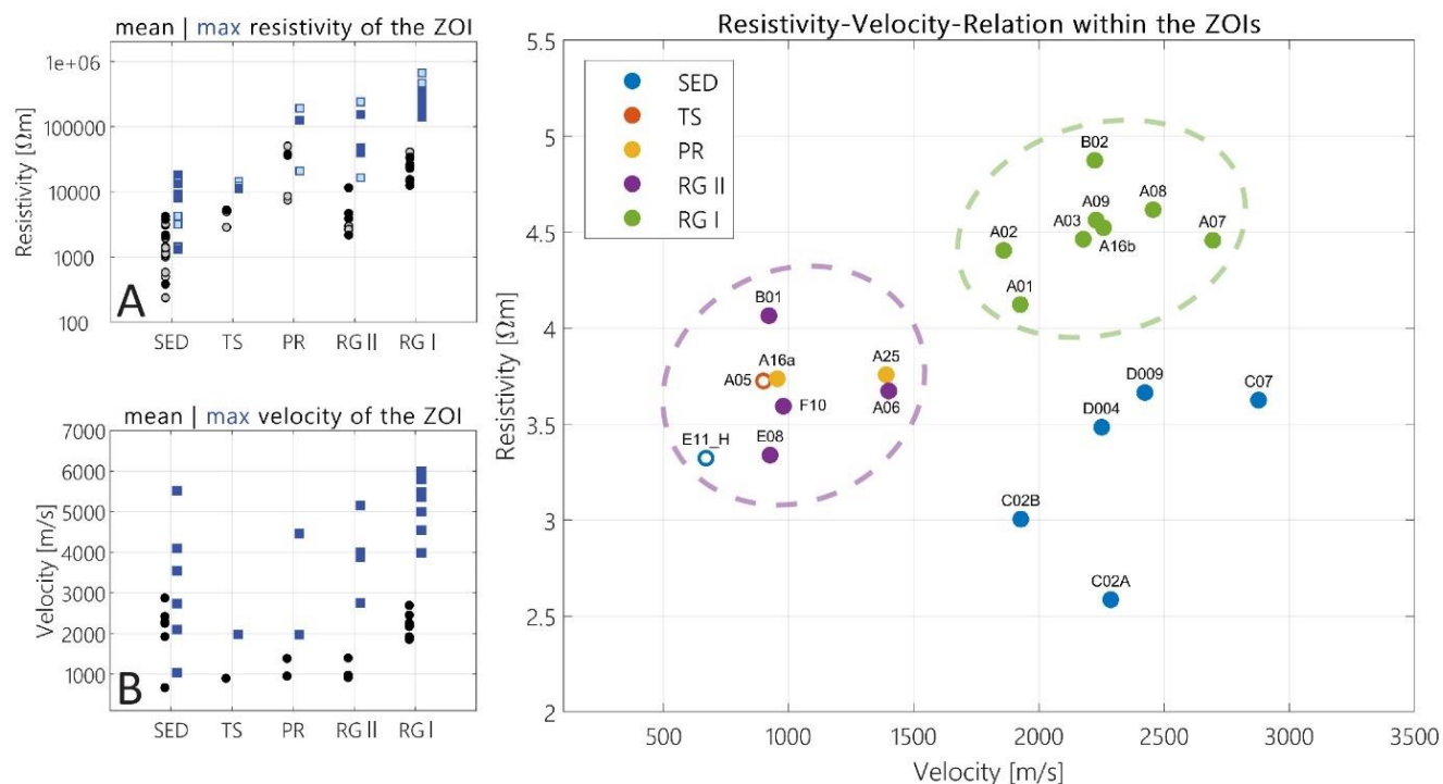
385 Figure 10: Landform-specific distribution of mean (black) and maximum (blue) values of inverted a) resistivity and b) velocity within the ZOIs of the respective ERT and RST tomograms. c) Scatter plot of mean resistivity and velocity for all co-located ERT and RST profiles, classified after landforms. Unfilled symbols in a) denote ERT profiles without co-located RST profiles. Unfilled symbols in c) denote ZOIs with only possible permafrost occurrence. Abbreviations: SED = sediment slopes (including debris-covered bedrock, colluvial slopes, gelifluction slopes, etc.); TS = talus slopes; RG = rock glaciers (groups I and II described in section 4.1.1).
