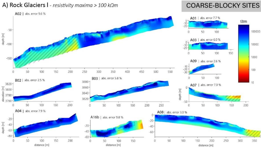
795 Figure A1: inverted tomograms of all ERT profiles from coarse-blocky sites (same spatial and colour scales), sorted by landforms
