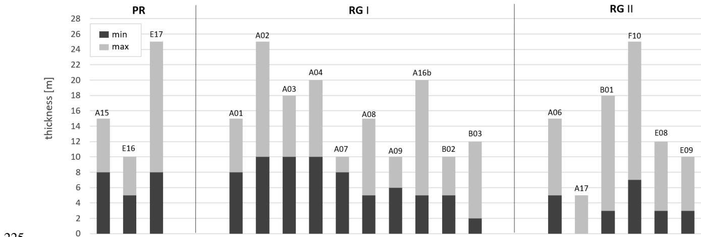
225 Figure 4: Overview over minimum and maximum thickness of ice-rich permafrost in all protalus ramparts (PR), and rock glaciers (RG) of group I and II, determined from the high-resistive zone in the ERT tomograms. Profile A17 is from a relict rock glacier with little probability for ground ice.
