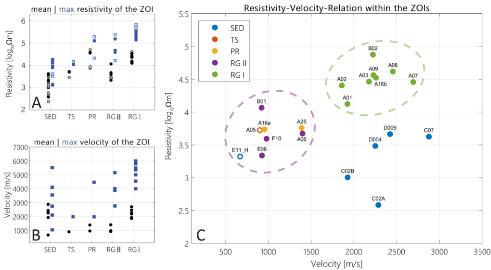
480 Figure 10: Landform-specific distribution of mean (black) and maximum (blue) values of inverted a) resistivity and b) velocity within the ZOIs of the respective electrical resistivity and refraction seismic tomograms. c) Scatter plot of mean resistivity and velocity for 485 all co-located ERT and RST profiles, classified after landforms. Unfilled symbols in a) denote ERT profiles without co-located RST profiles. Unfilled symbols in c) denote ZOIs with only possible permafrost occurrence. Abbreviations: SED = sediment slopes (including debris-covered bedrock, colluvial slopes, gelifluction slopes, etc.); TS = talus slopes; RG = rock glaciers (groups I and II described in section 4.1.1).
