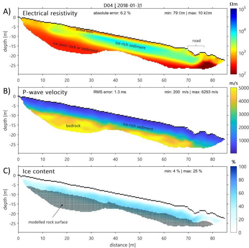
430 Figure 9: Geophysical results of profile D04 (colluvial sediments): a) section of the ERT profile covered by the RST profile (see Appendix, Fig. B2 for full profile), b) RST profile, and c) volumetric ice content modelled by the 4PM. Minimum and maximum values are indicated for all three tomograms, as well as the data misfit of both inversion models. The cross-hatched zone marks the area detected as bedrock in the 4PM. Labels denote the interpretation.
