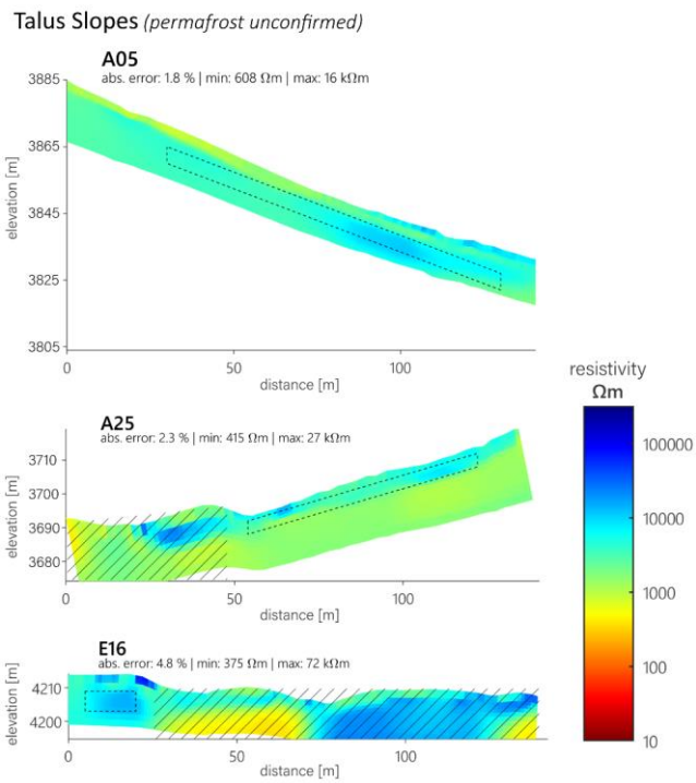
Figure 7: Inverted ERT tomograms for all talus slope profiles of the study. Zones of the tomograms not related to the talus slope are indicated by diagonal lines. The dashed rectangles mark the so-called zone-of-interest (ZOI) used for the resistivity averaging and comparison. Data misfit (absolute error in %) is indicated for each profile.
