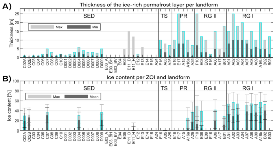
530 Figure 11: Landform-specific distribution of a) minimum and maximum thickness of the ground ice layer, and b) the mean and maximum volumetric ground ice content within the ZOIs defined before, as derived from the 4PM. The bars and error bars in b) are based on landform-specific porosity ranges indicated in the text. Abbreviations: SED = sediment slopes (including debris-covered bedrock, colluvial slopes, gelifluction slopes, etc.); TS = talus slopes; PR = protalus ramparts; RG = rock glaciers. Profiles with confirmed or probable permafrost occurrence are highlighted in light blue, while the other values are only based on zones with possible permafrost occurrence. 535
