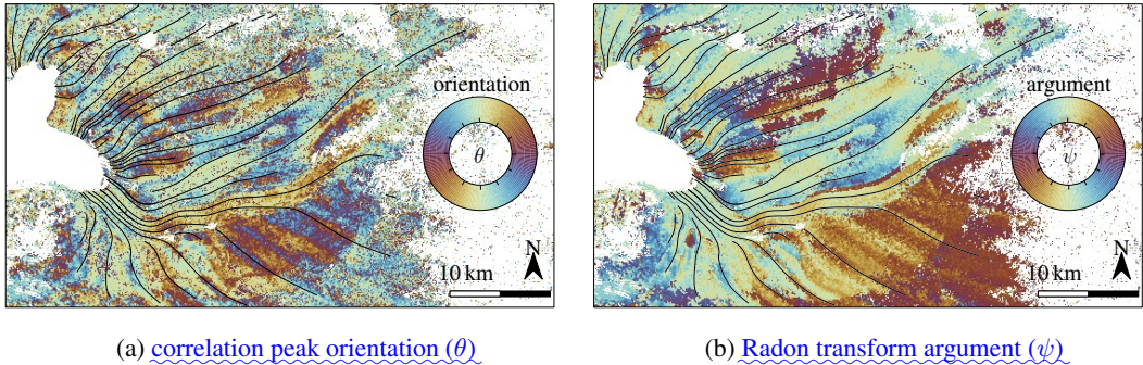
Figure 3. Correlation peak parameters for individual image matching results, describing the attitude (Fig. 3a, correspond this to Fig. 2b as well) and the strength of its a-symmetry (Fig. 4a).
