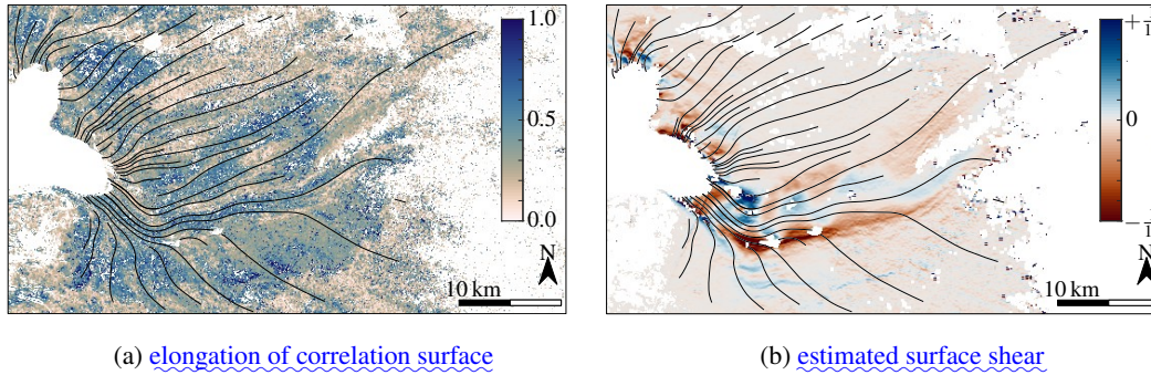
Figure 4. The strength of a-symmetry of the correlation peak (a) and estimated surface shear (b).
