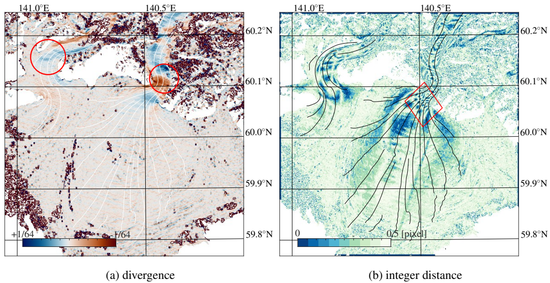
Figure 10. Estimated surface divergence, derived from the estimated velocity (Fig. 5a) and the red circles indicate regions where significant crevassing is present (Fig. 6b). The modulus from a combination of sub-pixel displacements (Fig. D2a & D2b) is shown in Fig. 10b. The red diamond indicates a pattern that is similar to the absolute correlation value as shown in Fig. 9a.
