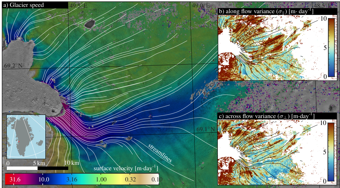
Figure 2. Colourcoded speed and streamlines of Sermeq Kujalleq (Jakobshavn Isbræ) between 20 th and 30 th of July 2020 based on Sentinel-2A imagery. The upper inset (b) shows the dominant crevasse orientation at this time based on the Radon transform along flow variance , while lower inset (c) shows the shear strain rate based on this velocity field across flow variance .
