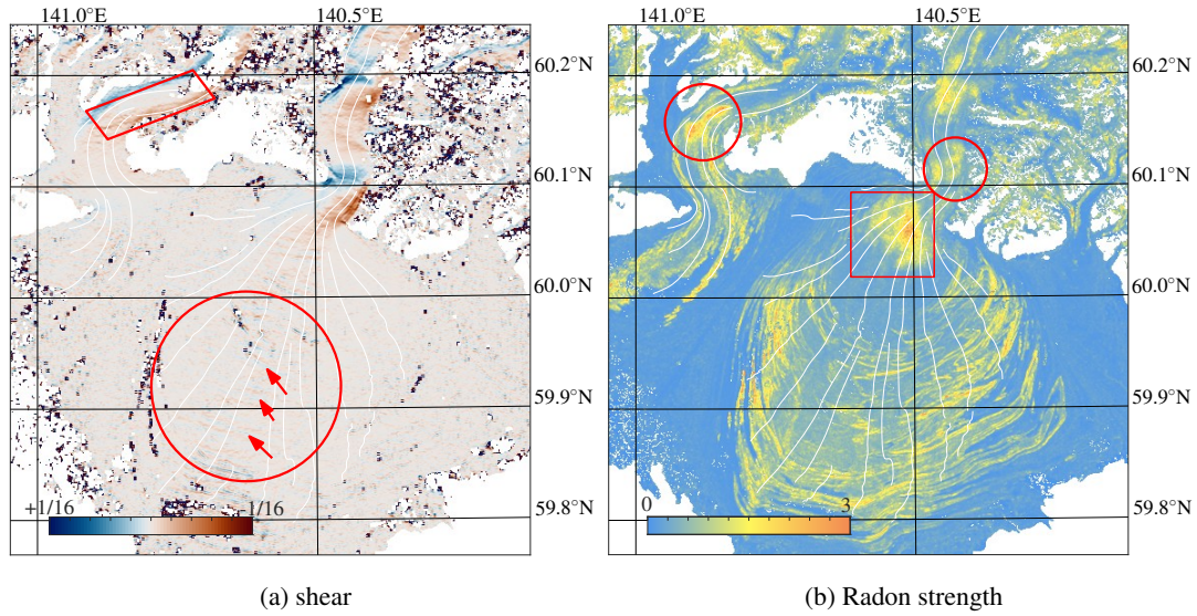
Figure 6. Estimated surface shear, derived from the estimated velocity (Fig. 5a). The red parallelogram illustrates a region with , but also regions of Malaspina Glacier have large shear rates and correspond to large elongations. Red arrows within the the large circle in the center highlight faint shear patterns that stem from sensor miss alignment (Fig. D2b). The strength of image content structure in the form of the Radon transform (Fig. 6b) has some distinct features of interest, the red rectangle highlights strong crevasses, which also results in elongated correlation spread (Fig. 5b). The red circle at Aggasiz Glacier highlights another region with strong crevasses, which also is present in the estimates of the flow divergence (Fig. 10a) and the signal to noise estimate of the image matching (Fig. 9b).
