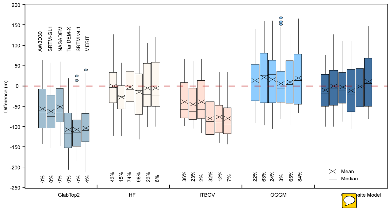
Figure 9. Point-by-point deviation comparison between the modelled and measured ice thickness from GlabTop2, HF, ITBOV, OGGM and the composite result. In each group, the boxes are plotted in the order: AW3D30, SRTM-GL1, NASADEM, TanDEM-X, SRTM v4.1 and MERIT. Different models using the same DEM are aggregated by weights (labelled at the bottom) to achieve minimum mean absolute error.
