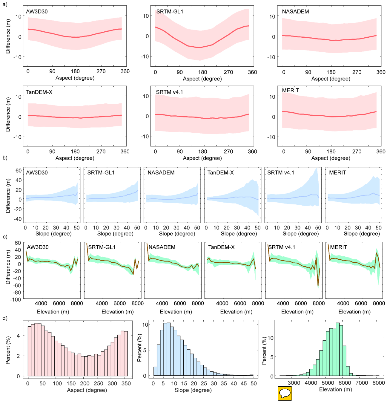
Figure 6. Differences between six DEMs and ICESat-2 with terrain factors. (a) 5° aspect bin. (b) 2° slope bin. (c) 200 m elevation bin. (d) Percentage (%) of data in each aspect, slope and elevation bin.
