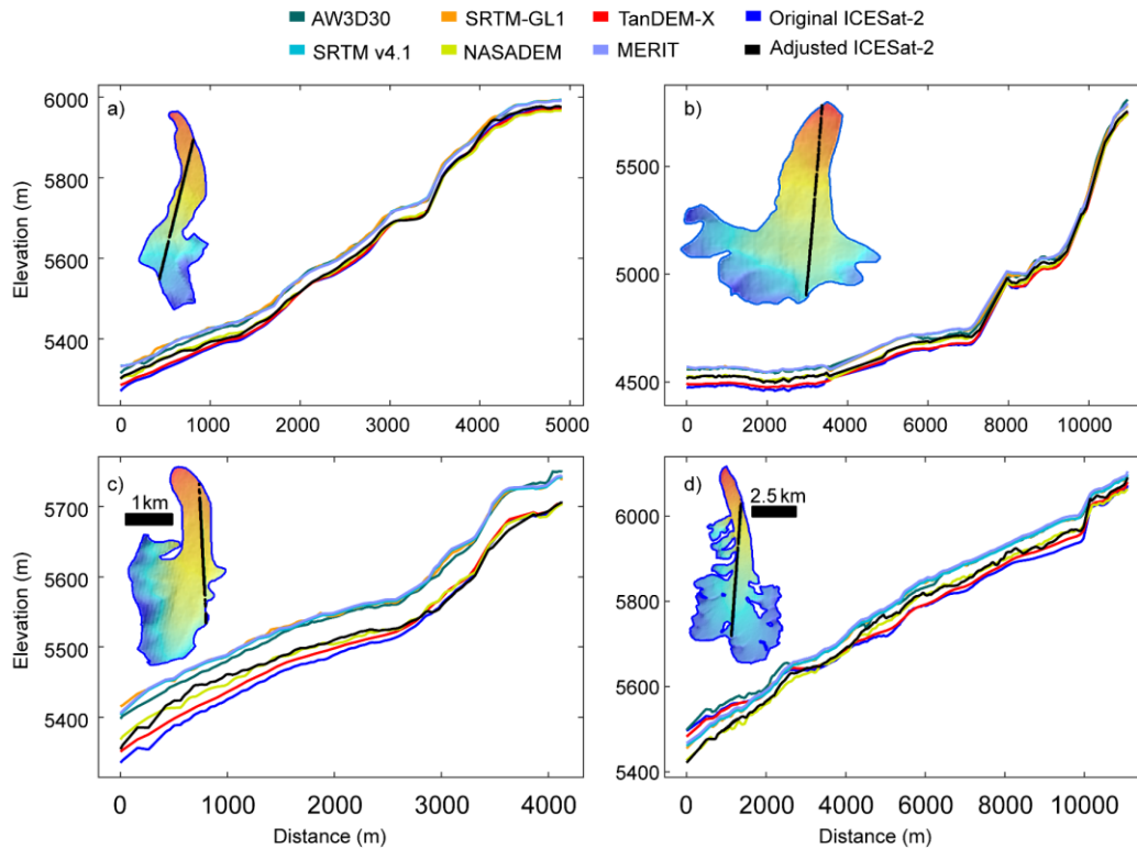
475 Figure 11. Elevation profiles of the original and adjusted six DEMs and ICESat 2 along the ICESat 2 tracks on four selected glaciers across the study region. Locations of glaciers in a–d are labelled 1–4 in Fig. 1, respectively. [49]
