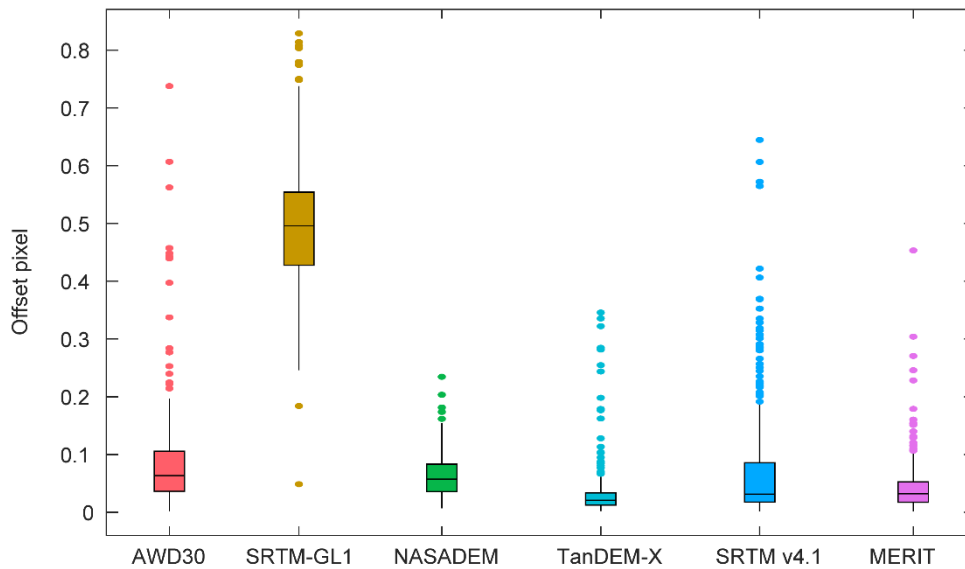
Figure 14.13. Distribution of offset pixels of DEMs relative to ICESat-2 on a 1^\circ \times 1^\circ grid. Only the grid squares with R^2 greater than 0.5 and the number of record greater than 1000 are considered.
