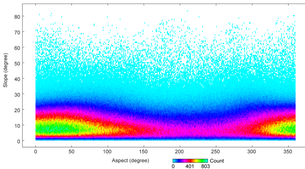
510 Figure 1312. Distribution of measurements in different slopes-aspects against the with aspectslope .
