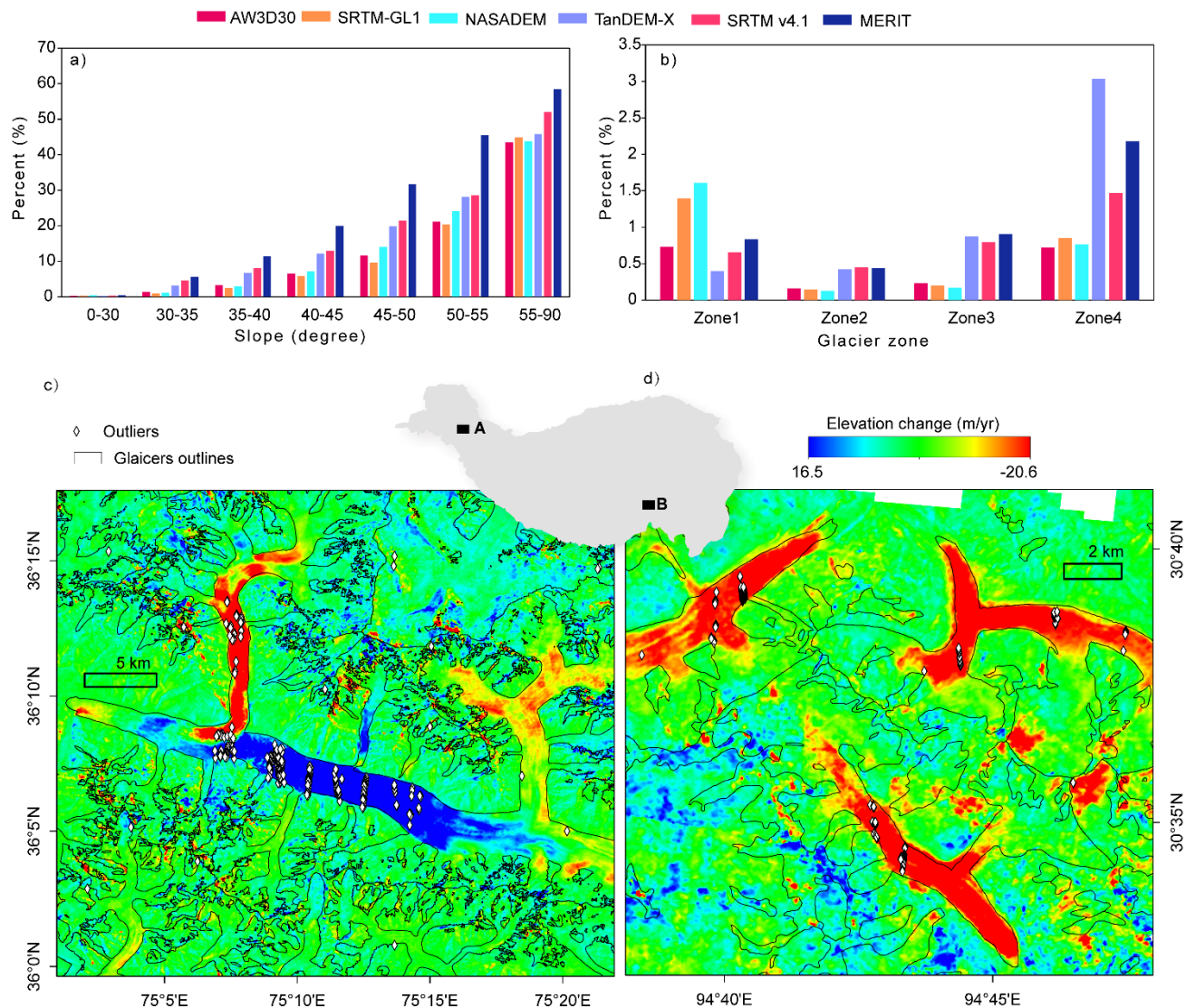
455 Figure 10. Distribution of excluded extreme outliers. The proportion of outliers accounting for the total number in slope bins (a) and each glacier Zone (b). Examples of locations of excluded points overlaid with glacier surface elevation change in the Karakoram (c) and southern TP (d). Locations of these two examples are labeled A and B in the central insert. Glacier elevation change data covering 2000–2019 is from Shean et al. (2020).
