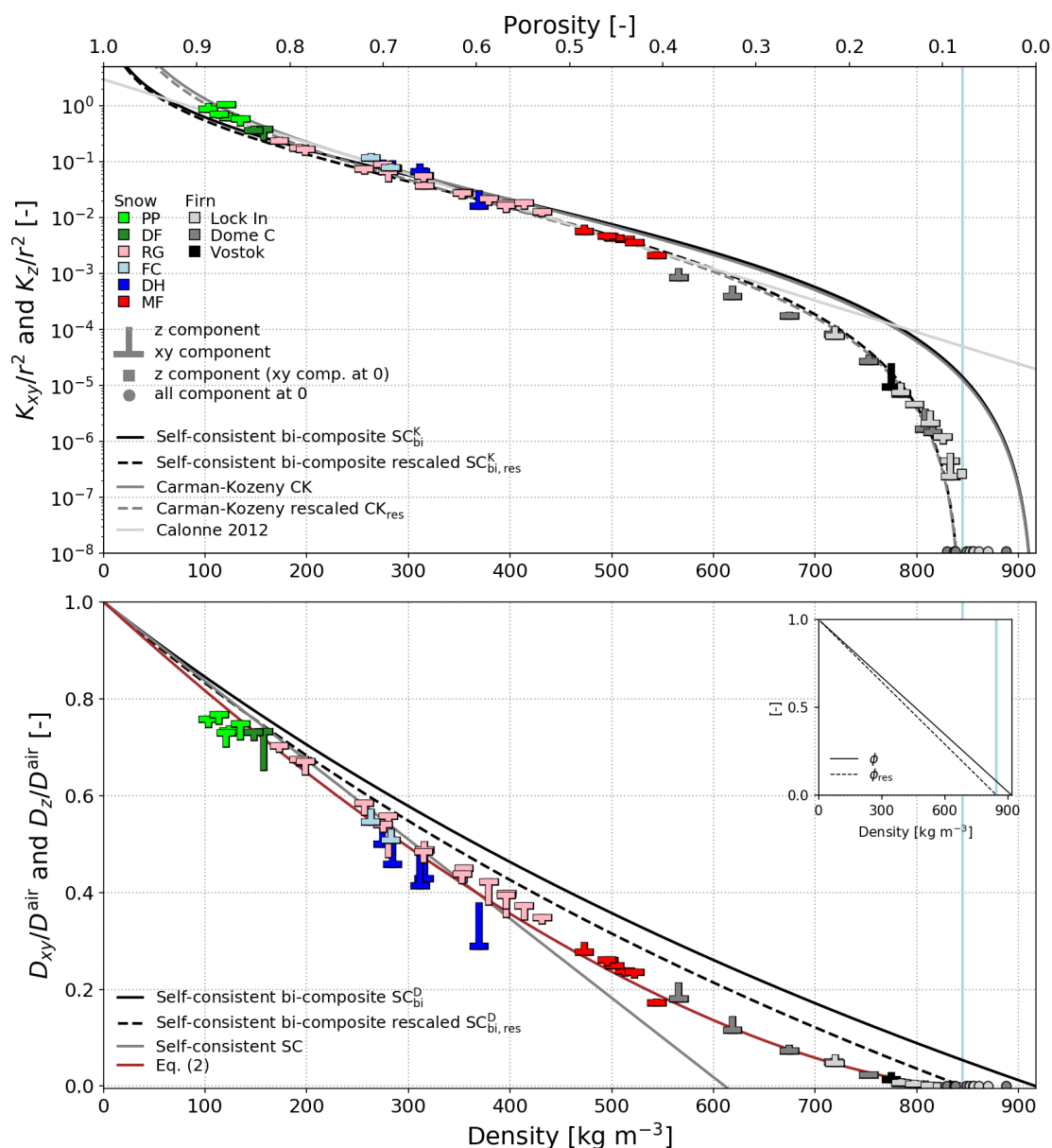
Figure 2. Dimensionless permeability and normalized diffusion coefficient of snow and firn versus density: computations on the 3D images ("T" symbols) and analytical models. The proposed regression Eq. 2 is also shown. The sub-caption shows the evolution of the rescaled porosity \phi_{res} (Eq. 1) compared to the total porosity \phi with density. Snow types correspond to the ICSSG (Fierz et al., 2009): precipitation particles (PP), decomposed and fragmented particles (DF), rounded grains (RG), faceted crystals (FC), depth hoar (DH), and melt forms (MF). The vertical blue lines at 845 \text{ kg m}^{-3} indicate the close-off density.
