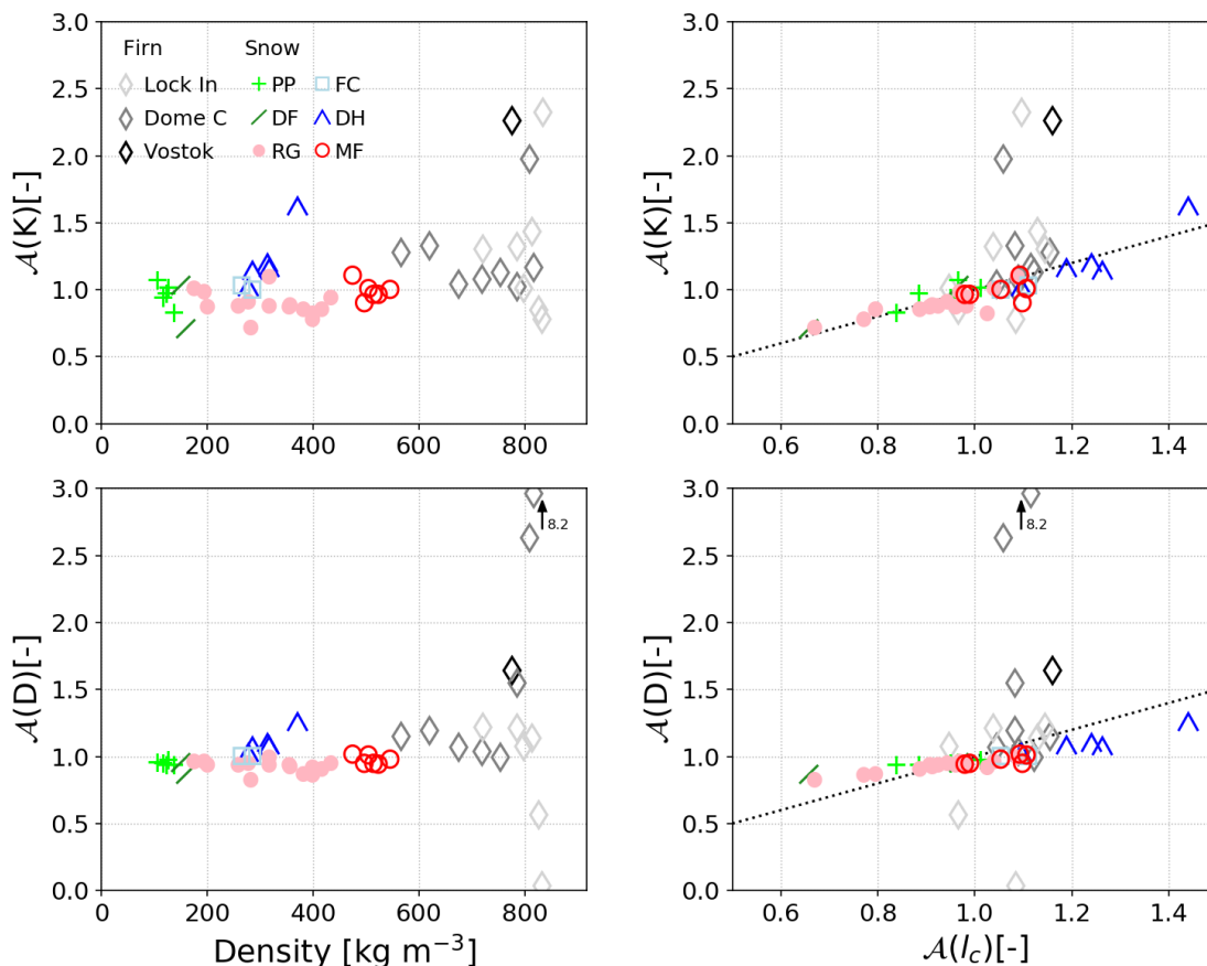
Figure 4. Relationships of the anisotropy ratio of the permeability tensor \mathcal{A}(K) (top) and of the diffusion coefficient tensor \mathcal{A}(D) (bottom) with density and structural anisotropy \mathcal{A}(I_c) . The arrows indicate a value of \mathcal{A}(D) of 8.2 at a density 832 \text{ kg m}^{-3} for a firn sample from Lock In.
