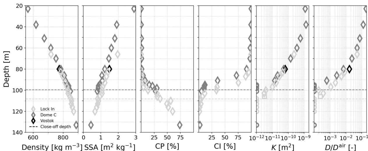
Figure 1. Evolution of firn properties with depth: density, specific surface area, closed-to-total porosity ratio, connectivity index, averaged permeability, and averaged effective coefficient of diffusion (from left to right). Dashed lines show the close-off depth at Dome C and Lock In, as given in Burr et al. (2018). Circle symbols indicate values of permeability and effective diffusion equal to zero. Square symbols show a Lock In sample (106 m depth) with horizontal components of the transport properties equal to zero and correspond thus to the values of the vertical component only.
