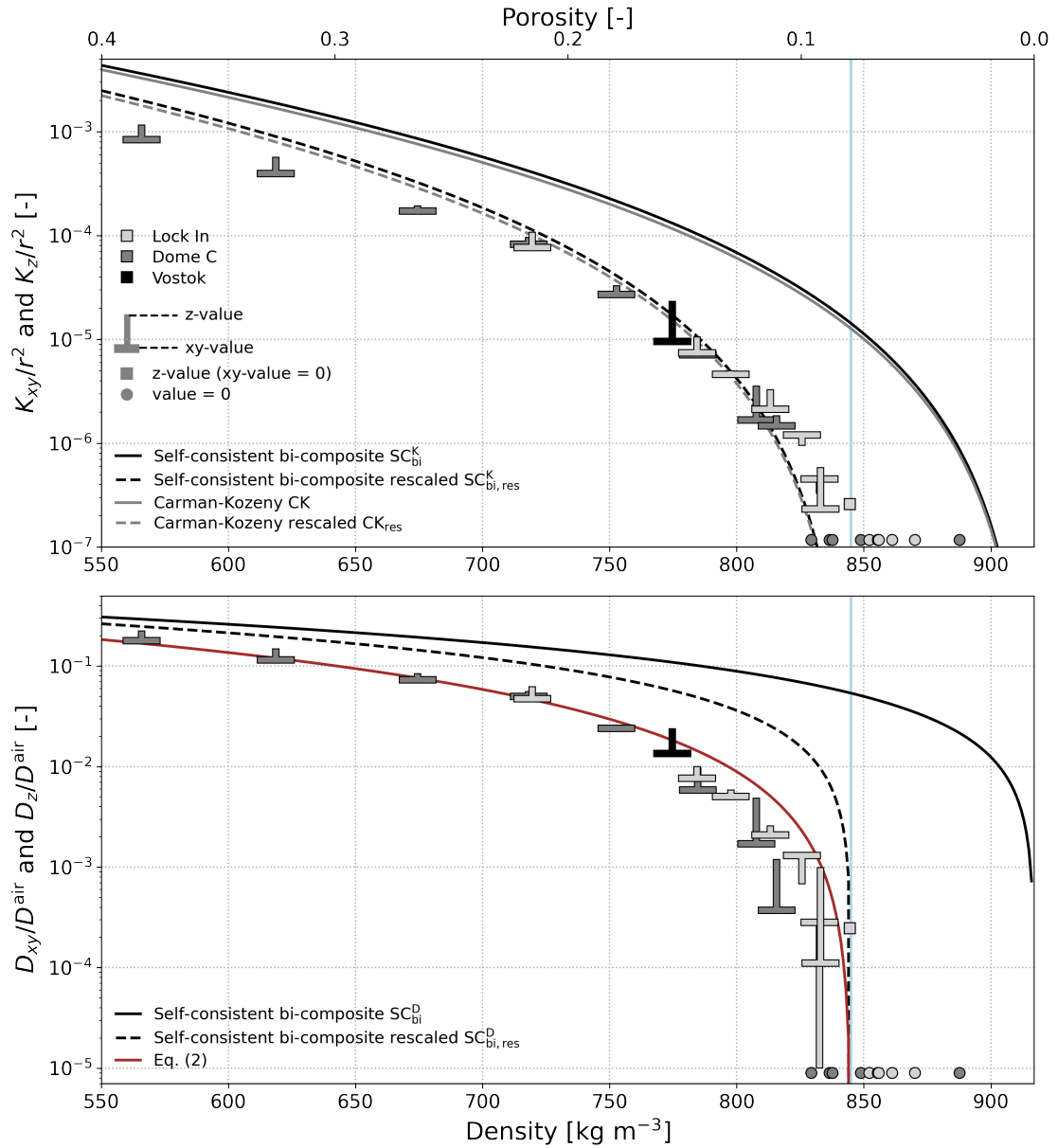
Figure 3. Dimensionless permeability and normalized diffusion coefficient of firm versus density: computations on the 3D images ("T" symbols) and analytical models (lines). The proposed regression Eq. 2 is also shown. The vertical blue lines at 845 \text{kg m}^{-3} indicate the close-off density.
