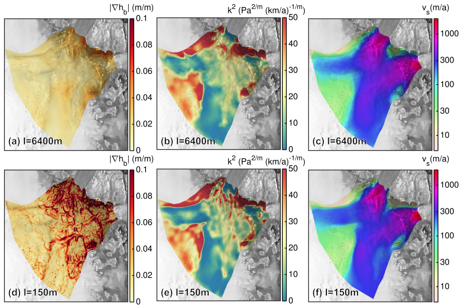
Figure 6. Overview of input parameters and exemplary simulation results of the outlet NEGIS subsetregion . Upper row shows slope of bed topography (a), basal friction coefficient for E = 1 (b), and simulated surface velocity with FS P1P1GLS-weak and m = 3 , and (c) for 6400 m horizontal resolution. Lower rows shows the same fields but for 150 m horizontal resolution. Background image is a RADARSAT Mosaic (Joughin, 2015; Joughin et al., 2016).
