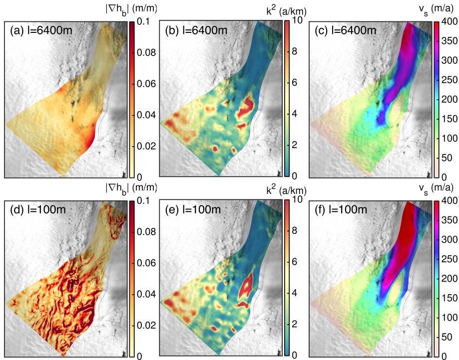
Figure 3. Overview of input parameters and exemplary simulation results of the ice-stream NEGIS subset region . Upper row shows slope of bed topography (a), basal friction coefficient for E = 1 inferred with ISSM (b), and simulated surface velocity with FS, E = 1 , m = 1 and with FS PIPIGLS-strong (c) for 6400 m horizontal resolution. Lower rows shows the same fields but for 100 m horizontal resolution. Background image is a RADARSAT Mosaic (Joughin, 2015; Joughin et al., 2016).
