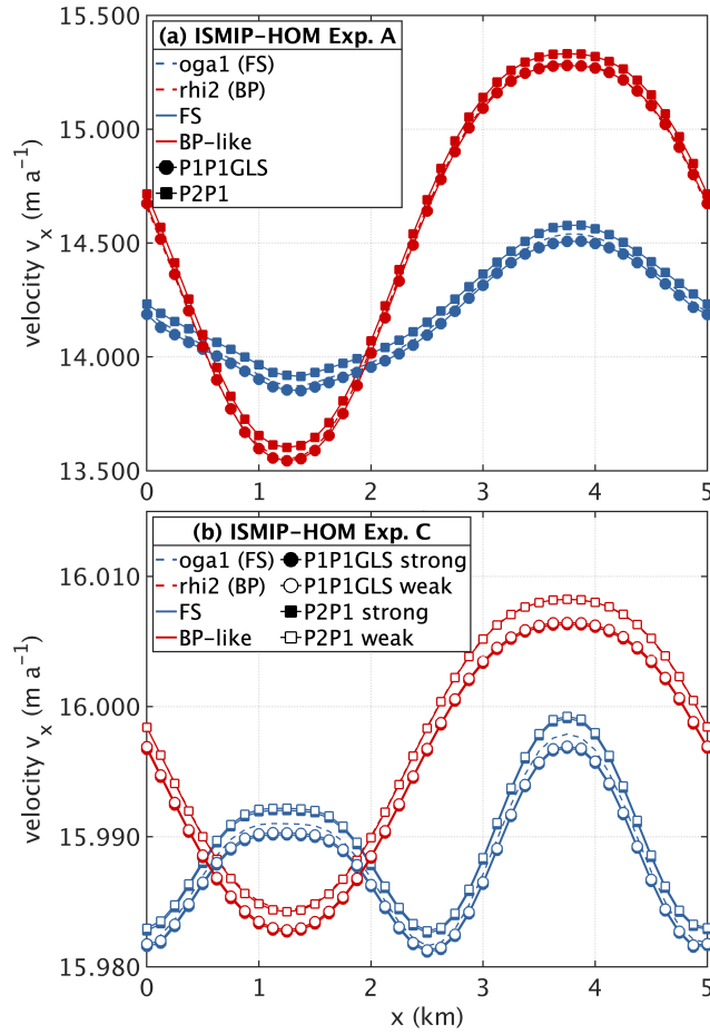
Figure 1. Results of the ISMIP-HOM experiments A (a) and C (b) for the length scale L = 5 km. Surface velocity component v_x ( \text{m a}^{-1} ) at y = L/4 . Values computed in this study for FS and BP-like are compared to the BP model 'rhi2' and the FS model 'oga1' from the original ISMIP-HOM benchmark (Pattyn et al., 2008). Please note that the BP-like P1P1GLS and 'rhi2' BP solutions in Exp. A overlay on each other; in Exp. C the 'rhi2' BP solution is overlaid by BP-like P2P1 strong and and BP-like P2P1 weak.
