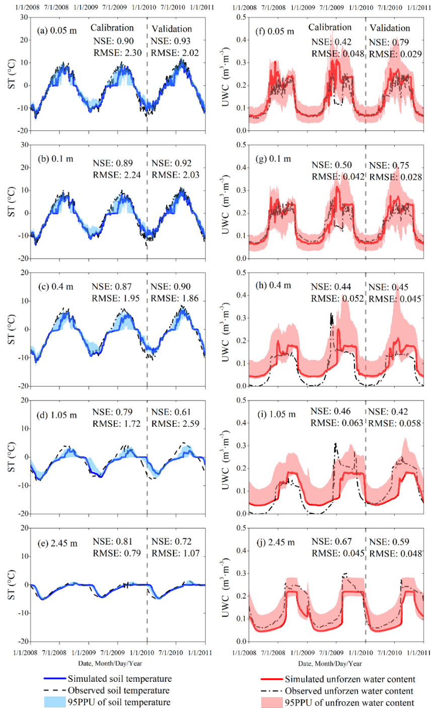
Figure 2 Simulated (solid lines) and observed (dashed lines) daily soil temperatures (ST; left panels) and unfrozen water contents (UWC; right panels) at 0.05 (a and f), 0.1 (b and g), 0.4 (c and h), 1.05 (d and i) and 2.45 m (e and j) depths at the Tanggula (TGL) site from 1 January 2008 to 31 December 2010. The simulated soil temperatures (solid blue line) and UWCs (solid red line) are the results with the optimal parameter values identified from the 1000 random parameter combinations. NSE: the Nash-Sutcliffe efficiency coefficient; RMSE: root mean square error. The 95PPUs of the model outputs are from all 1000 randomly generated parameter combinations.
