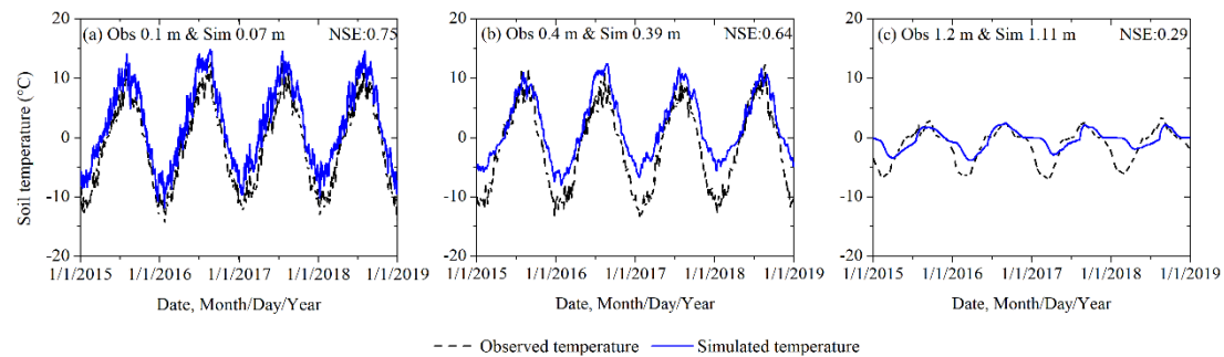
Figure A2 Validation of simulation results at different depths at QT08 against the observed daily soil temperatures during January 1, 2015 to December 31, 2018. (a) for simulation depth of 0.07 m and observation depth of 0.1 m; (b) 0.39 m for simulation and 0.4 m for observations; and (c) 1.11 m for simulation and 1.2 m for observations.
