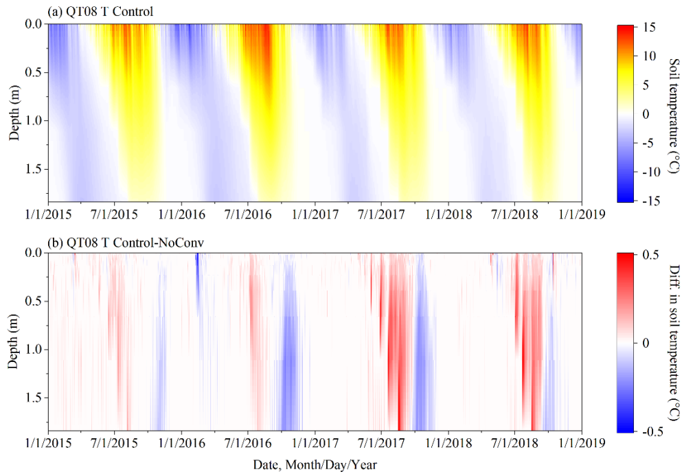
815 Figure A1 Simulated ground temperature profiles at QT08 under the Control scenario (a), and the differences in simulated soil temperature between the Control and NoConv scenarios (Control–NoConv) (b). Control and NoConv represent the scenarios with full and no consideration of convective heat transfer (CHT) in the SHAW model, respectively. Note, this figure has a different scale than Figure 4.
