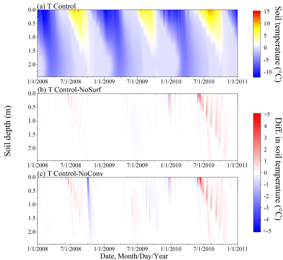
Figure 4 Simulated hourly ground temperature profiles under the Control scenario (a), and the differences in soil temperature between the scenarios: Control–NoSurf (b) and Control–NoConv (c). Control, NoSurf and NoConv represent full, partial and no consideration of convective heat transfer (CHT) in the SHAW model, respectively. NoSurf removes CHT due to infiltration and NoConv removes all CHT processes from the model.
