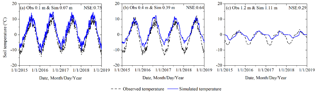
820 Figure A2 Validation of simulation results at different depths at QT08 against the observed daily soil temperatures during January 1, 2015 to December 31, 2018. (a) for simulation depth of 0.07m and observation depth of 0.1m; (b) 0.39m for simulation and 0.4 m for observations; and (c) 1.11 m for simulation and 1.2 m for observations.
