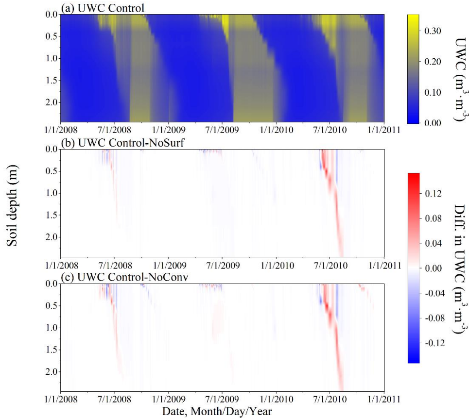
Figure 5 Simulated hourly unfrozen water content (UWC) profiles under the Control scenario (a), and the differences in UWC between the scenarios: Control–NoSurf (b) and Control–NoConv (c).
