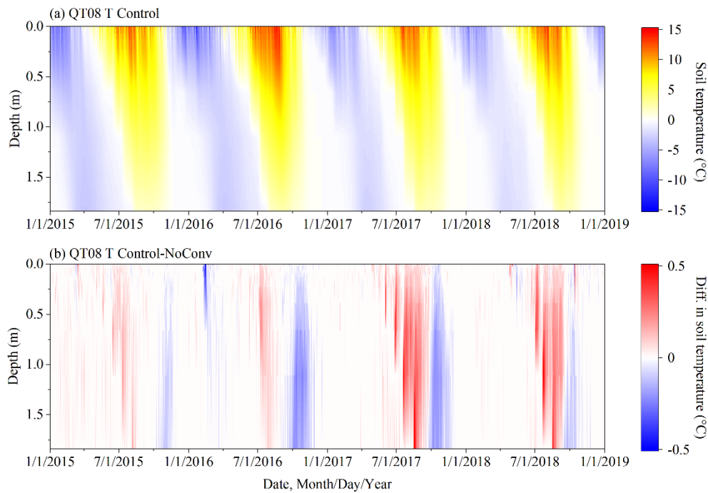
835 Figure A1 Simulated ground temperature profiles at QT08 under the Control scenario (a), and the differences in simulated soil temperature between the Control and NoConv scenarios (Control–NoConv) (b). Control and NoConv represent the scenarios with full and no consideration of convective heat transfer (CHT) in the SHAW model, respectively. Note, this figure has a different scale than Figure 4.
