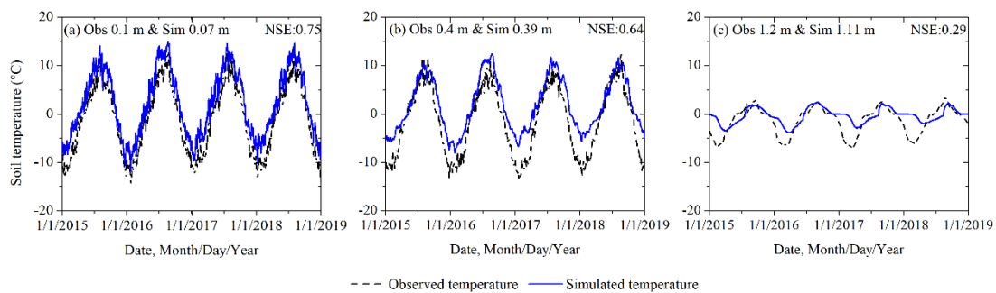
840 Figure A2 Validation of simulation results at different depths at QT08 against the observed daily soil temperatures during January 1, 2015 to December 31, 2018. (a) for simulation depth of 0.07 m and observation depth of 0.1 m ; (b) 0.39 m for simulation and 0.4 m for observations; and (c) 1.11 m for simulation and 1.2 m for observations.
