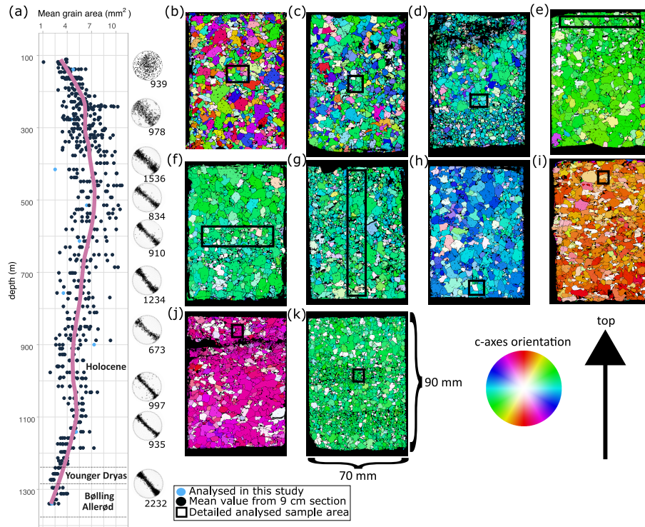
Figure 1. Grain size, CPO and fabric data from the upper 1340 m of the EGRIP ice core. a) 9 cm section mean grain sizes derived via FA G50. The violet line is a locally weighted regression with a smoothing parameter of 0.3. C-axis orientations of each section projected into a horizontal plane rotated towards their most likely position (Westhoff et al., 2020), the true orientation was lost during drilling. The number is c-axes per section. b)-k) Fabric data from the analysed thin sections. The colour code (legend) indicates the c-axes orientation, vertical c-axes appear white. Fabric image surfaces are not the same as in impurity maps due to sample processing and the focusing into the sample. Black areas are background corrections.
