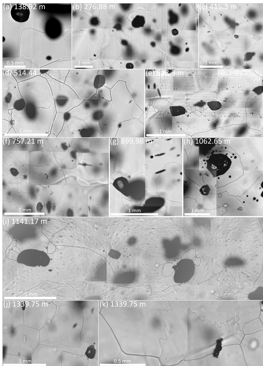
Figure 4. Microstructural observations from all depths. Dark and grey lines are grain and subgrain boundaries, respectively. Visible are bulged and cuspidate grain boundaries (A-K), different types of subgrain boundaries (A-K), and small grains at grain boundaries (C, D, E, I, J, K). Grain boundary pinning by bubbles and subgrain boundaries (B, E, I, J) and grain islands (G) also occur. Images vary in grey values due to different light conditions, grey values of lines vary due to different depths of etch grooves.
