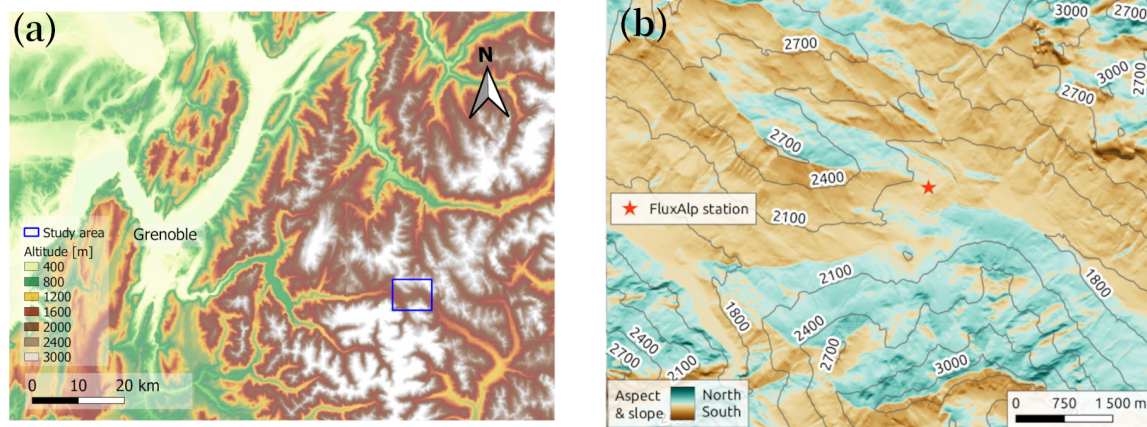
Figure 3. Location of the study area, around the Col du Lautaret alpine site. The blue rectangle in (a) represents the extension of the study area, shown in (b). The domain is generated from the RGE ALTI®Version 2.0 Digital Elevation Model (DEM) provided by IGN France at a spatial resolution of 5 m, and resampled to 10 m for this study. Slope angle is represented by the intensity of the color.
