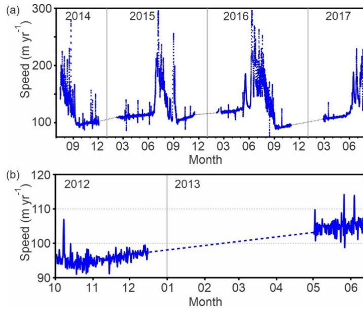
610 Figure 2. Ice flow speed measured with on-ice GPS stations and processed against base station shown in Figure 1: (a) three years of flow speed at 33 km site; (b) one winter of flow speed at 46 km site. Dashed lines indicate missing data due to GPS shutdown due to mid-winter power loss. All measurements indicate higher speeds in late winter than early winter.
