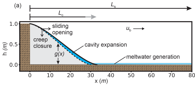
Figure 8. Cavity geometries based on the Kamb (1987) stepped-bed analysis. (a) bed and cavity geometry, showing cavity expansion as sliding speed increased over the 2016-2017 winter. Labels correspond to terms in equations 2-4 in text. Model results for three different winter periods show the stable cavity lengths required to balance sliding speed, meltwater generation, and cavity expansion under the assumption of isolated cavities. Plotted are results for a range of potential step heights: (b) final cavity length after cavity has expanded to accommodate the meltwater generated over winter period; (c) length of steps required to accommodate both the water cavity and the portion of the step in contact with ice; (d) ratio of cavity length to step length, which must be less than 1 because cavities cannot be longer than their steps.
