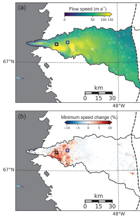
625 Figure 4. Spatial characteristics of ice flow across Isunnguata Sermia basin during winter of 2017-2018 based on MEaSUREs v2 product. (a) pattern of ice flow speed during early winter measured over month of October 2017. (b) minimum ice speed change (as percentage) from October through April; shown are the percentage speed changes minus the potential percentage change resulting from error terms. Areas showing no change could have potentially experienced an October-April speed change, but not enough to overcome errors. The 33 km and 46 km measurements sites are shown as boxes.
