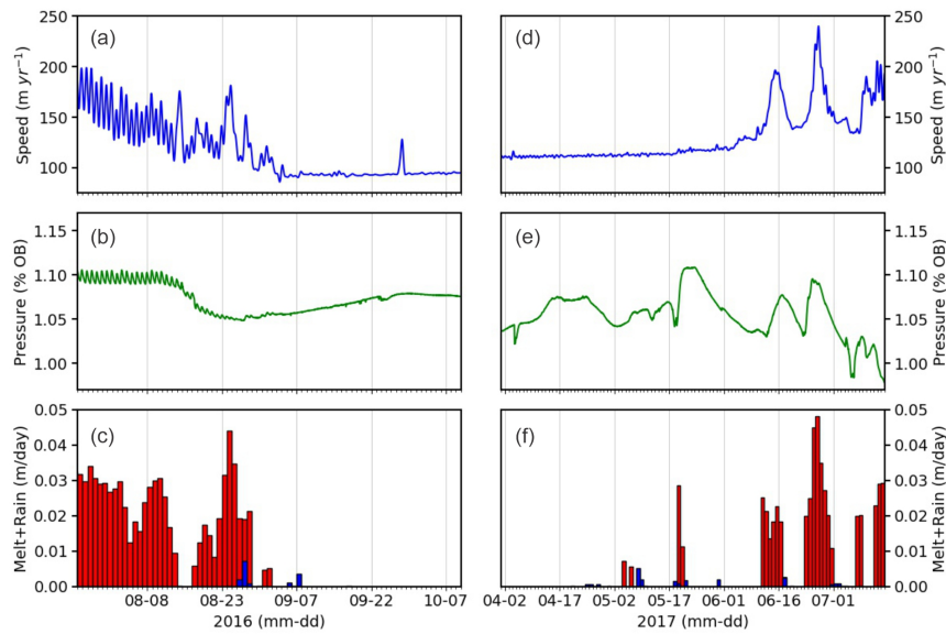
615 Figure 3. Time series of data collected at 33 km borehole site showing start and end of the winter period: (a-c) show winter onset; (d-f) show winter termination. Melt is red, rain is blue (c and f). Borehole, GPS, and meteorological instruments all located within 10 m of each other.
