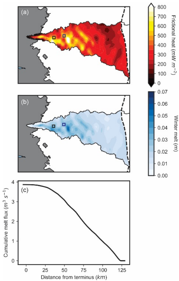
Figure 7. Basal ice melt during winter of 2017-2018 across the Isunnguata Sermia basin based on satellite velocity and model assumptions described in text: (a) Basal frictional heat rate averaged over the winter period (October through April); (b) total basal meltwater generated during the winter months; (c) Top-to-bottom accumulation of basal meltwater generation rate averaged over the winter period. Basal meltwater is integrated as a function of inland distance, irrespective of potential routing pathways.
