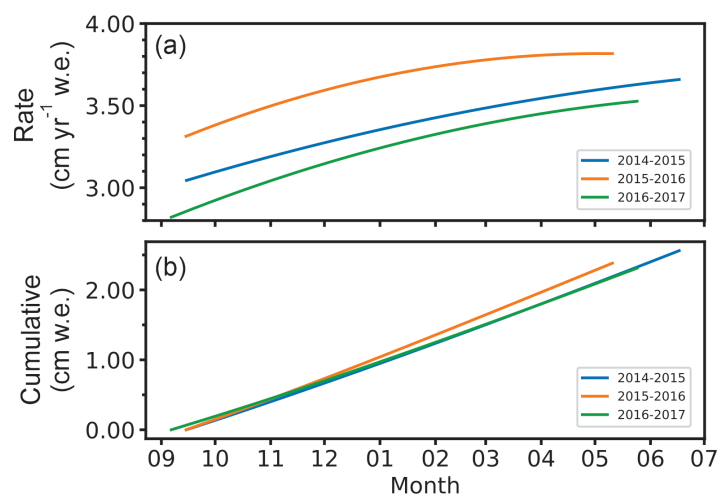
Figure 6. Basal meltwater generation at 33km site: (a) instantaneous basal melt rate in water equivalent over the winter during three different years; (b) Cumulative meltwater generation over the winter period during three years.
