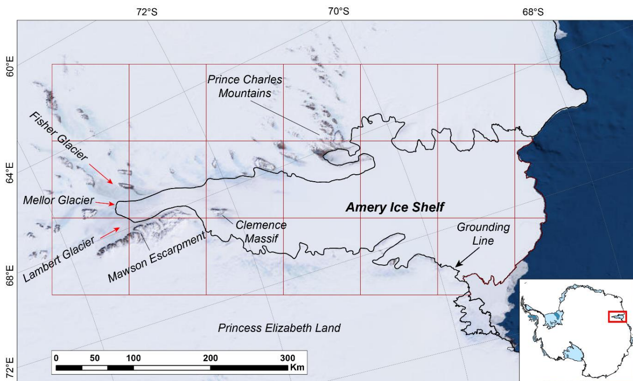
115 Figure 1. Study region over the Amery Ice Shelf, including an inset showing its location within Antarctica. The background image is a 15 m TerraColour Antarctic Basemap (ESRI). The red boxes indicate the area over which melt was mapped, with tiles representing twenty-one separate 100 by 100 km regions of interest (ROIs) for mapping within GEE. The black line marks the grounding line based on the Depoorter et al. (2013) dataset. Red arrows indicate the flow direction of labelled outlet glaciers.
