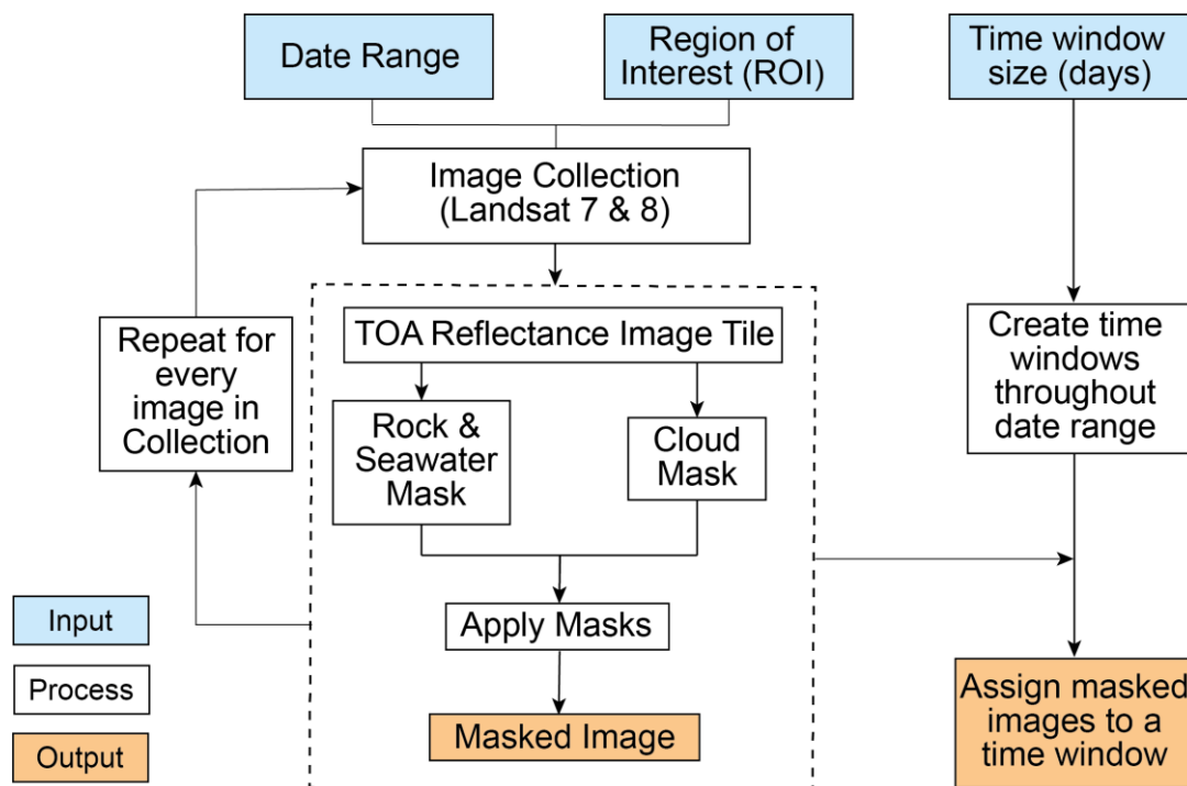
Figure 2. Flowchart illustrating the optical image masking steps taken within GEE, including the method by which images are assigned to time windows. See Table 1 for the threshold values (Moussavi et al., 2020) used during each masking stage.
