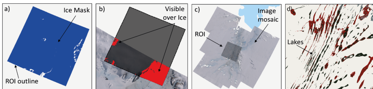
195 Figure 3. Flowchart detailing the method used to conduct lake visibility assessments within GEE for each time window. Images (a-d) provide visual examples of selected stages, and are referred to within the flowchart. The different lake colours in (d) indicate which optical image each lake pixel has originated from (e.g. Red = Image 1, Black = Image 2 etc.). If the same
