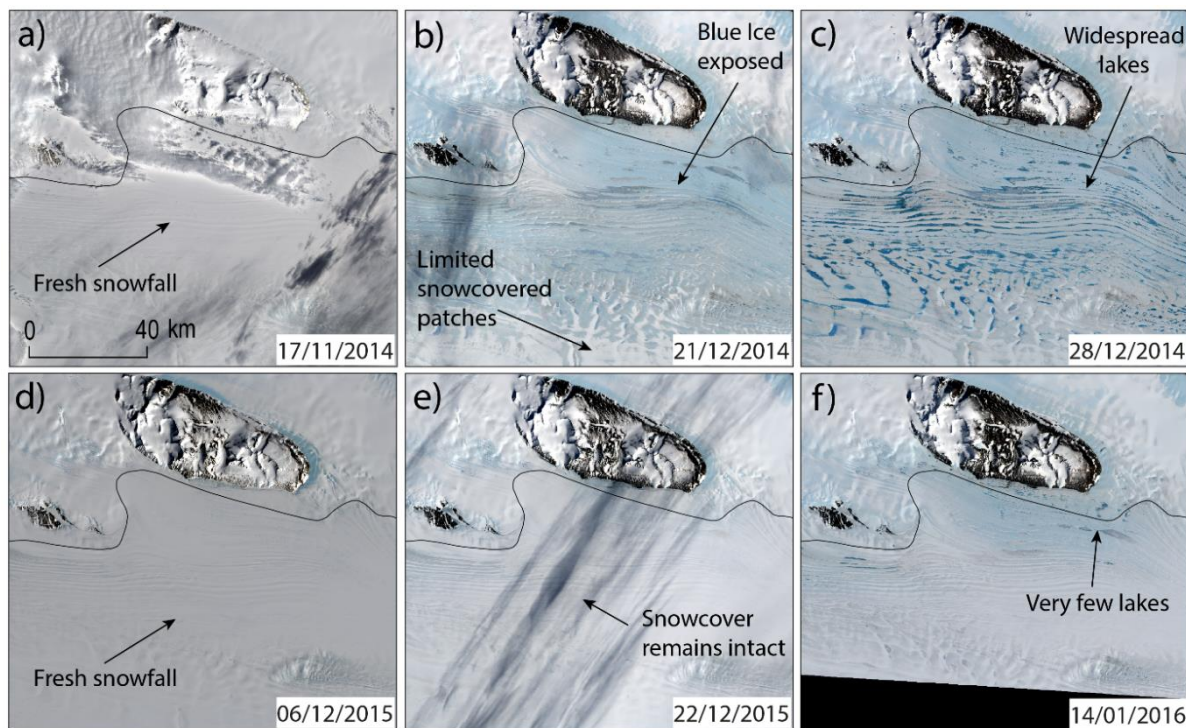
Figure 11. Landsat 8 images showing the evolution of the ice shelf surface to the east of the Fisher Massif in the 2014/15 (a-c) and 2015/16 (d-f) melt seasons.
