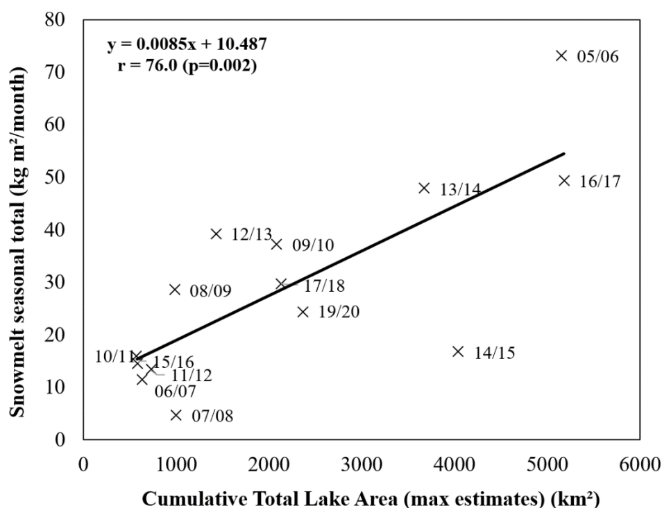
Figure 9. Scatter plot and correlation statistics of the relationship between cumulative RACMO melt and cumulative lake area over the study region per melt season.
