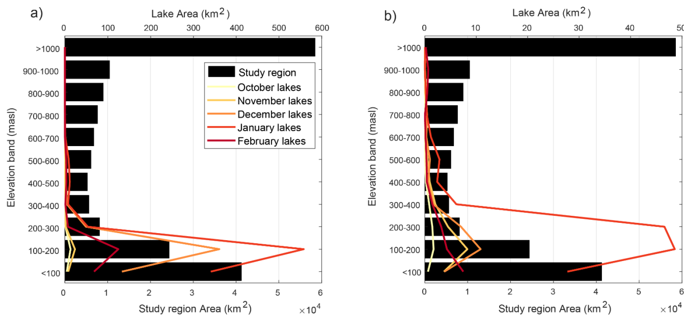
Figure 7. Averaged total lake areas per month by elevation bands, for a high melt season (a, 2005/06) and a low melt season (b, 2015/16). Black horizontal bars show the hypsometry of the study region. Note the total lake area is an order of magnitude greater during the high melt year (see lake area scales).
