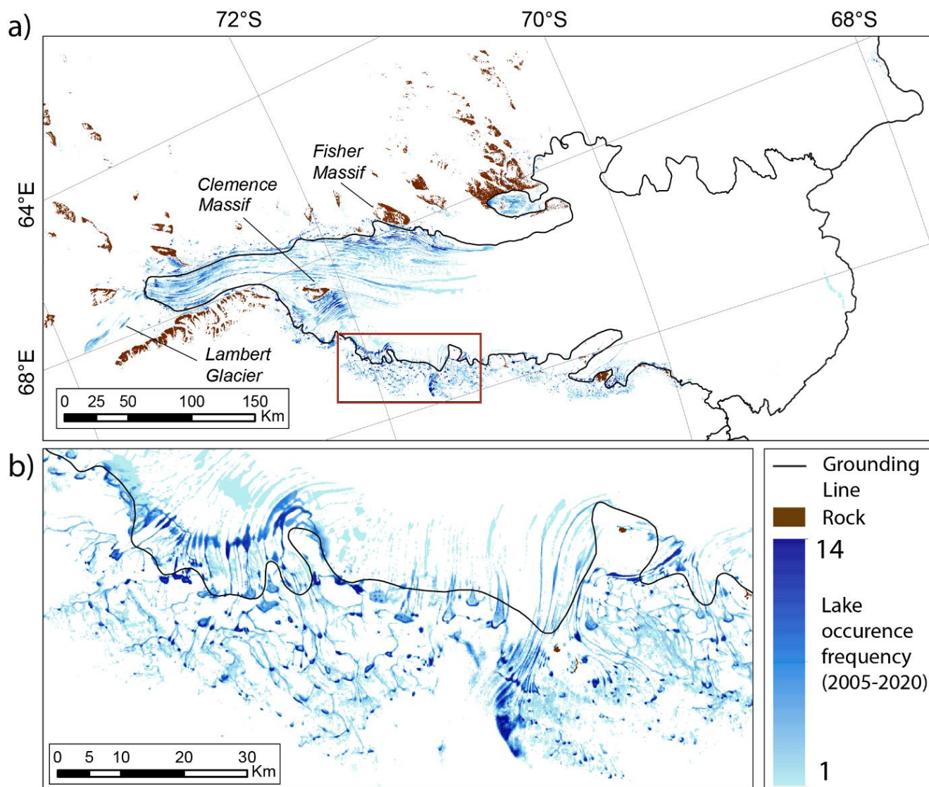
335 Figure 6. Spatial distribution of SGLs over the study region, showing the recurrence frequency of surface meltwater between 2005 and 2020. The maximum recurrence frequency is 14 years, due to the exclusion of the 2004/05 and 2018/19 melt seasons. Pixels were assigned values of 1 (melt) or 0 (no melt) per year, based on the occurrence of surface water at any stage during each melt season. Pixels were then summed to derive recurrence frequency. The linear light blue feature near the ice shelf 340 2021).
