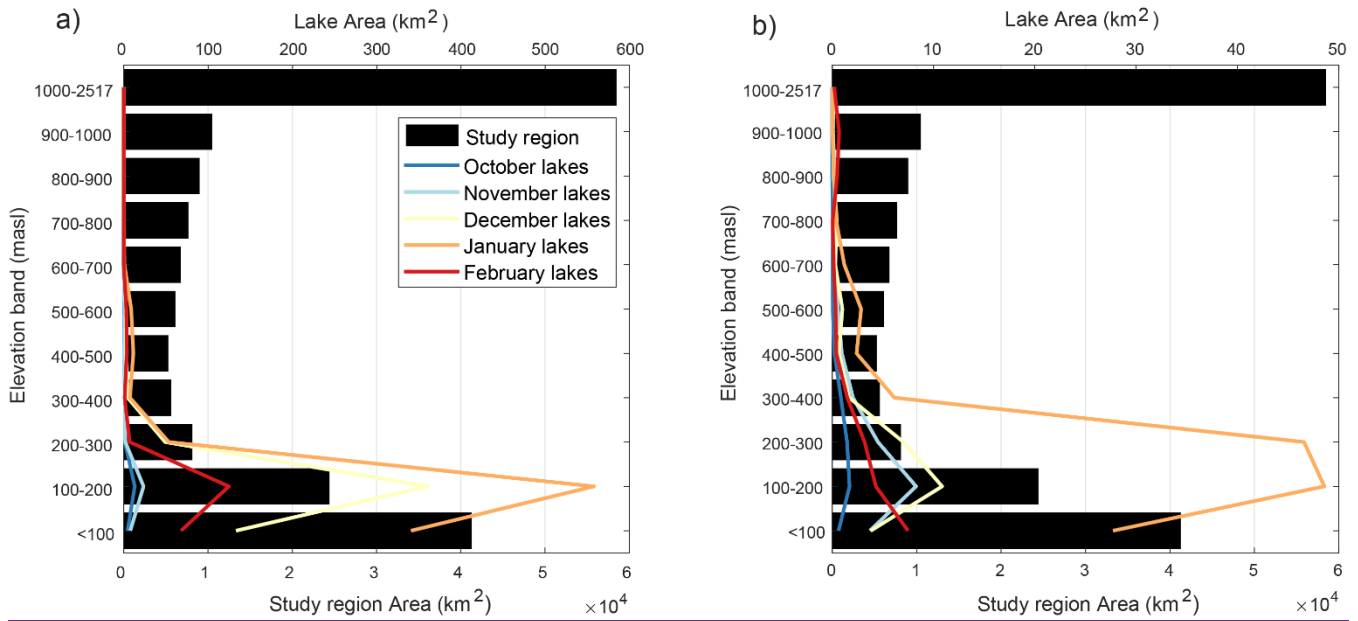
390 Figure 7. Averaged total lake areas per month by elevation bands, for a high melt season (a, 2005/06) and a low melt season (b, 2015/16). Black horizontal bars show the hypsometry of the study region. Note the total lake area is an order of magnitude greater during the high melt year (see lake area scales).
