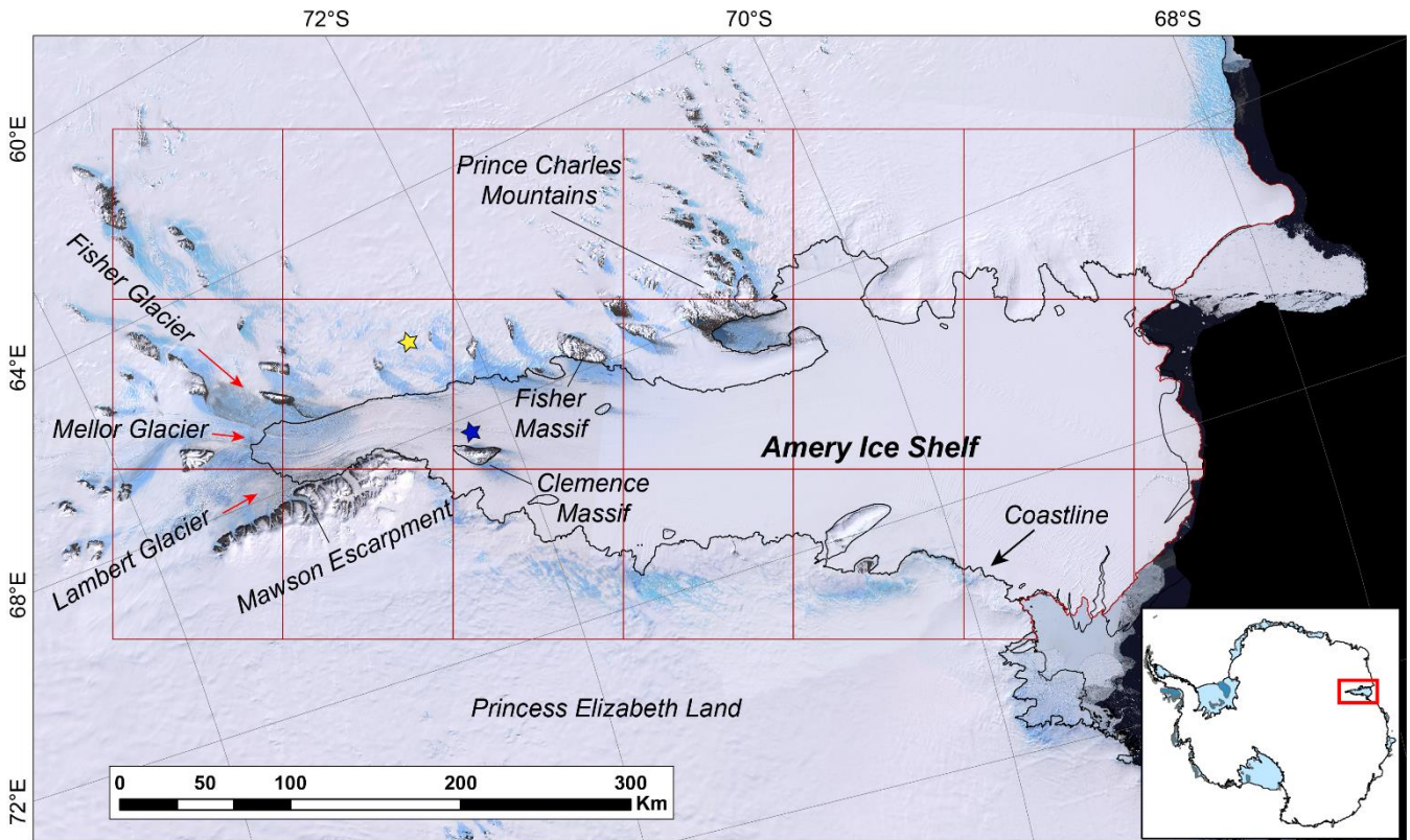
120 Figure 1. Study region over the Amery Ice Shelf, including an inset showing its location within Antarctica. The background image is a 15 m TerraColour Antarctic Basemap (ESRI) -the Landsat Image Mosaic of Antarctica (LIMA) . The red boxes indicate the area over which melt was mapped, with tiles representing twenty-one separate 100 by 100 km regions of interest (ROIs) for mapping within GEE. The black line marks the grounding line based on coastline from the Depoorter SCAR Antarctic Digital Database (Gerrish et al. (2013) dataset., 2021) . Red arrows indicate the flow direction of labelled outlet 125 glaciers. The blue and yellow stars represent the location of Figure 5a/c and 5b respectively.
