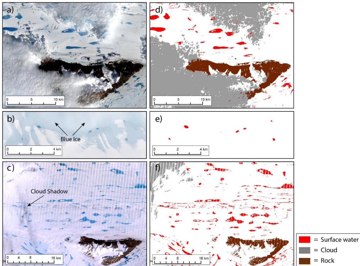
335 Figure 5. (a) Landsat 8 image from 25 th January 2017 of the Clemence Massif; (b) Landsat 8 image from 1 st January 2019, highlighting blue ice ~100 km south of Fisher Massif; (c) Landsat 7 image from 2 nd January 2005, showing widespread surface lakes to the west of the Clemence Massif. Note the white stripes resulting from the failure of the Landsat 7 scan line corrector. (d-f) Automatic masking of cloud, rock and surface water from Landsat imagery.
