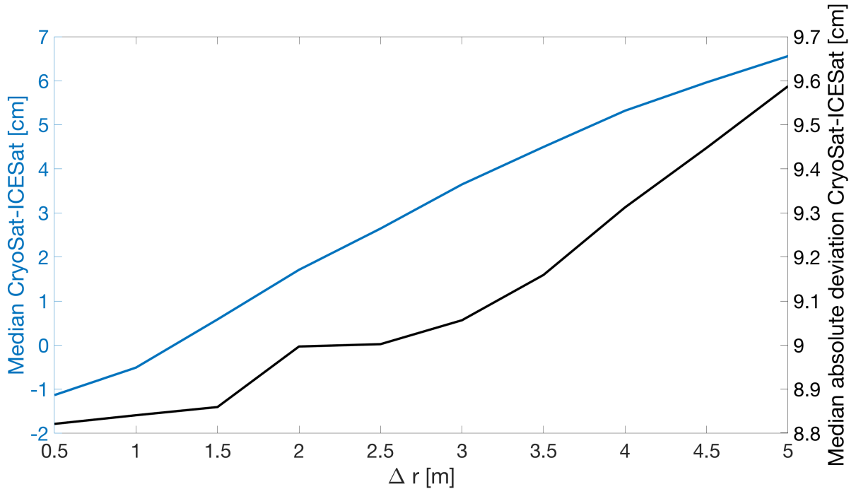
Figure 5. Median (left axis) and median absolute deviation (right axis) of the height differences between CryoSat-2 and ICESat-2 ( \Delta h calculated with Eq. (16)) as function of \Delta r . Outliers are removed using 10th and 90th percentiles.
