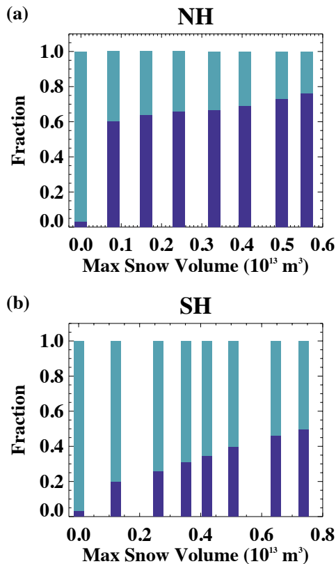
Figure 11. The fraction of the total ice area occupied by seasonal ice (light blue) and perennial ice (dark blue) as a function of 450 the maximum snow volume across the experiments. Values are shown for the (a) Northern Hemisphere and (b) Southern Hemisphere.
