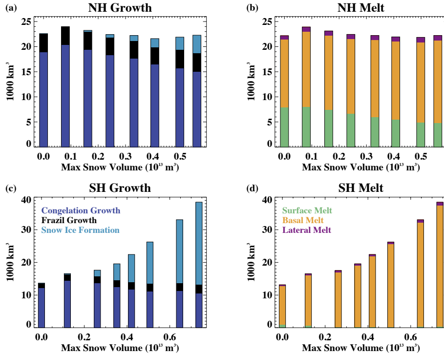
Figure 8. The volume of total annual (a) Northern Hemisphere ice growth, (b) Northern Hemisphere ice melt, (c) Southern Hemisphere ice growth, and (d) Southern Hemisphere ice melt as a function of the maximum snow volume across the simulations.
