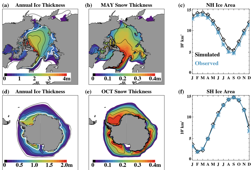
Figure 1. The simulated Northern Hemisphere (a) annual ice thickness, (b) May snow depth, (c) ice area and Southern Hemisphere (d) annual ice thickness, (e) October snow depth, and (f) ice area. On the ice thickness plots, the contour interval for the black lines is 0.5m and the simulated 15% ice concentration for March and September are shown in the bold white and grey contour lines. For the snow thickness plots, the contour interval for the black lines is 0.1m. Observed ice area averaged from 1979-2013 shown on panels (c) and (f) is from the NSIDC sea ice index (Fetterer et al., 2017).
