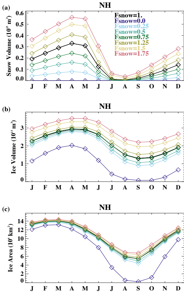
Figure 3. The Northern Hemisphere (a) snow volume, (b) ice volume and (c) ice area in the different Fsnow experiments.
