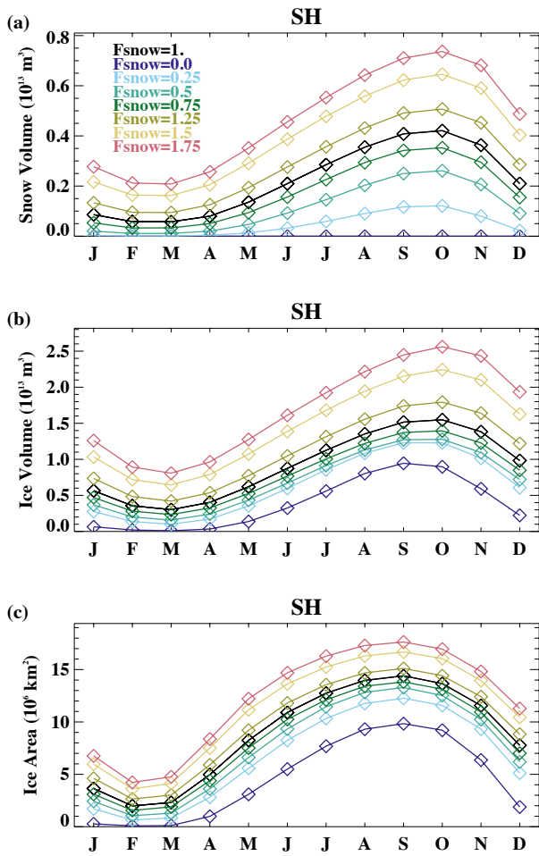
325 Figure 5. The Southern Hemisphere (a) snow volume, (b) ice volume and (c) ice area in the different Fsnow experiments.
