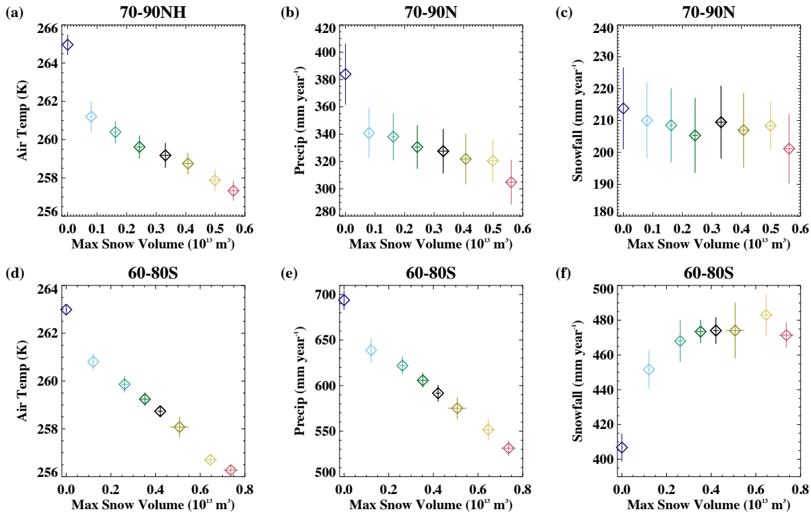
345 Figure 7. The relationship of the climatological 70-90N (a) annual average surface air temperature, (b) annual total precipitation, (c) annual total snowfall versus the annual maximum Northern Hemisphere volume of snow on sea ice across the simulations. Bottom panels show conditions for 60-80S versus the Southern Hemisphere snow volume for (d) annual mean surface air temperature, (e) annual total precipitation, and (f) annual total snowfall. The whiskers show +/- one standard deviation across the 20 years analyzed for each simulation.
