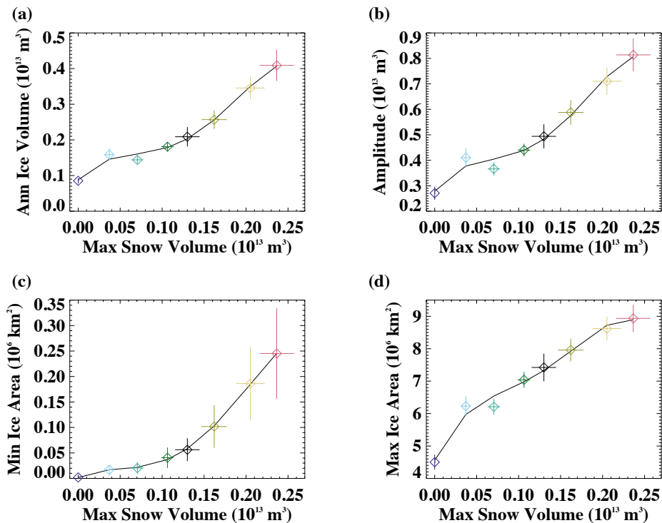
Figure 13. As in Figure 12 but for Southern Hemisphere values in the 2\times\text{CO}_2 climate.
