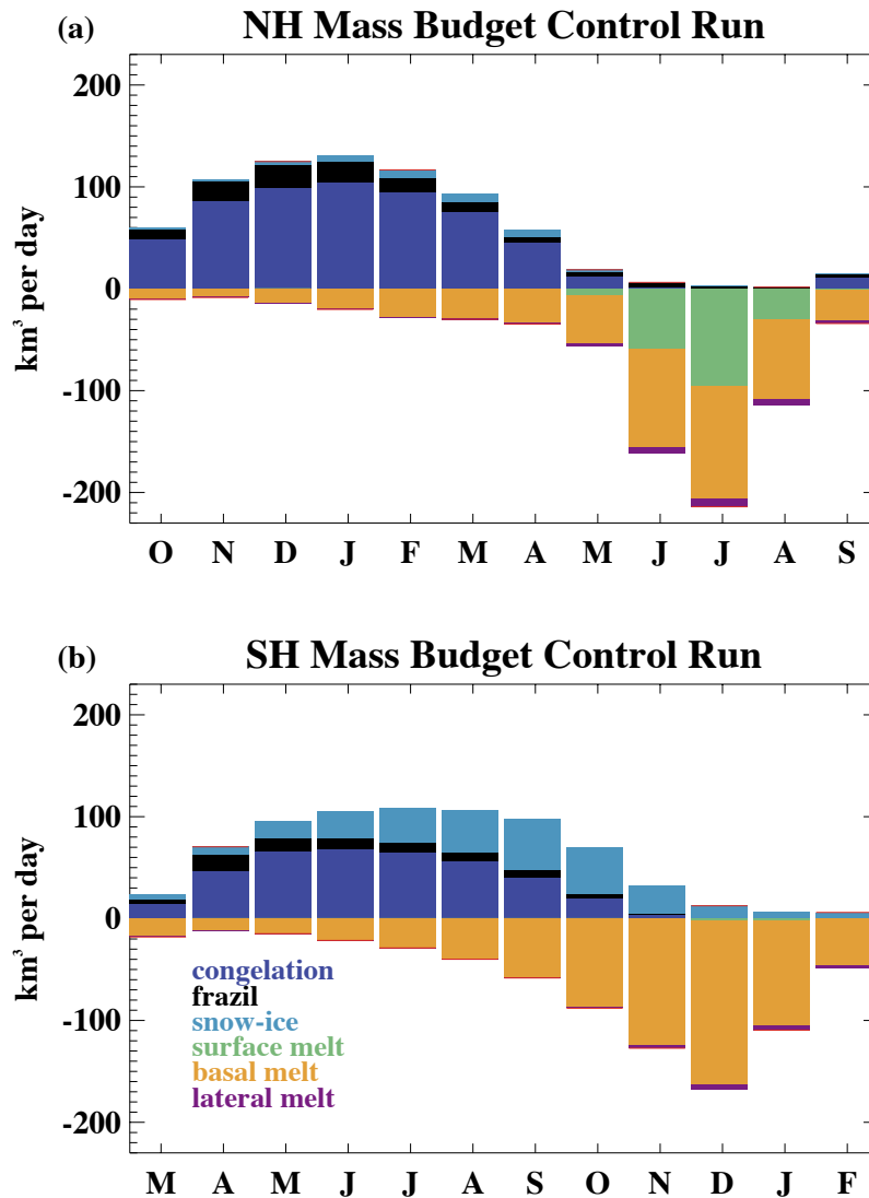
Figure 2. Annual cycle of the climatological ice volume budgets in the F_{\text{snow}}=1 preindustrial control run for the (a) Northern Hemisphere and (b) Southern Hemisphere. The volume budgets can be directly converted into mass budgets using the constant sea ice density of 917 \text{ kg/m}^3 used in the model. Note that the annual cycle is shifted in both hemispheres to begin with the ice growth season (starting in October for panel (a) and March for panel (b)). Values are computed over the entire hemisphere.
