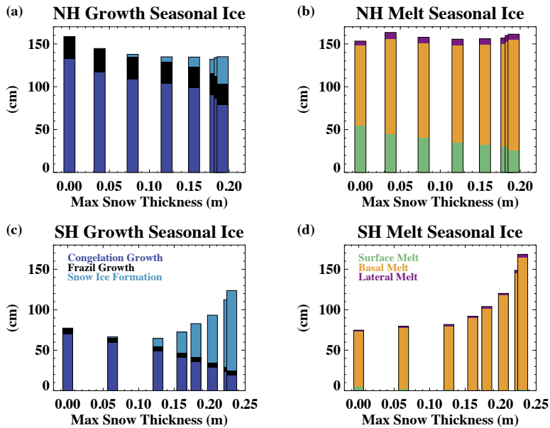
Figure 10. As in Figure 9 but for the seasonal sea ice region.
