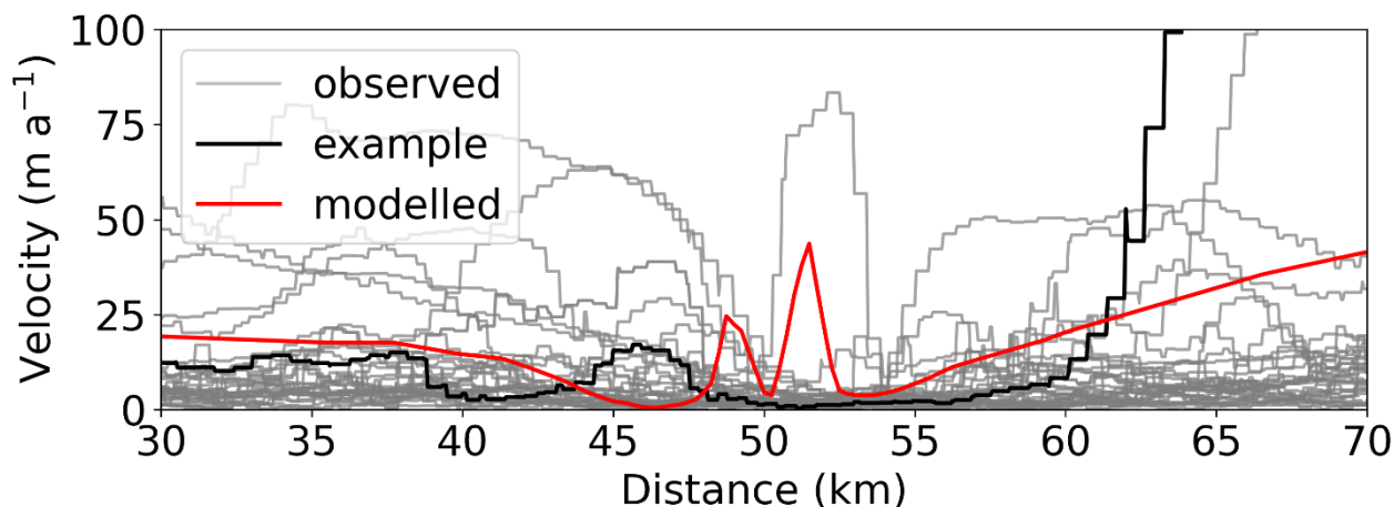
Figure S6. Surface velocity profiles across 33 nunataks (grey, observed; black line refers to the example profile in d; Mouginot et al., 2012) and along the spun-up ice cap centreline (red, modelled); only the first 20 km up and downstream of the nunatak are shown for a better visualisation (nunatak summits are centred on x=50 km).
