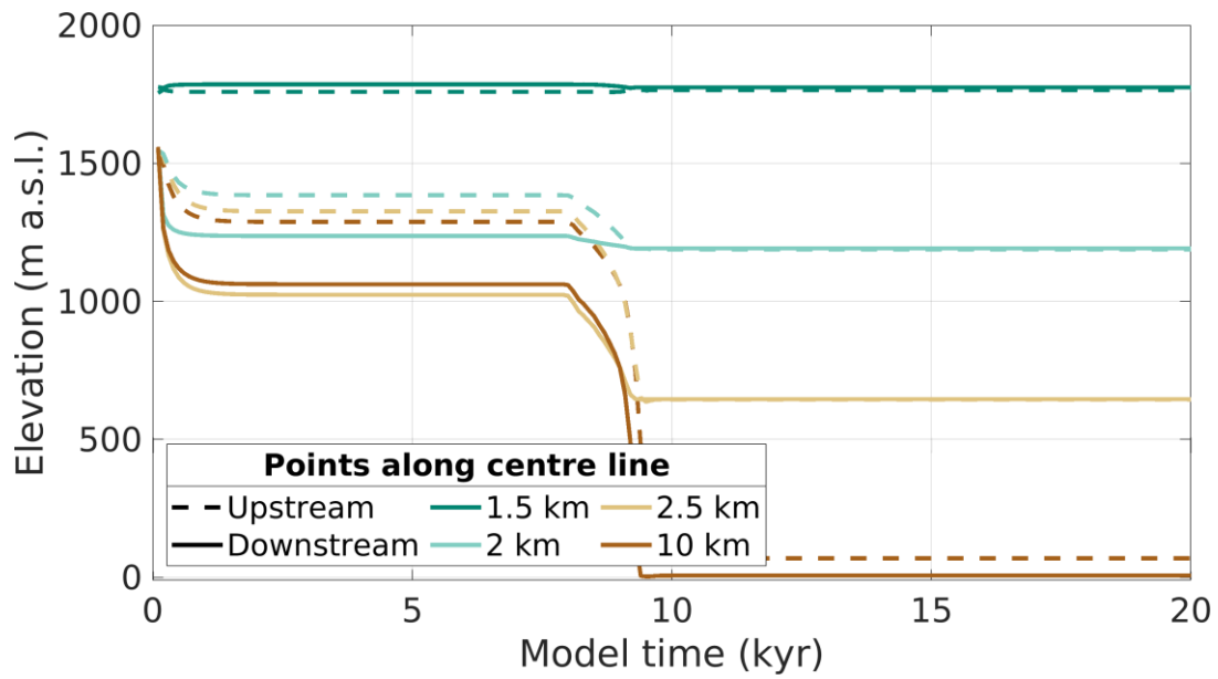
130 Figure S7. Surface evolution of select points equidistant (up and downstream) from the nunatak centre along the domain centre line, for an experiment on a retrograde bed slope (cf. Methods section in the main text).
