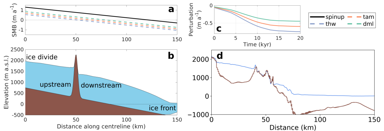
Figure 4. Model domain setup: (a) SMB ( \text{m a}^{-1} ) profiles for the spin up and initial state (black), and at the end of each different ice thinning experiment ('thw', Thwaites; 'tam', Transantarctic Mountains; 'dml', Dronning Maud Land); (b) ice surface elevation (m a.s.l.) after the 20 kyr spin up for the across-flow elongated nunatak; (c) applied transient perturbation (in \text{m a}^{-1} ) to each ice thinning experiment during the 20 kyr simulations subsequent to spin up; (d) Bedrock and ice sheet surface elevation profiles across an example nunatak in Antarctica (Half-way nunatak, [78.38 °S, 161.1 °E], upper Skelton Glacier, Transantarctic Mountains; see Fig. S1 for another 32 examples).
