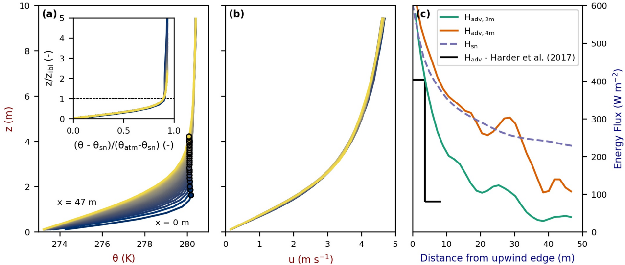
Figure 8. Time-averaged vertical temperature (a) and wind profiles (b), and horizontally advected sensible energy H_{adv} (at 2 and 4 meter integration height) and vertical sensible heat flux at the surface H_{sn} (c) along the snow patch at y = 83 \text{ m} and x = 150 \text{ m} in the P30m simulation. The markers in the temperature profile resemble the IBL height, which is computed as the first value (seen from the bottom) of the gradient of the temperature over height below 0.1 \text{ K m}^{-1} . The first 2 upwind grid cells and 2 downwind grid cells have been removed, as these are located in the transitions region from bare ground to snow and vice versa. The labels with 'x =' show the location of vertical profile related to the downwind distance of the leading edge, whereas the line colors are based on the distance from the leading edge and go from purple to red. In the inset graph, the vertical temperature profile has been normalised with height of the IBL and prescribed temperature of the surface and atmosphere. The advected energy as a function of distance from the leading edge are based on Equation 17.
