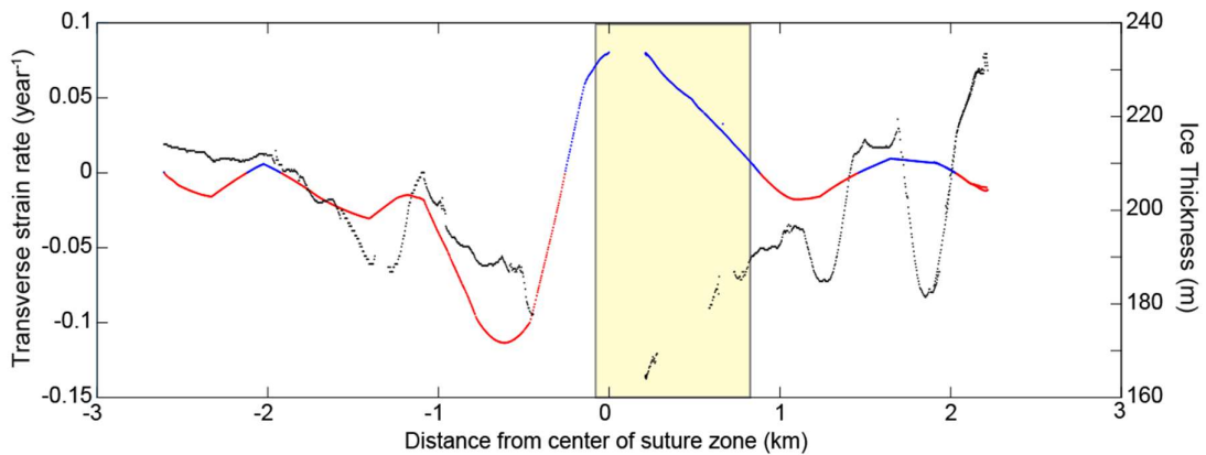
Figure 7: Site 2 transect ice thickness (black) with transverse strain rate (red: compression; blue: extension) interpolated along the transect. The location of the new surface fracture formed in 2016 is blocked in yellow and intersected this IPR transect. Note the radar drop out in the region of fracture formation.
