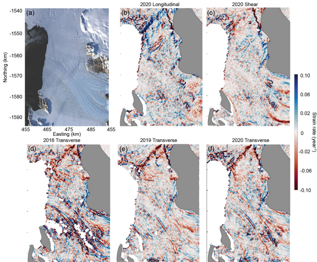
Figure C2: (a) The Nansen Ice Shelf (NIS) from Landsat-8 acquired March 22, 2017. (b) Longitudinal strain rate from GoLIVE velocity data acquired between October 10 and November 11 2020. (c) Shear strain rate from the same data as (b). (d) Transverse strain rate from GoLIVE velocity data acquired between September 29 and October 31 2016. (e) Transverse strain rate from GoLIVE velocity data acquired between October 8 and November 9 2019. (f) Transverse strain rate from the same data as (b).
