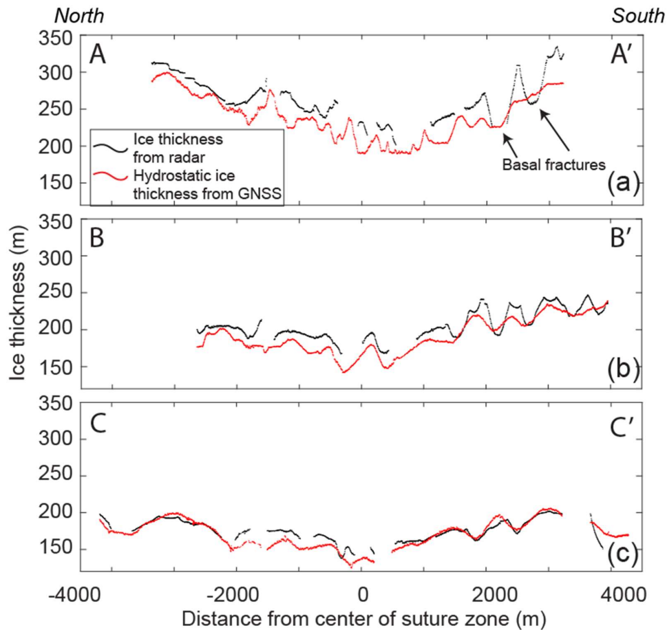
Figure 3: Cross-ice shelf transects of ice thickness from radar measurement (black) and from hydrostatic balance calculations using in situ GNSS surface elevations (red) at (a) Site 1, (b) Site 2 and (c) Site 3 on the NIS. The transects are marked on Fig. 2a.
