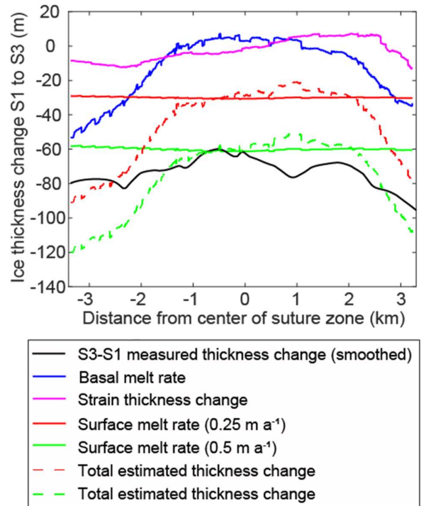
Figure 6: Cumulative ice thickness change between Site 1 and Site 3 calculated from IPR thickness change (black), Cryosat-2 basal melt data (blue), two surface melt rates (red and green), and strain thinning (pink). Total thinning (Cryosat-2 basal melt plus surface melt plus strain thinning) is shown by the dashed red and green lines for surface ablation rates of 0.25 and 0.5 m a -1 , respectively.
