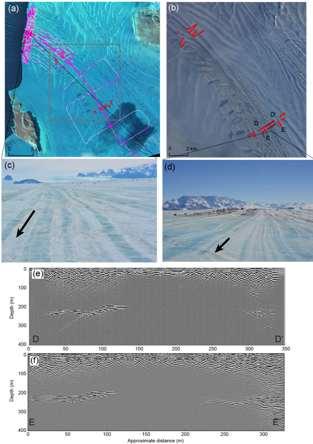
290 Figure 5: (a) Sentinel image of NIS from October 5 th 2016. Pink points are regions with radar signal dropout from the airborne radar and red points show signal dropout from the ground-based radar. The grey lines show the airborne radar and the grey box shows the extent of (b). (b) Larger-scale image showing ground-based radar dropouts in red. The black lines show the extent of the radar transects plotted in (e) and (f). Background image is Landsat 8 March 22, 2017. (c) and (d) Photos of surface striping on NIS showing filled crevasses associated with the marine ice drop-out regions taken on November 11 and November 18, 2016, respectively. (e) and (f) Radargrams with signal dropout. Transect locations are shown in (b).
