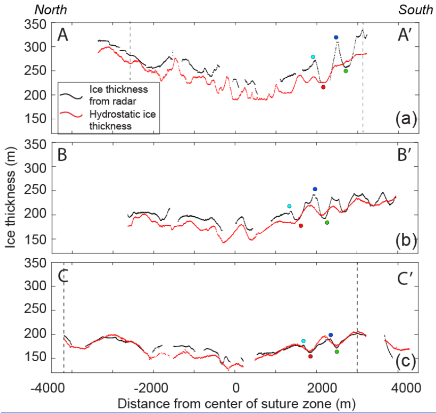
Figure 3: Cross-ice shelf transects of ice thickness from radar measurement (black) and from hydrostatic balance calculations using GPS the ice shelf surface elevations (red) at (a) Site 1, (b) Site 2 and (c) Site 3 on the Nansen Ice Shelf NIS . The colored dots represent where the basal draft apexes and keels were compared between sites. The dashed grey lines show the limits of the flux gate calculations. Transects are marked on Fig. 2a.
