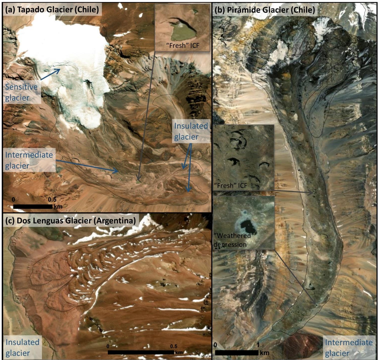
Figure 1: Three glaciers in the semiarid Andes for which the glacier-type (sensitive, semi-sensitive intermediate or insulated) is clearly identifiable based on the geomorphological criterion presented in this paper are shown. Tapado Glacier is made up of the three distinct glacier types proposed in this study. Approximately 95 % of surface of Pirámide Glacier is covered by debris and there are numerous thermokarst depression features, so it is classified as an an semi-sensitive intermediate glacier. Dos Lenguas glacier does not have ice exposed at the surface, has convex topography accentuated with ridges and furrows, and an obvious frontal slope so it is classified as an insulated glacier. Image source (Esri basemap): (a) 11 March 2019 GeoEye (0.46 m), (b) 18 January 2013 WorldView-2 (0.5 m), (c) 17 September 2017 WorldView-2 (0.5 m).
