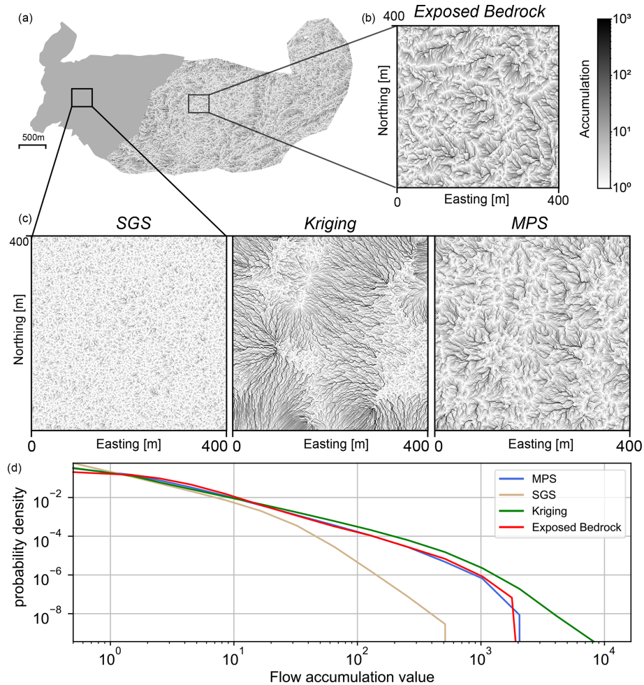
Figure 9. Flow accumulations calculated from the three methods and compared against the one computed in the exposed part of the bedrock used as reference and the probability density of accumulation values. The SGS simulation underestimates the length of the connected path, while kriging overestimates it. The visual patterns and the flow accumulation distribution obtained with MPS are the closest to the exposed bedrock reference.
