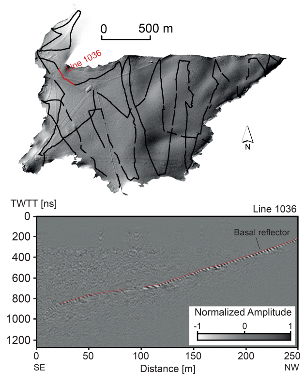
Figure 2. Acquisition lines from August 2018. The cumulative length is about 18 km. Hill shade from the DEM derived from drone images. The straight lines visible on the hill shade are ski lifts and transit tracks for snow groomers. A GPR line is displayed, with the basal reflector outlined.
