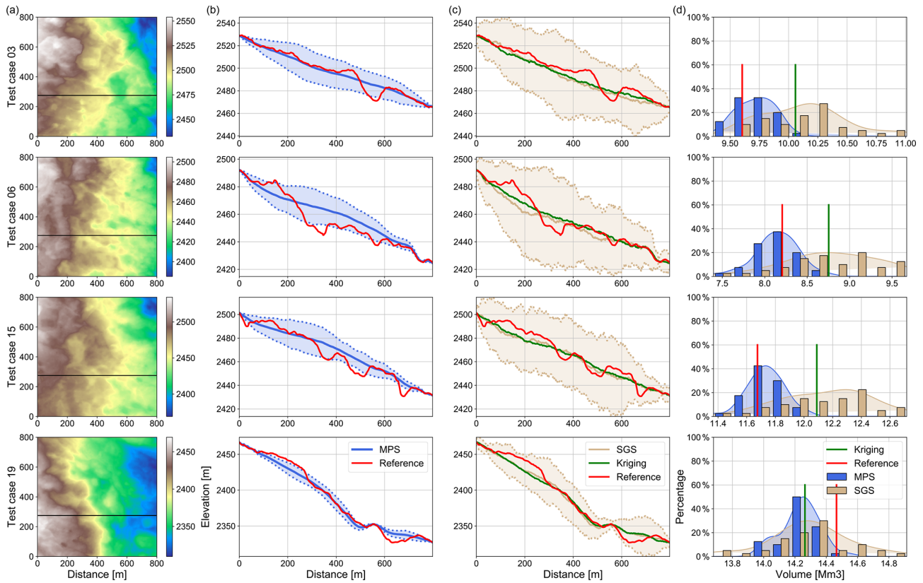
Figure 6. Synthetic test results. Panel (a) displays the reference DEM in a plan view, with the black line showing the location of the cross sections. Panel (b) presents the distribution of the cross section simulated with the MPS method (parameter set 3). Panel (c) presents the distribution of the cross section simulated with the SGS methods (parameter set 1). Panel (d) presents the different volume distribution of the methods against the reference one in red.
