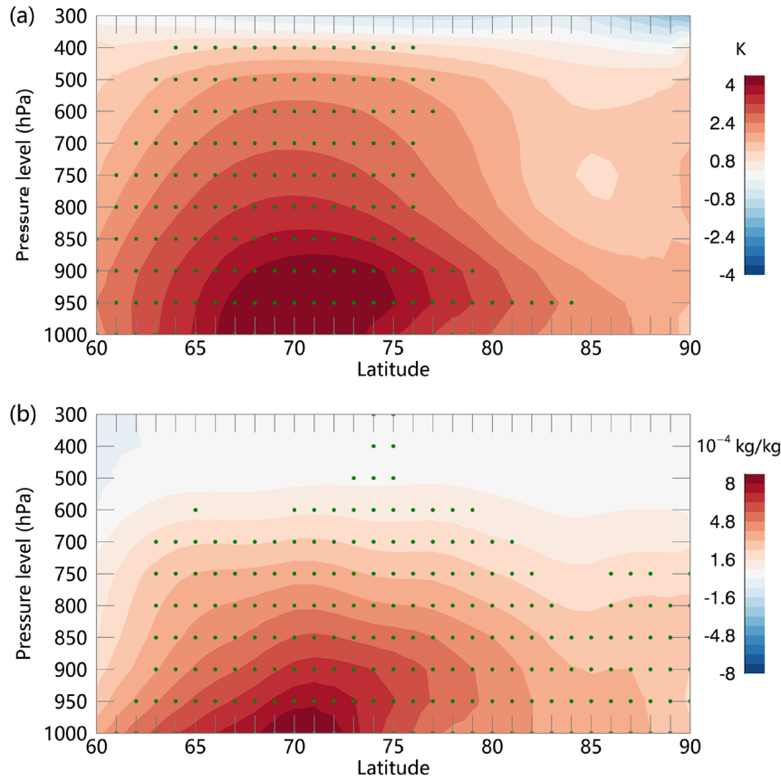
235 Figure 4. Vertical cross-sections of zonal averaged (a) air temperature and (b) specific humidity anomalies, as a function of latitude and pressure level, during the spring months (April–June) of 2020 spanning the regions with significant energy and moisture convergence (60° E-165° E, 60° N-90° N). The anomalies are calculated as the difference between the averaged fields of the three months (April–June) and the corresponding 1979-2020 climatology. Stipplings represent the values where the anomaly exceeds 2 standard deviations.
