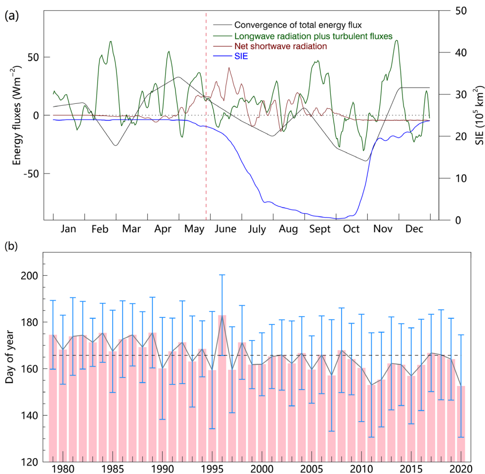
310 Figure 6. (a) Time series of SIE, the anomalies of atmospheric energy transport convergence and surface energy fluxes over the study area (indicated by the purple polygon in Fig. 1) during 2020. The blue curve represents the SIE. The red line denotes the anomalies of net solar radiation. The green line corresponds to the anomalies of the sum of the downwelling thermal radiation and the turbulent (latent plus sensible) flux. The vertical pink dashed line denotes the average date of ice surface melt (May 28) in 2020. The retrieved values are averaged over the oceanic grids by applying a land mask. The anomalies are relative to the 1979–2020 climatology of the years. (b) Melt onset date in each
