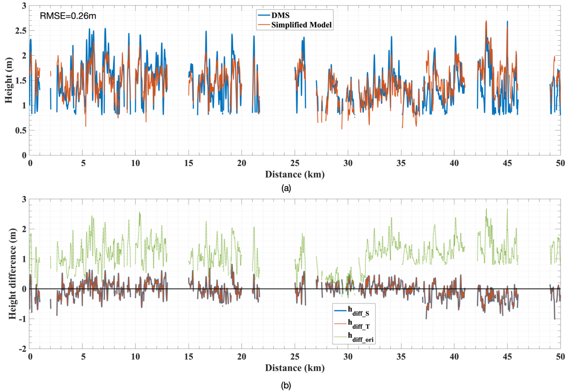
Figure 14. (a) Sea ice height profiles from DMS measurement (blue) and model inversion (red). Each profile represents the height along a 1 \times 5000 -pixel section at the center of the co-registered segment. (b) Height difference between the DMS measurement and the simplified model-derived height (blue), theoretical model-derived height (red), or original InSAR-derived height (green). The mis-coregistered and h_{\text{DMS}} below 0.8m samples are excluded from the plots. 0m is plotted in the black line as a reference.
