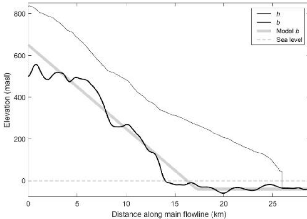
Figure 4. Cross-section along centerline profile (shown in Figure 3) of the main flowband, with band-averages of: surface topography (thin black line) from the 2009/2011 NPI DEM, bed topography from the Fürst et al (2018) reconstruction (0-12.5 km), 2015 helicopter radar measurements (12.5-25 km), and hydrographic data in the fjord (Norwegian Mapping Authority Hydrographic Service). A piecewise linear profile is fit to the bed profile for the MGM.
