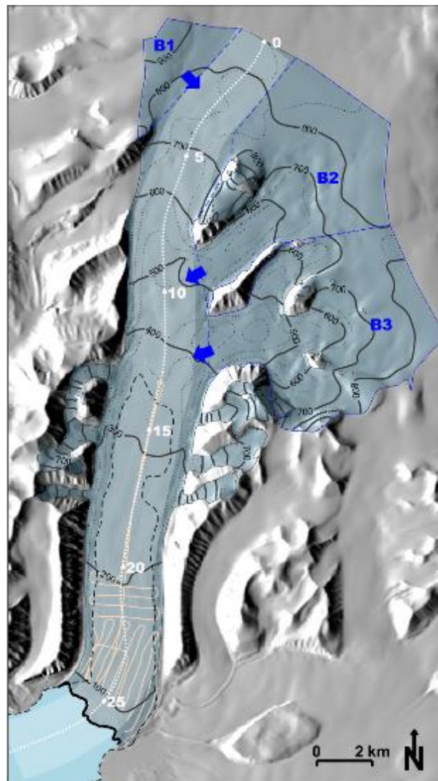
65 Figure 3. Map of Tunabreen. Surface contours (thick black lines) at 100-m intervals are from the NPI S0 DEM (Norwegian Polar Institute, 2014), based on aerial photography from 2009 (lower glacier tongue, 0-450 masl) and 2011 (upper glacier, > 450 masl). Bed contours (dotted black lines) at 100-m intervals are based on the Furst et al (2018) reconstruction in the upper glacier, and 2015 helicopter radar (K. Lindback & J. Kohler, in Welty et al 2020) measurements (light-red lines) in the lower glacier. Dashed subglacial contour shows the part of the bed below sea level. Center line profile (dotted white line) along 2200-m wide main flowband (lighter blue) shows distance from the ice divide at 5-km intervals. Three upper basins (blue dashed outlines) supply mass to the main flowband (blue arrows).
