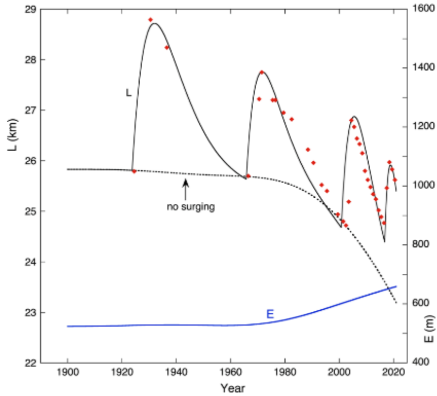
300 Figure 7. Simulation of glacier length L achieved after optimization of the model parameters. Observations are indicated by red dots. The blue line shows the optimal ELA forcing (scale at right). Glacier length simulated for a case without surging is shown by the dotted line.
