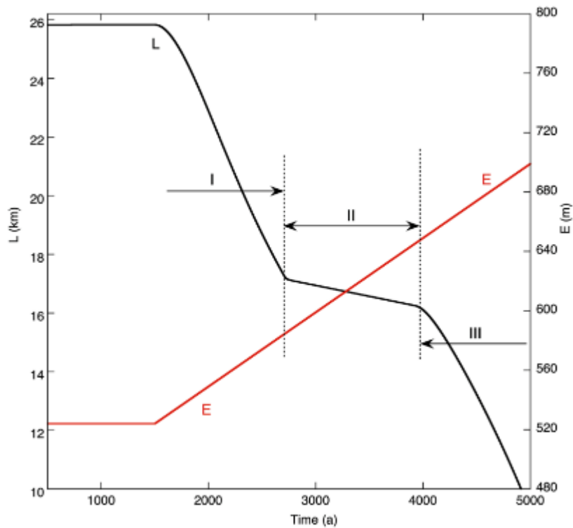
Figure 6. Glacier length L for a very slowly increasing ELA ( E ). Three regimes are identified (I, II, III) for which the sensitivity of glacier length to the ELA ( \partial L / \partial E ) differs significantly.
