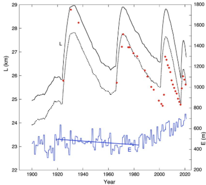
305 Figure 8. Simulation of glacier length L with ELA_{LYR} as climate forcing (scale at right). Observations are indicated by red dots. The simulation shown by the solid line is tuned to the first observed glacier length (1926), the dotted line is tuned to the last observed glacier length (2020).
