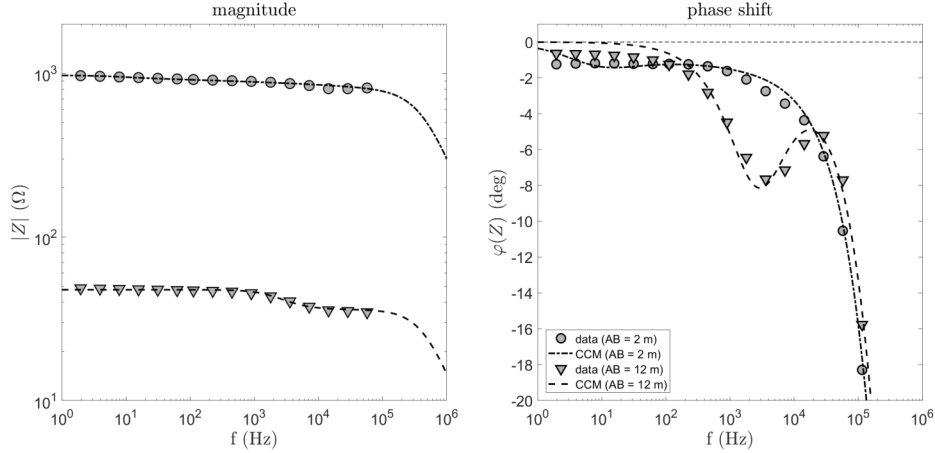
Figure 7. Spectra of the magnitude (left) and the phase shift (right) of the impedance Z for two measurements with electrode spacing \overline{AB} = 2 m (dots) and \overline{AB} = 12 m (triangles). The larger spacing, associated with higher investigation depth, shows a distinct frequency peak above 1 kHz, whereas the other spacing shows weaker frequency dependence. The symbols indicate the measured data, the dashed lines are the data calculated for the single Cole-Cole model, the parameters of which are provided in table 1.
