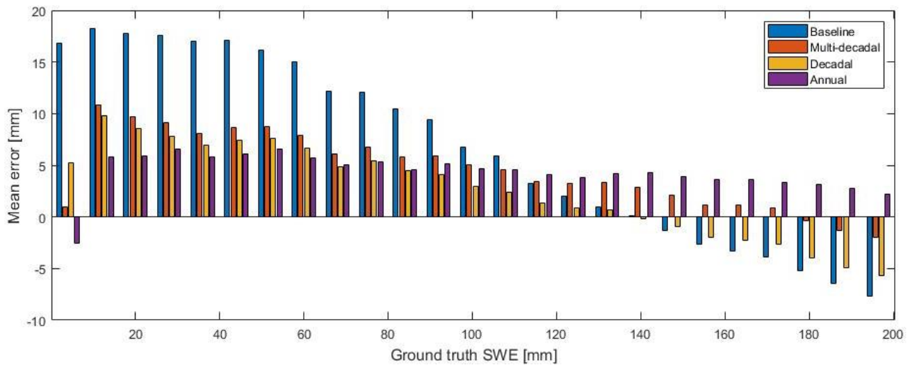
Figure 7. The mean error for the baseline, multi-decadal, decadal and annual SWE estimates, 2000-2009 Eurasia.
