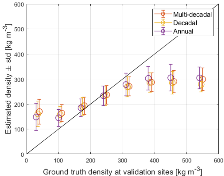
245 Figure 6. Comparison of multi-decadal, decadal and annual density estimates. As can be observed, annual densities perform best for small and large density values.
