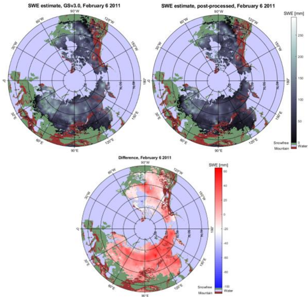
340 Figure 10. SWE maps for baseline GSv3.0 retrieval (top left), post-processed retrieval (top right) and difference between GSv3.0 and post-processed retrieval (post-processed subtracted from the baseline) for February 6, 2011. The post-processed SWE values are lower as overestimation of small SWE values is reduced.
