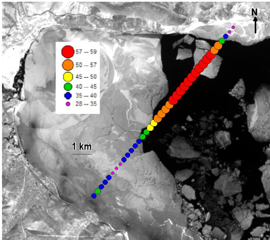
Figure 11. Backscatter values (dB) for the Jason-3 track 79, cycle 155 (26 April 2020, 20 h local time) overlaid over Landsat-8 image for 26 April 2020, 11h57 local time. Projection UTM 48N.
