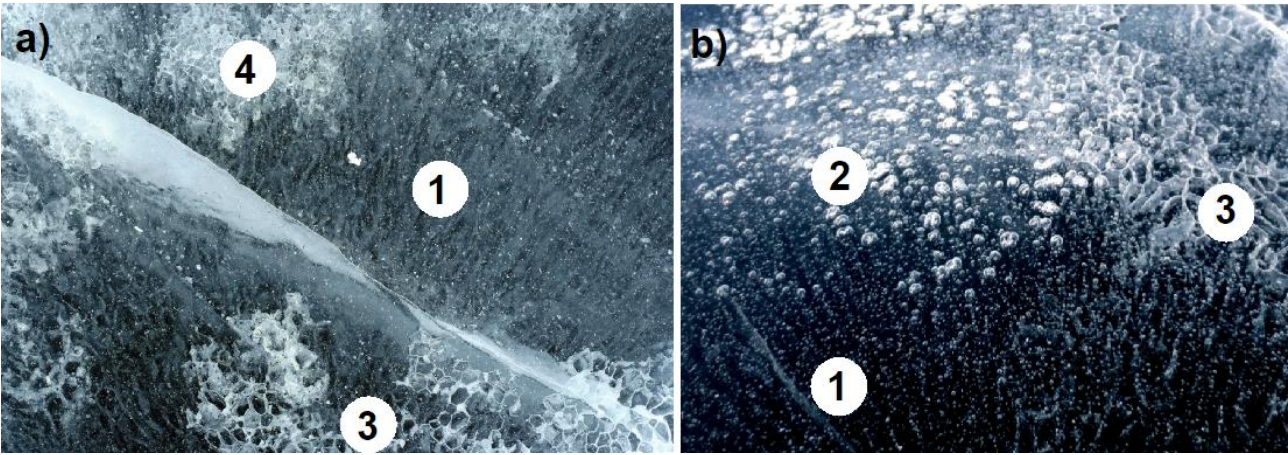
Figure 8. Different manifestations of ice metamorphism on the ice cover surface. a) Southern Baikal, 10 April 2006 (Photo: E. Petrov) b) Middle Baikal, 3 April 2014 (Photo A. Kouraev). Photo shots were taken while standing on ice (about 1.5 m height). 1 - vertical lines of air bubbles; 2 - large bubbles just below ice surface; 3 - air channels showing boundaries of columnar ice crystals; horizontal size of these crystals is about 2-4 cm; 4 - similar to 3, but upper central parts of columnar ice is also white.
