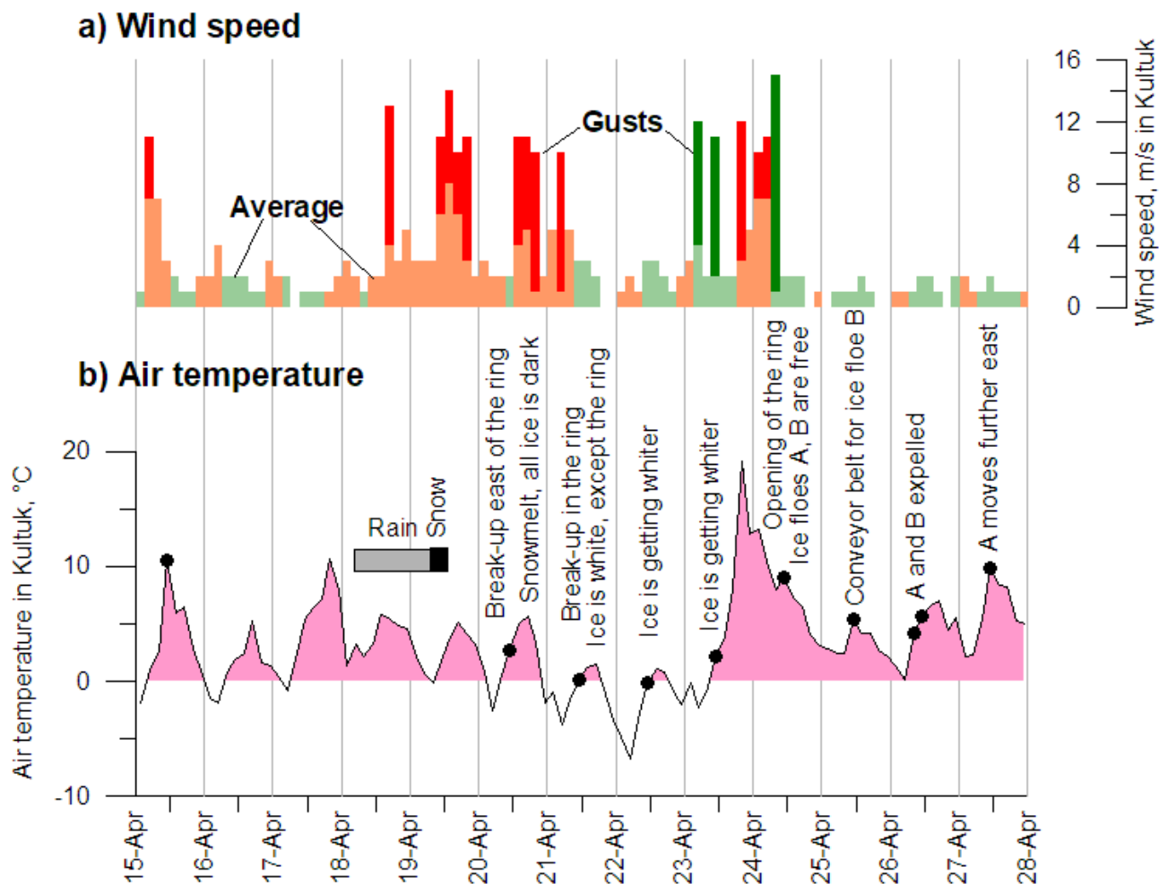
Figure 6. Temporal changes of a) wind and b) air temperature for 15-28 April 2020 at the Kultuk meteorological station (Russian Hydrometeorological Service). The period is selected to represent meteorological conditions for satellite imagery presented in the paper. Wind speed is coloured as a function of the general direction. Wind coming from the Tunka Valley (Kultuk wind) was classed as wind coming from the direction 292.5°(WNW, main direction of the opening of the valley) with a \pm 45^\circ span: 247.5 to 337.5°, or wind between WSW and NNW. Kultuk wind is coloured in peach/red, winds from all other directions – in light/dark green. For each of the two directions we also present two different estimates of wind speed: average wind speed (lighter colour), and maximal gusts (darker colour). Black circles on the air temperature graph – date and time of satellite images discussed in the text.
