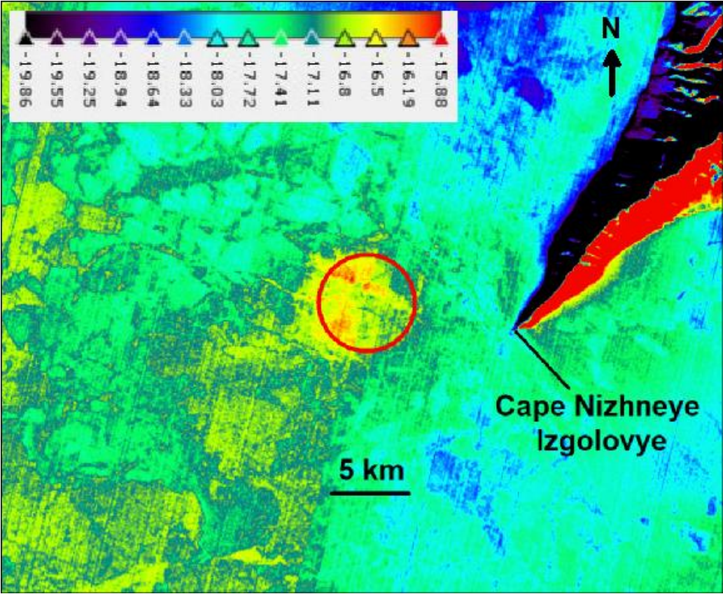
Figure 12. Ice and land surface temperature (°C) from Landsat 8 image on 6 March 2018. Red circle - position of outer eddy limit as defined from in situ data in February 2018. Projection UTM 48N.
