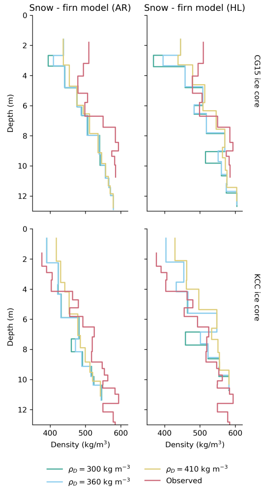
Figure 8. Observed and modelled (with multi-layer version) firn density profiles for KCC (bottom panels) and CG15 (top panels). AR and HL stand for the model version with Arnaud et al. (2000) and Herron and Langway (1980) implemented, respectively.
