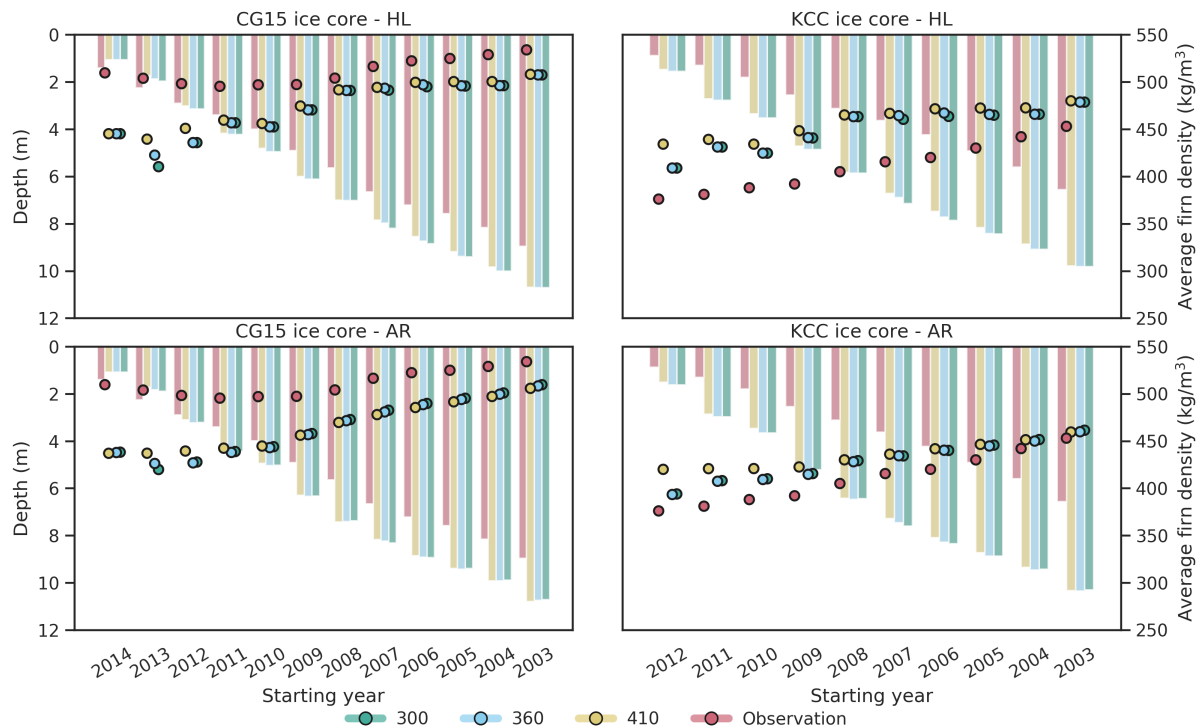
Figure 7. Observed and modelled (with one-layer version) average firn density for CG15 (left panel dots, right axis) and KCC depth (right panel bars, left axis) for KCC and CG15. The range Each cluster corresponds to a run of years in the x-axis indicates model whose starting date is reported on the deposition x-axis. Ending year of the layers whose density was averaged for all runs is 30 August 2013 for KCC and 30 September 2015 for CG15. AR and HL stand for the model version with Arnaud et al. (2000) and Herron and Langway (1980) implemented, respectively. The values 300, 360 and 410 stand for the chosen value of \rho_D .
